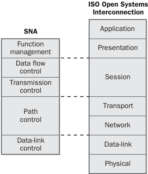
SNA. Comparable (not compatible) layers in the SNA and ISO/OSI architectures.
