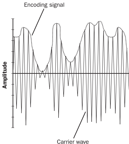
Amplitude modulation.
