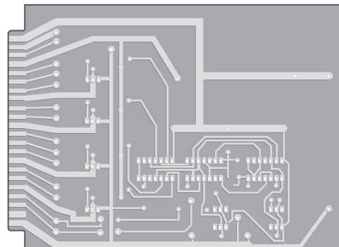
Printed circuit board.
