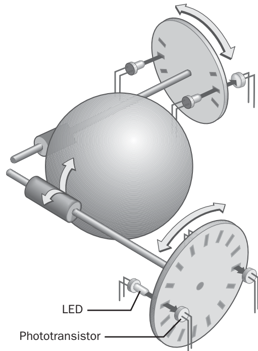
Optomechanical mouse.
