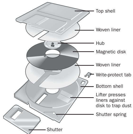
Exploded view.
