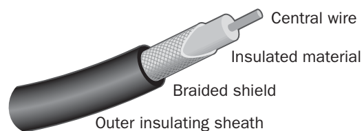
Coaxial cable.
