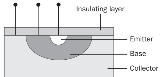
Planar transistor.
