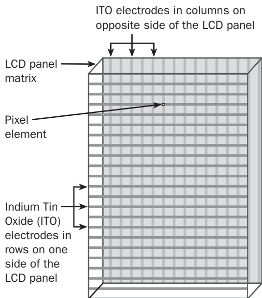
Passive-matrix display.
