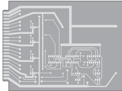
Circuit board.
