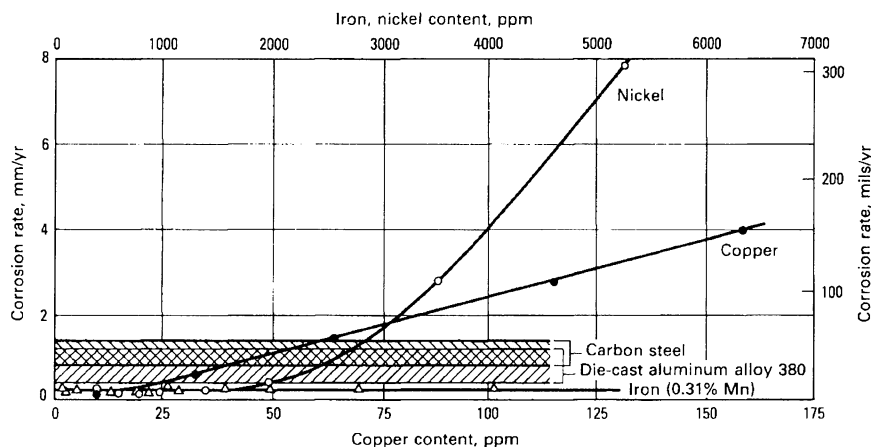
Fig. 5 Effect of nickel and copper contamination on the salt-spray corrosion performance of die-cast AZ91 alloy. Source: Ref 7
