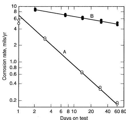
Fig. 2 Corrosion rates as a function of time for commercially pure magnesium. Curve A, distilled water vented to air through a caustic trap; curve B, distilled water vented to atmospheric \text{CO}_2 . Source: Ref 2
