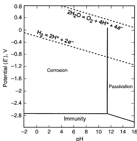
Fig. 1 Potential-pH (Pourbaix) diagram for the system of magnesium and water at 25 °C (77 °F), showing the theoretical domains of corrosion, immunity, and passivation. Source: Ref 1
