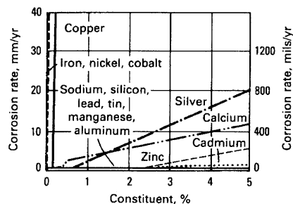
Fig. 4 Effect of alloying and contaminant metals on the corrosion rate of magnesium as determined by alternate immersion in 3% NaCl solution. Source: Ref 5
