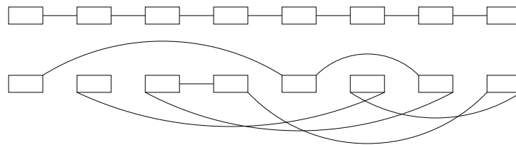
Figure 3.2 The list L before and after the call of permute .
