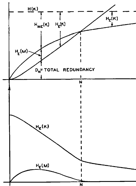
Fig. 8—Graphical calculation of equivocation.
