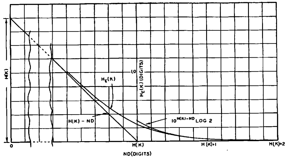
Fig. 7—Equivocation for random cipher.
