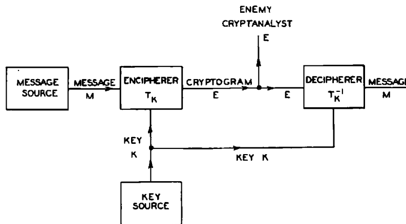
Fig. 1—Schematic of a general secrecy system.
