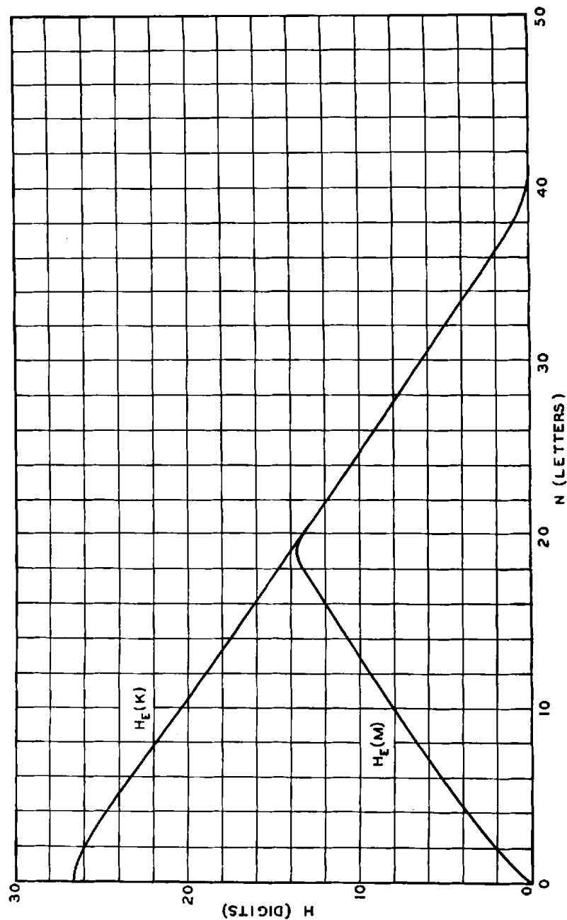
Fig. 10—Equivocation for Vigenère on English.
