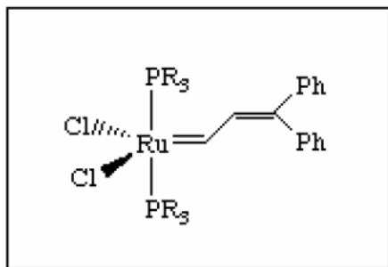
Figure 2.6: Ruthenium-based Grubb's catalyst for ROMP reactions
