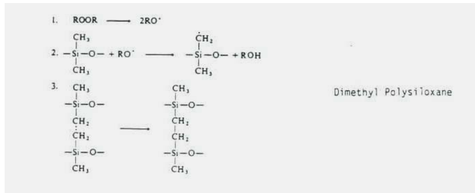
Figure 2.2: Peroxide-based mechanism for PDMS cross-linking
