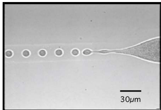
Figure 3.21: In-line Ebecryl 270 microfluidic device: n-hexane (8.0 psi)/dimethylformamide-1% p123 block copolymer (10.0 psi). Uniform droplet generation observed at tip of hexane stream in central cavity.
