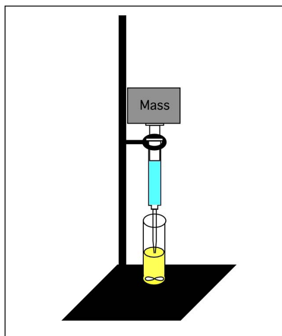
Figure 3.4: Experimental setup for capillary-based crossflow (w/o) emulsification experiment. A constant mass over the syringe provides a constant flow rate as water is introduced into the stirring continuous phase.
