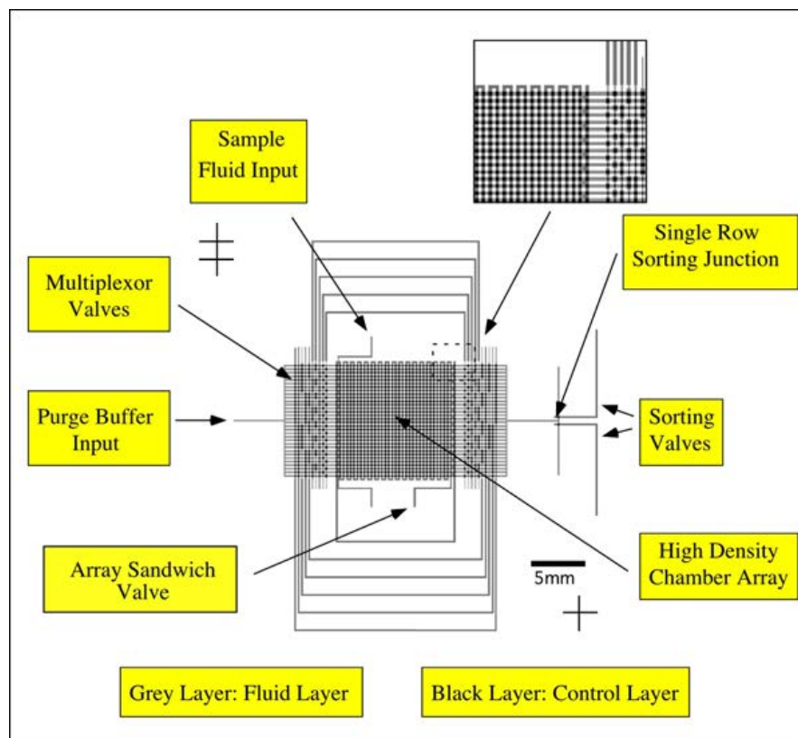
Figure 5.2: 1024 well serpentine chip schematic.
