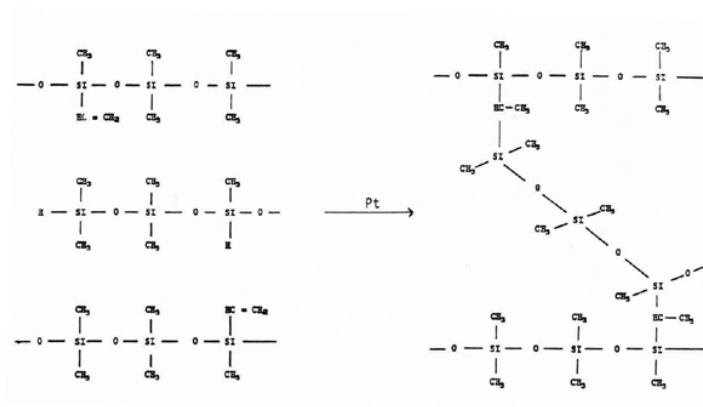
Figure 2.3: Platinum-based mechanism for PDMS cross-linking
