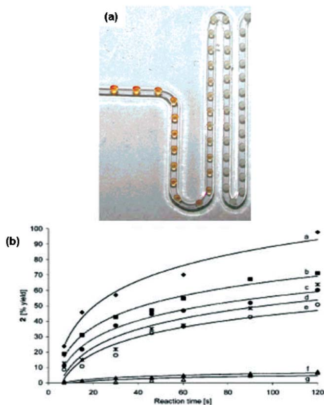
Fig. 12 (a) Bromination reaction performed in droplet microreactors. Change in color indicates completion of reaction. methods (reproduced with permission from ref. 47). (b) Comparison of hydrolysis reaction yields of p -nitrophenyl acetate under various conditions. Segmented flow (curves a–e) shows significant improvement in yield over bulk methods (curves f–g) (reproduced with permission from ref. 194).
