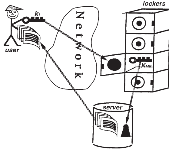
Figure 1: The Locker Key scheme
