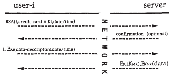
Figure 2: The Locker Key scheme: basic description
