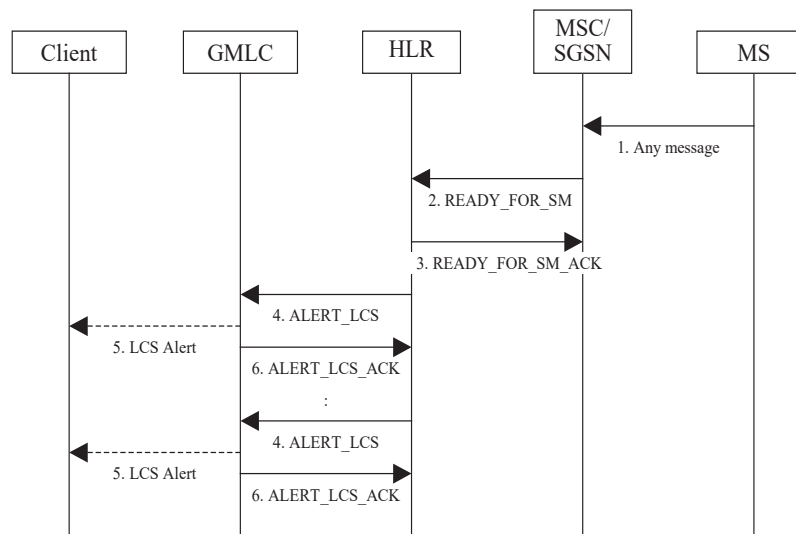
Figure 9.y: LCS Client Alerting procedure
