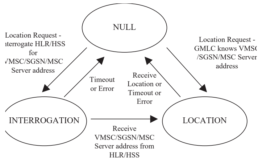
Figure 8.1: State Transitions in the GMLC
