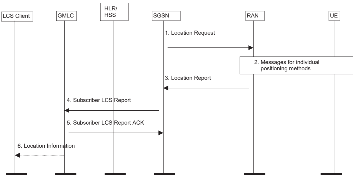
Figure 9.6: Network Induced Location Request
