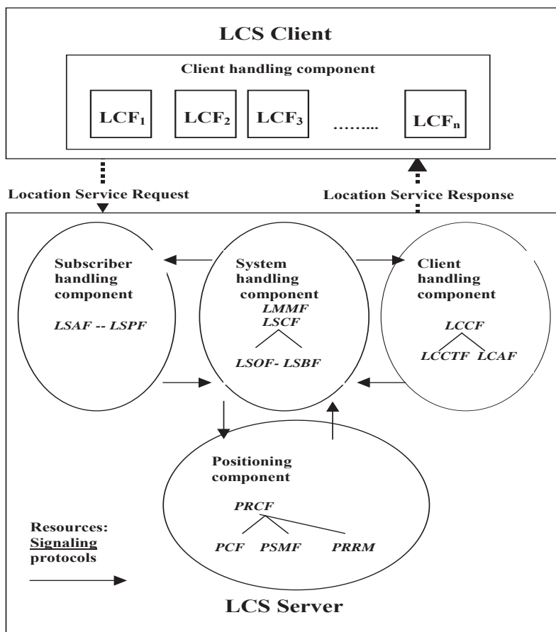
Figure 5.2: LCS capability server Functional Diagram
