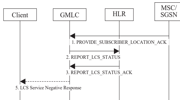
Figure 9.z: UE Presence Notification procedure
