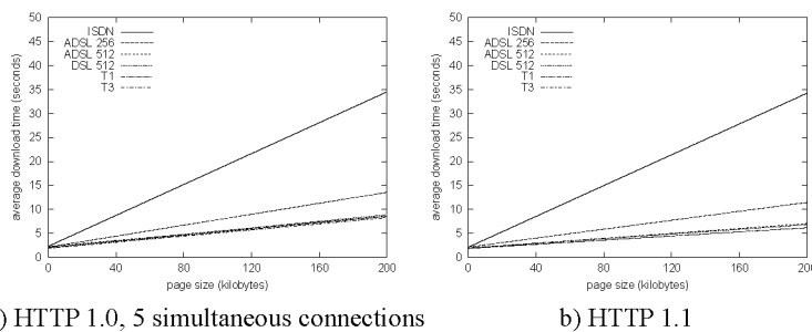
Figure 8.3: Download times with optimised tunnel throughput.
