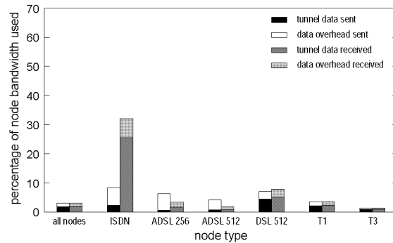
Figure 8.9: Bandwidth usage.
