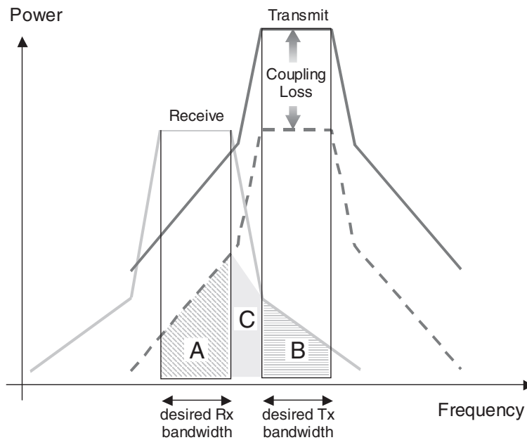
Figure 23.2: Frequency-domain interference between transmitter and receiver.
