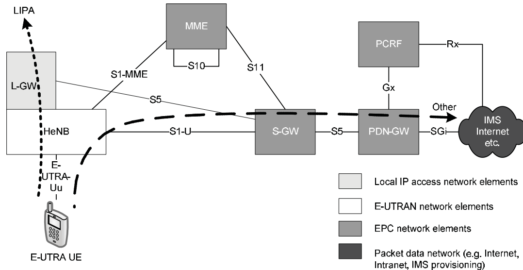
Figure 24.3: HeNB operating in LIPA mode in Release 10.
