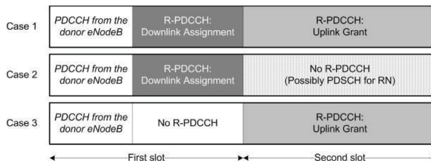
Figure 30.16: Supported R-PDCCH/PDSCH multiplexing possibilities.
