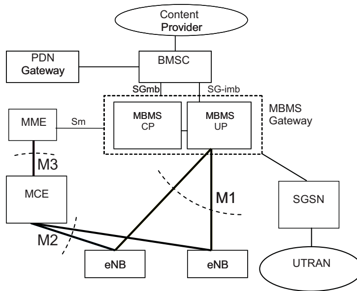
Figure 13.2: EPS reference architecture for MBMS broadcast mode [1].
