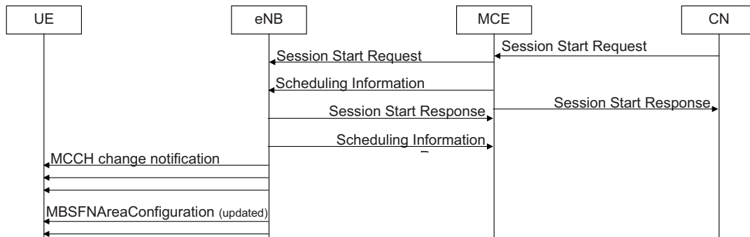
Figure 13.9: The MBMS session start message sequence.
