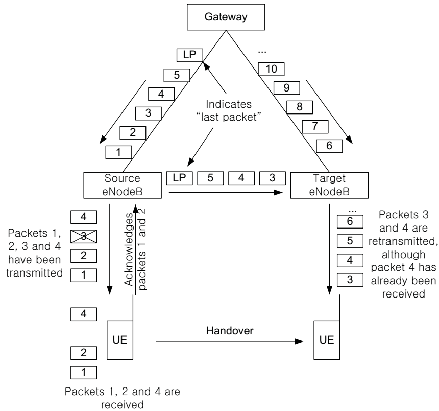
Figure 4.5: Lossless handover in the downlink.
