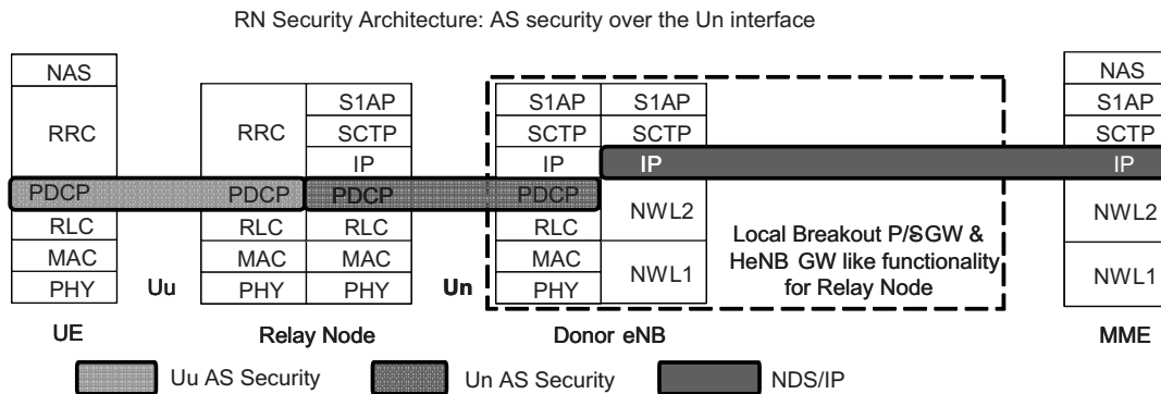
Figure 30.13: RN security architecture. Reproduced by permission of © 3GPP.
