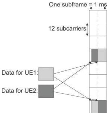
Figure 9.3: Frequency-distributed data mapping in LTE downlink.
