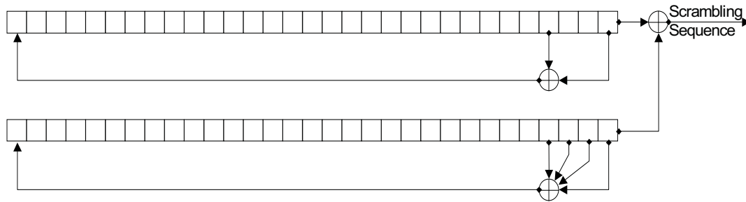
Figure 6.4: Shift-register implementation of scrambling sequence generator.
