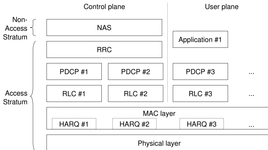
Figure 4.1: Overview of user-plane architecture.
