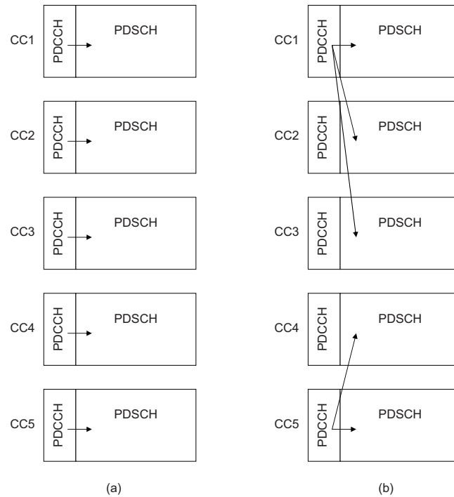
Figure 28.6: Examples of semi-statically configured mappings from PDCCH scheduling messages to CCs for data transmission:
