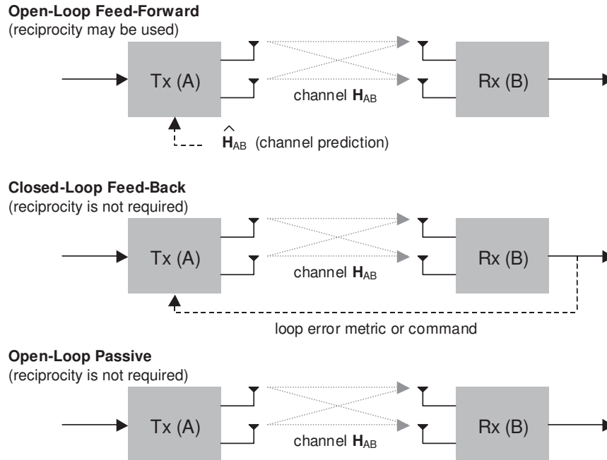
Figure 23.17: Feed-forward, feed-back and open-loop exploitation of the radio channel.
