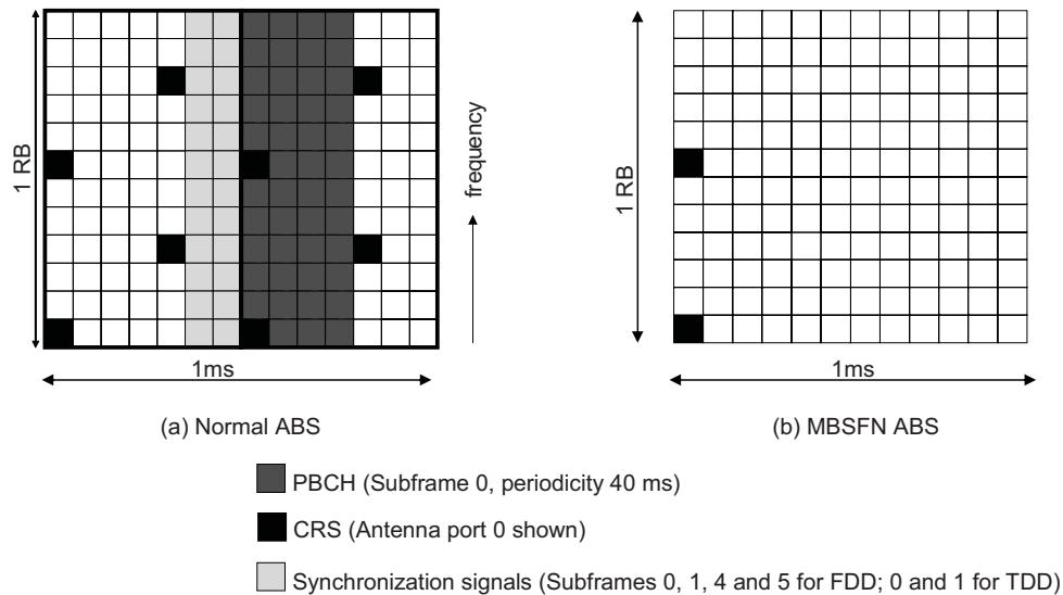
Figure 31.3: Normal and MBSFN Almost Blank Subframes.
