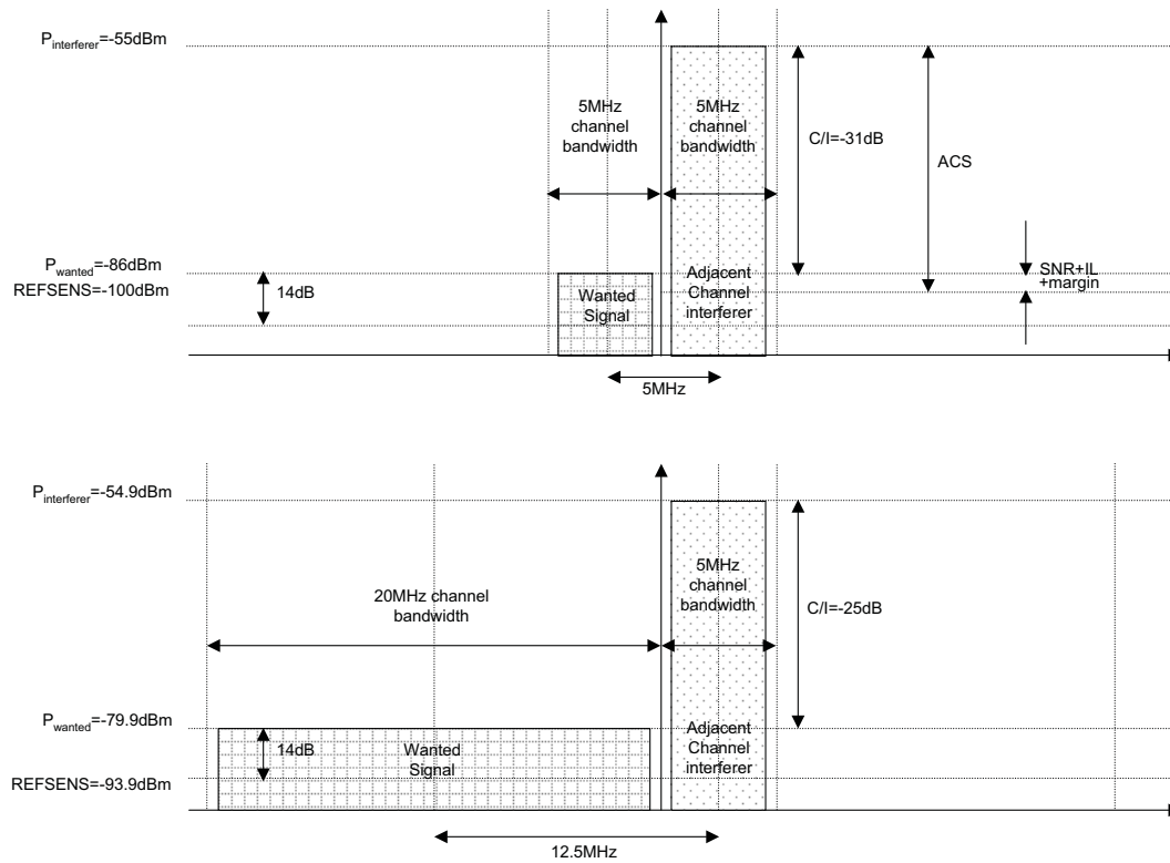
Figure 21.16: Adjacent channel selectivity illustrated for Case 1 [5].
