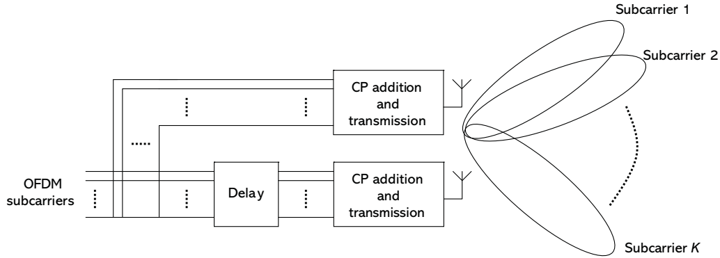
Figure 11.7: Principle of Cyclic Delay Diversity.
