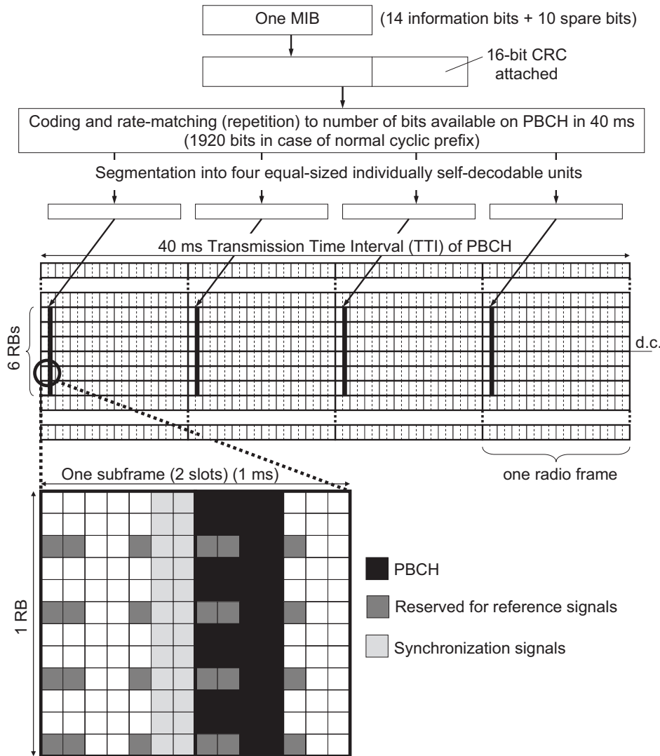
Figure 9.1: PBCH structure.
