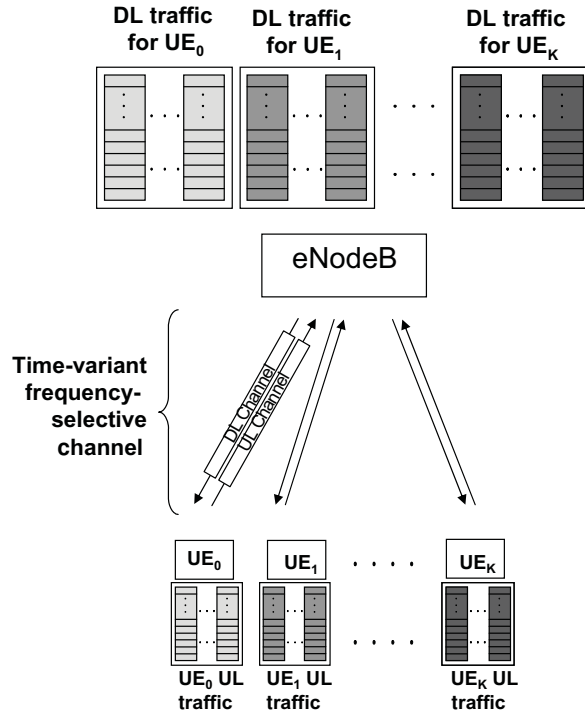
Figure 12.1: A typical single-cell cellular radio system.
