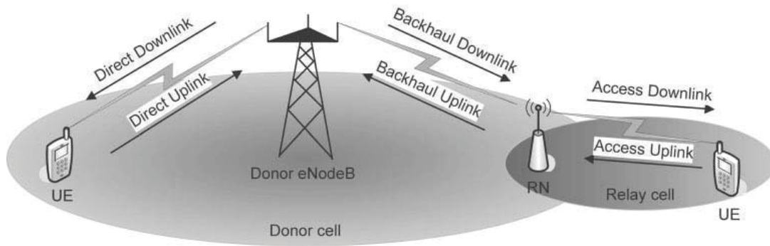
Figure 30.2: Terminology for relaying.
