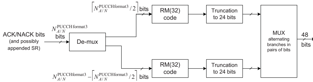
Figure 28.10: Coding and scrambling for PUCCH format 3.
