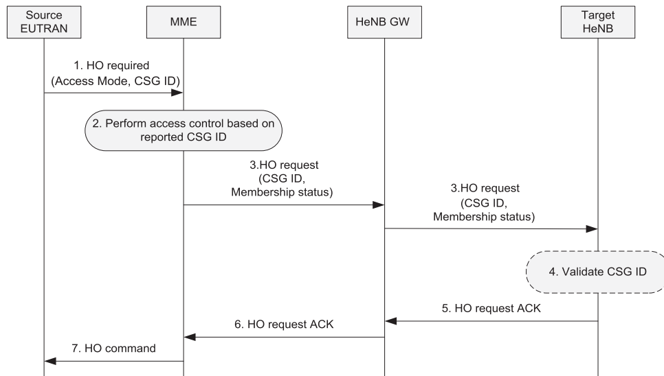
Figure 24.2: A typical call flow for mobility towards a HeNB.
