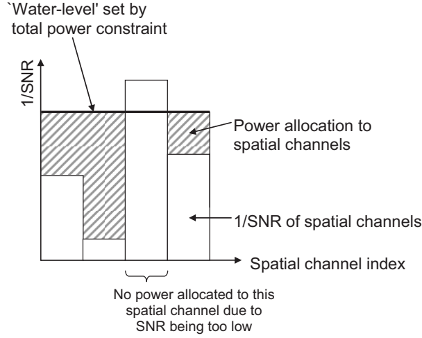
Figure 11.3: The waterfilling principle for optimal power allocation.
