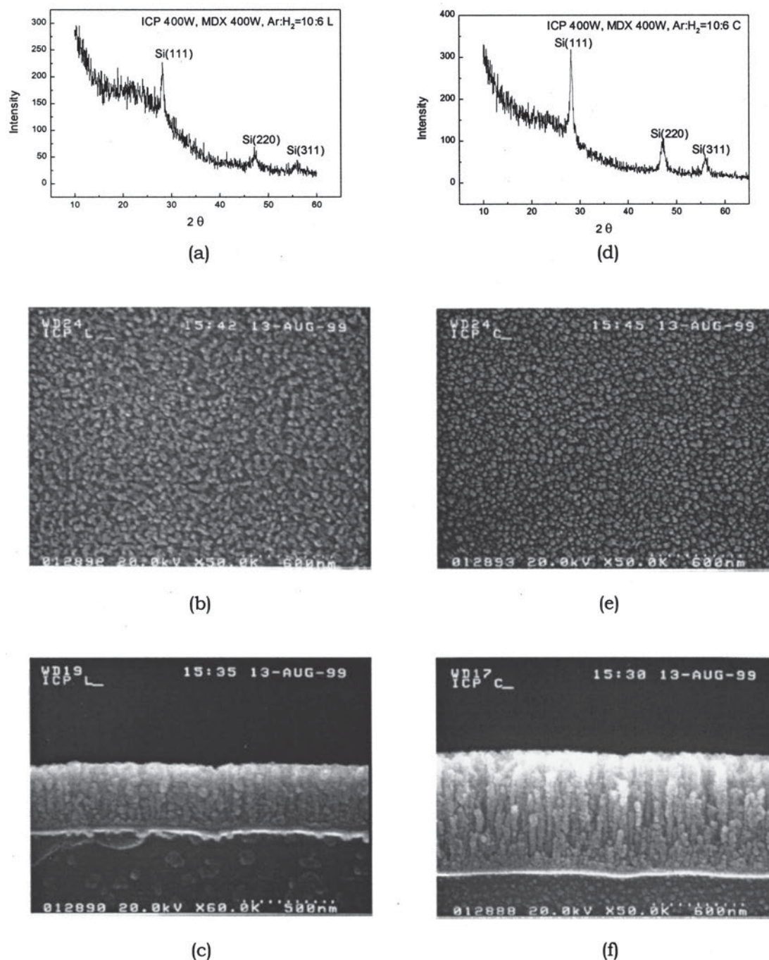
FIG. 4. X-ray diffraction analysis and SEM micrograph show that films have good structural property and grain size from 300 to 700 Å. (a), (b), and (c) are deposited in high- \text{Ar}^+ bombardment condition, and (d), (e), and (f) are deposited in low \text{Ar}^+ bombardment condition.
