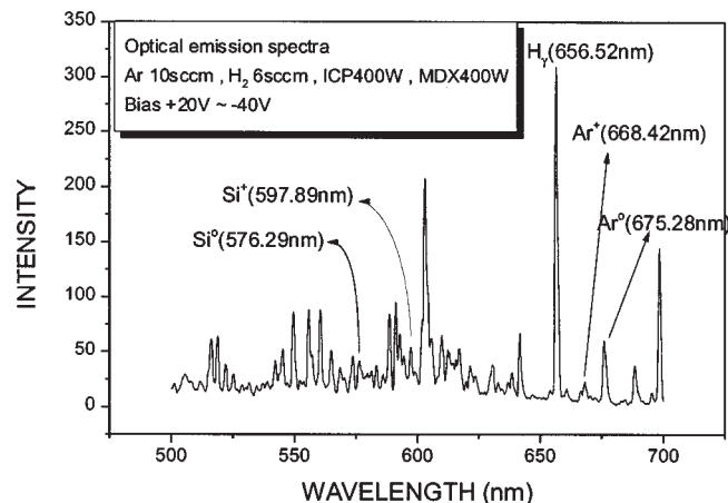
FIG. 7. Optical emission spectra show sputtered Si atom is ionized and hydrogen atoms are present in the ICP volume.
