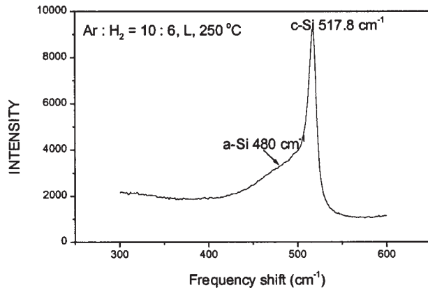
FIG. 6. Extended scan of Raman spectroscopy. Crystalline peak is shifted from 520 to 517.8 \text{cm}^{-1} and also contains amorphous Si contribution around low-frequency shoulder.
