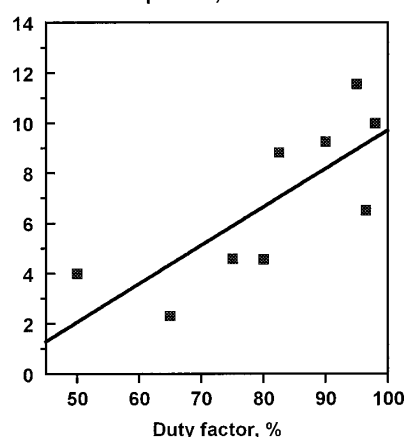
FIG 6 Relationship between the duty factor and normalized deposition rate for reactive pulsed sputtered alumina films
