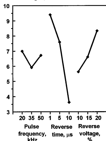
FIG 5 Taguchi analysis of alumina films, using the normalized deposition rate as the response variable
