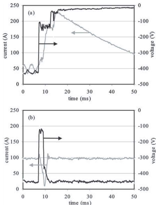
Figure 6. Electrical I-V behavior of an existing (a) and the new in-house developed (b) DC power supply on a bipolar arc (no additional arc suppressing electronics used).
