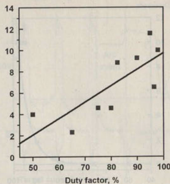
FIG. 6. Relationship between the duty factor and normalized deposition rate for reactive pulsed sputtered alumina films.
