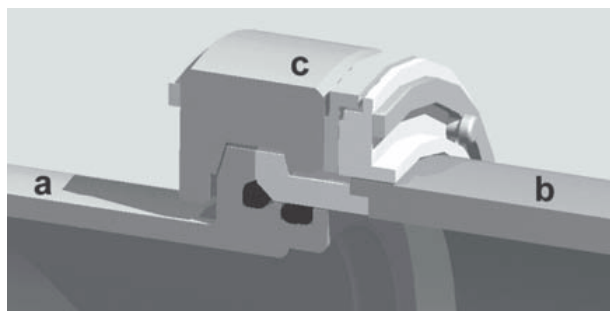
Figure 5. Schematic representation of the anti-arcing guard ring for rotating cylindrical target: (a) magnetron spindle, (b) cylindrical target tube, (c) target clamping with dielectric ring for arc prevention.
