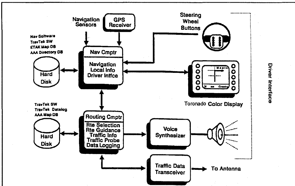
Figure 27. TravTek vehicle architecture. (2)
