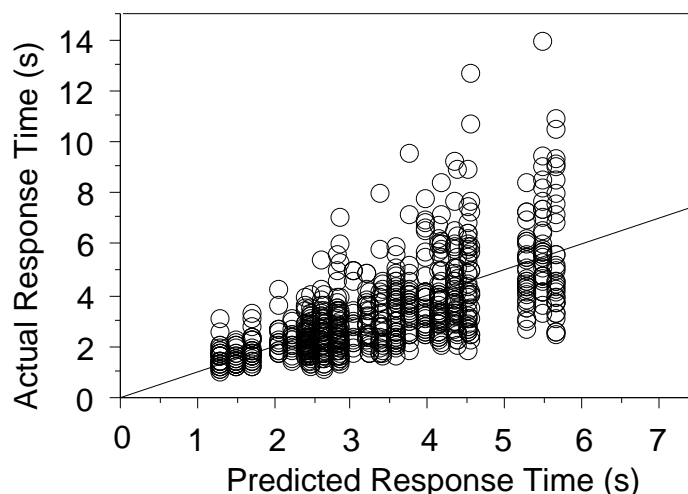
Figure 23. Task 2: Predicted response time vs. actual response time.
