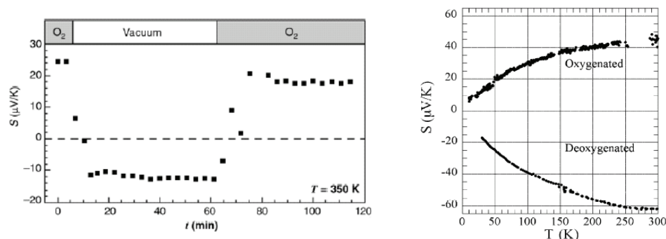
FIGURE 5 (a) TEP ( S ) versus time data for a SWNT film cycled between vacuum ( S < 0 ) and O_2 saturation ( S > 0 ). 17 (b) The T dependent TEP data for a SWNT film that has been O_2 saturated and then deoxygenated. 18
