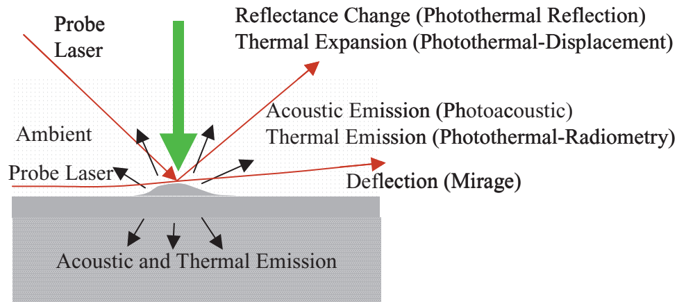
FIGURE 9 Variation of the sample temperature under time varying heating conditions generates different signatures that can be detected and used for obtaining the thermal diffusivity/effusivity of the samples. Examples of these signatures, as shown, are the thermal emission, refractive index change in both the sample and the surrounding media, and the thermal expansion in both the solids and the surrounding media.
