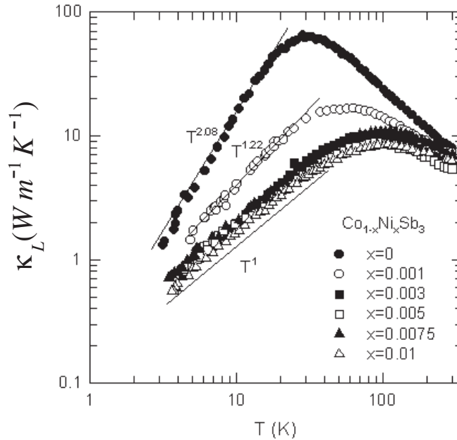
FIGURE 9. Temperature dependence of the lattice thermal conductivity of \text{Co}_{1-x}\text{Ni}_x\text{Sb}_3 between 2 K and 300 K. The lines indicate \kappa_L \propto T^{2.08} , T^{1.22} , and T^1 between 2 K and 30 K for x = 0, 0.001 , and 0.003 , respectively. 38 (Reprinted from Ref. 38. Copyright 2002, American Physical Society.)
