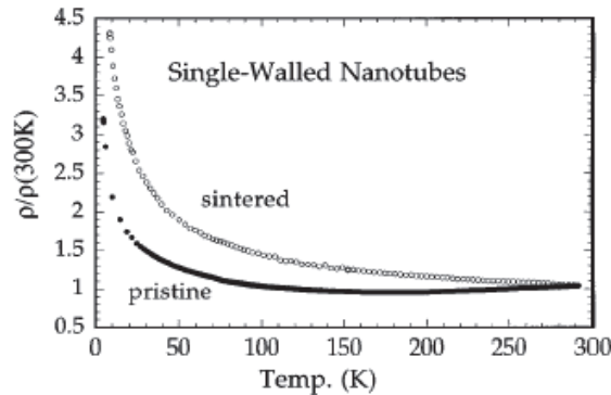
FIGURE 2 Normalized \rho(T) data to room temperature value for pristine and sintered SWNT films. 11
