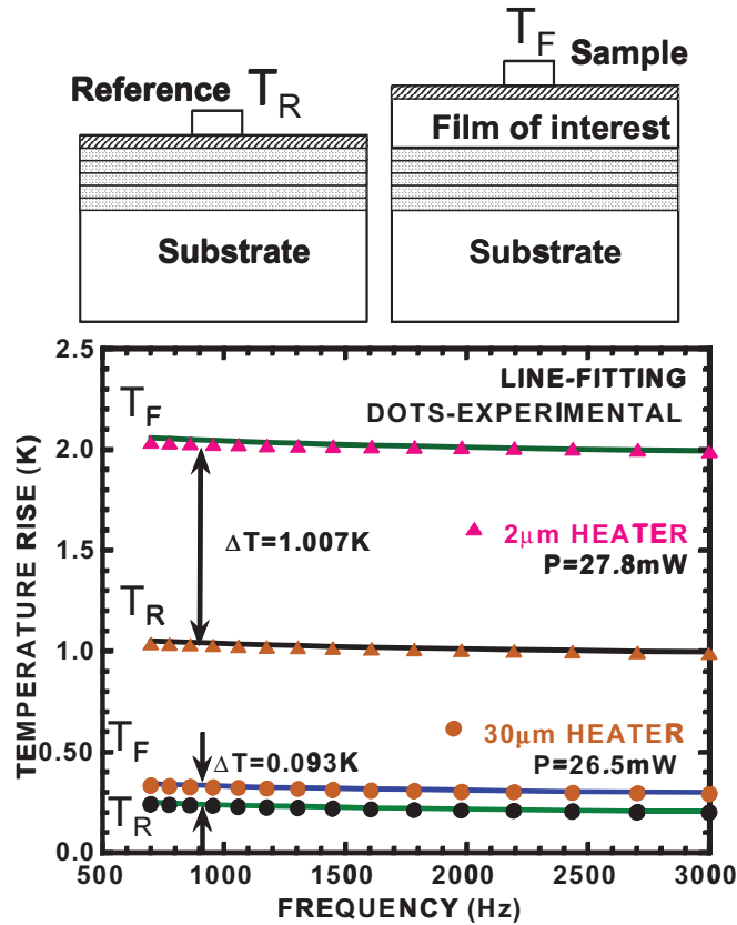
FIGURE 4. Example of an experimentally determined temperature drop across a Ge quantum dot super lattice film using a differential 3\omega method. In this method similar heaters are deposited on the sample and a reference without the film of interest. The temperature drop across the film is given by the difference in the temperature rise of similar heaters under similar power dissipation conditions. If the experiment is performed using a pair of large width or narrow width heaters, the anisotropic properties of the film may be determined. The solid lines are calculated by using Eq. (9) and the fitted thermophysical properties of the sample.
