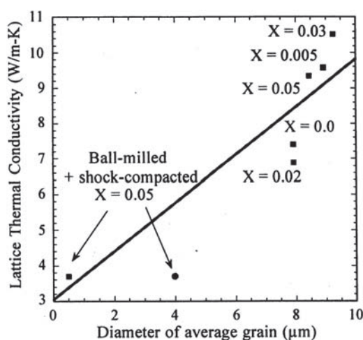
FIGURE 22. Lattice thermal conductivity versus average grain diameter of \text{TiNiSn}_{1-x}\text{Sb}_x including ball milled and shock compacted \text{TiNiSn}_{0.95}\text{Sb}_{0.05} . The line is a linear fit to the data. 73 (Reprinted from Ref. 73. Copyright 1999, American Institute of Physics.)
