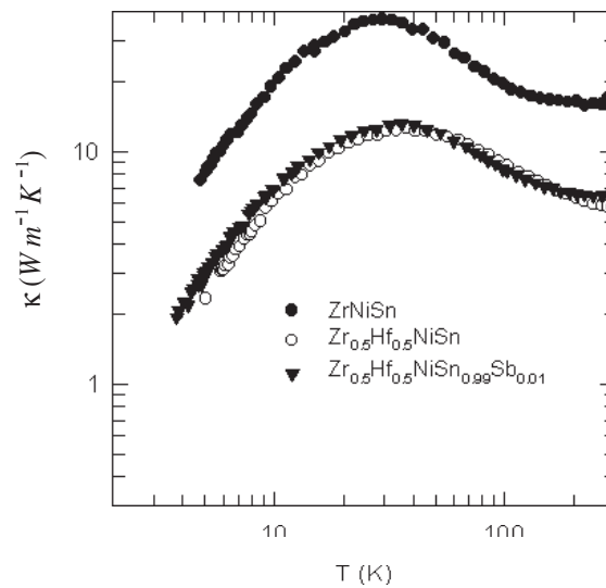
FIGURE 20. Thermal conductivity as a function of temperature for one week annealed ZrNiSn, \text{Zr}_{0.5}\text{Hf}_{0.5}\text{NiSn} , and \text{Zr}_{0.5}\text{Hf}_{0.5}\text{NiSn}_{0.99}\text{Sb}_{0.01} . 65 (Reprinted from Ref. 65. Copyright 1999, American Physical Society.)
