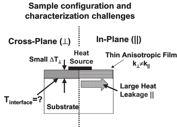
FIGURE 1 Typical sample configuration and challenges raised by the thermal conductivity characterization of thin films. Because the film typically has anisotropic thermal properties, measurements must be carried out in both the cross plane and in plane directions. For the cross plane direction the difficulties consist of creating a reasonable temperature drop across the film without creating a large temperature rise in the substrate and experimentally determining the temperature drop across the film. The in plane thermal conductivity measurement is affected by heat leakage through the substrate, which makes it difficult to determine the actual heat flow in the plane of the film.
