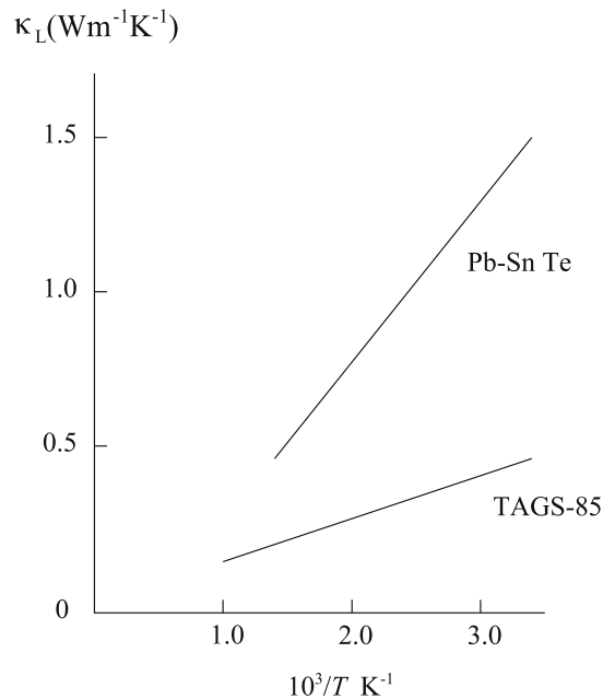
FIGURE 5. Plots of lattice conductivity against the reciprocal of the temperature for \text{PbTe} , \text{SnTe} and TAGS 85. 18
