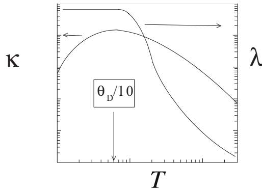
FIGURE 1 Schematic view of the thermal conductivity, \kappa , and the phonon mean free path, \lambda , as functions of temperature for a simple, insulating solid. Note that the peak in \kappa occurs at a temperature about 10% of the Debye characteristic temperature, \theta_D .
