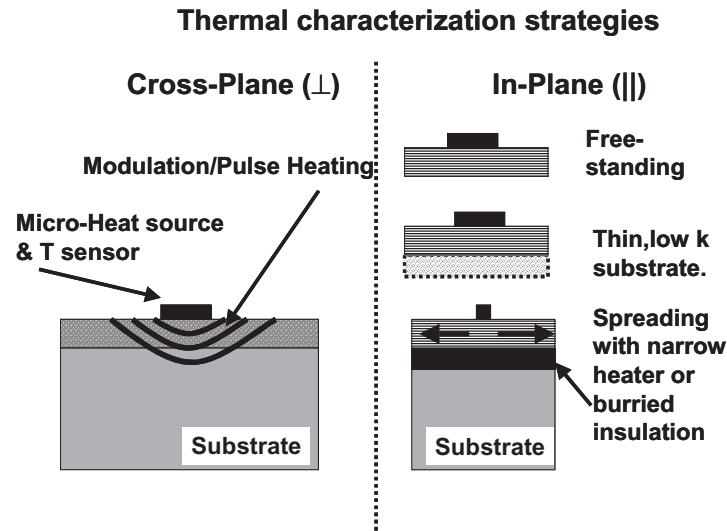
FIGURE 2 Strategies developed to measure the thin film thermal conductivity, or thermal diffusivity, in different directions. In the cross plane direction, the general strategies are creating a large heat flux through the film while minimizing the heat flux in the substrate and measuring the surface temperature rather than the temperature drop. For the in plane direction, often used strategies are to remove the substrate such that the heat flux through the film can be uniquely determined or to deposit the films on thin, low thermal conductivity substrates, which minimizes heat leakages. Other methods take advantage of the lateral heat spreading that surrounds small heat sources.
