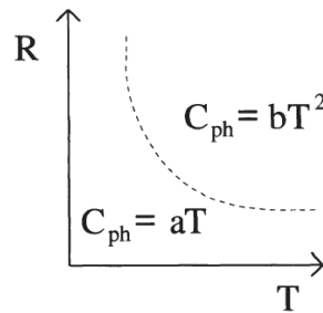
FIGURE 15 Schematic demonstrating the relationship between the radius ( R ), T , and C_{ph} in SWNTs. 31 For sufficiently small R and T ; C_{ph} scales as T ; otherwise it scales as T^2 .
