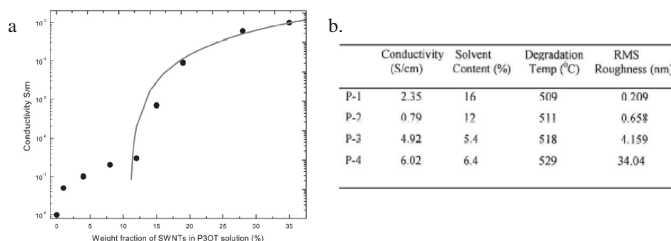
FIGURE 22 Enhancements in \sigma seen in many nanotube/polymer composites is evidenced by \sigma data in films of both (a) P3OT and SWNTs 45 and (b) PANI and MWNTs. 46
