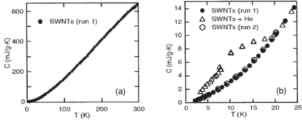
FIGURE 16 The T dependence of C_P per unit mass for SWNT bundles. 32 (a) The cooling data from room temperature to 2 K and (b) the low T data showing the effects of He exposure on C_P .
