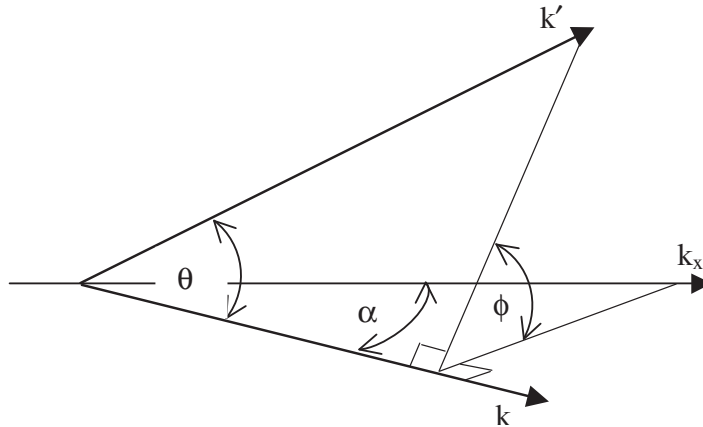
FIGURE 2 Scattering configuration in three dimensions. The electric field is assumed to be in the x direction. Magnitudes of both initial and final electron wave vectors are k_F . A current change results from changes in the electron velocity with respect to the direction of the electric field. Assuming free electrons, the direction of the electron velocity coincides with the direction of its wave vector. Consequently, after averaging over \phi , the change in the current is given by (k_x - k'_x)/k_x = 1 - v'_x/v_x = (1 \cos \theta) .
