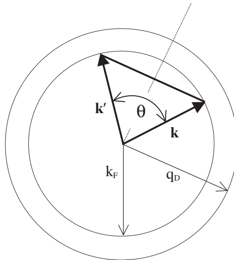
FIGURE 4 Relationship between the Fermi and Debye spheres for free electrons: q_D = 2^{1/3} k_F \cong 1.26 k_F . The maximum scattering angle \theta_{\max} is given by \theta_{\max} = 2 \sin^{-1}(q_D/2k_F) \cong 78^\circ .
