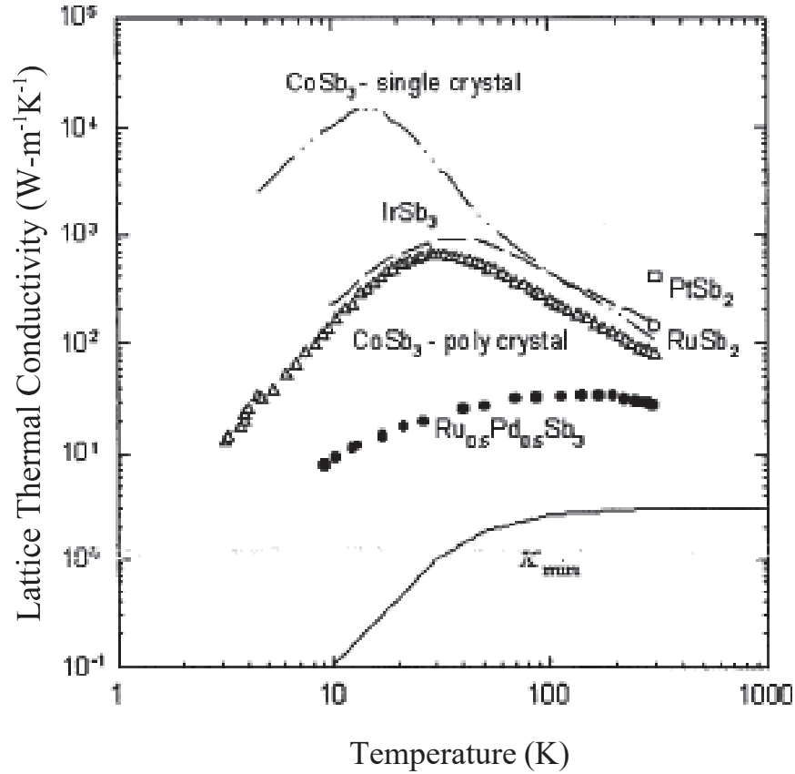
FIGURE 7. Lattice thermal conductivity versus temperature for single crystal \text{CoSb}_3 , polycrystalline \text{CoSb}_3 , polycrystalline \text{IrSb}_3 , and polycrystalline \text{Ru}_{0.5}\text{Pd}_{0.5}\text{Sb}_3 . 36 Also included are the room temperature data for \text{PtSb}_2 and \text{RuSb}_2 , and the calculated minimum thermal conductivity \kappa_{\min} for \text{IrSb}_3 . 36,38 (Reprinted from Ref. 36. Copyright 1996, American Institute of Physics.)
