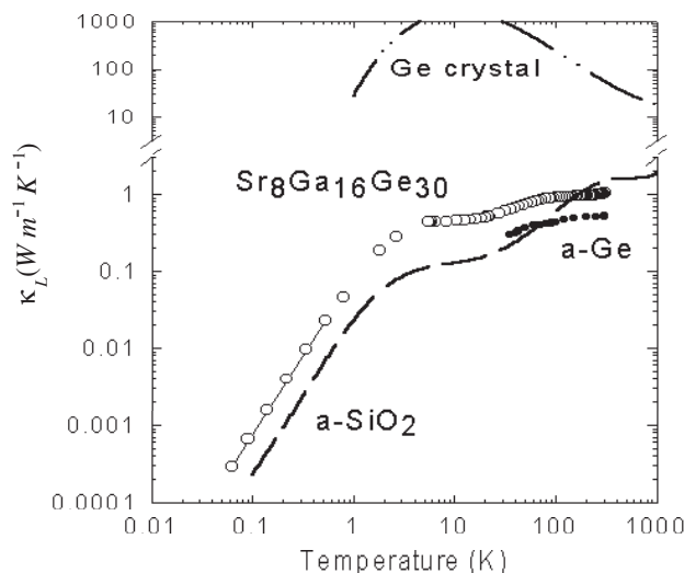
FIGURE 15. Lattice thermal conductivity versus temperature for polycrystalline \text{Sr}_8\text{Ga}_{16}\text{Ge}_{30} , single crystal Ge, amorphous \text{SiO}_2 , and amorphous Ge. The straight line fit to the \text{Sr}_8\text{Ga}_{16}\text{Ge}_{30} data below 1 K produces a T^2 temperature dependence characteristic of glasses.
