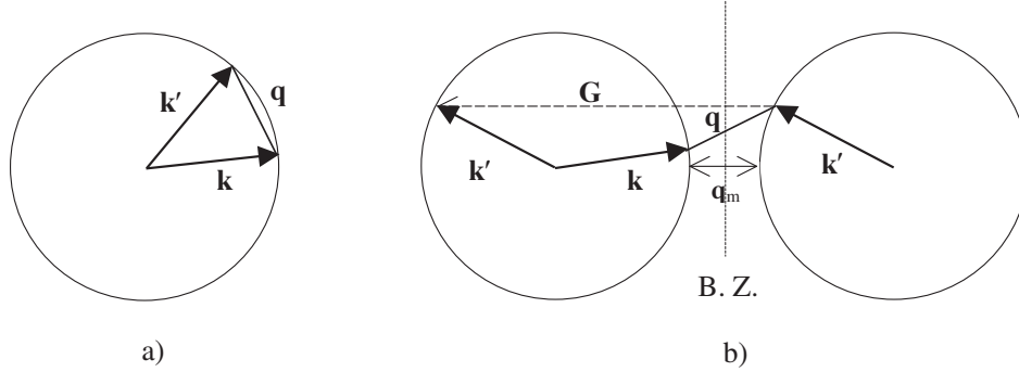
FIGURE 3 (a) Electron-phonon N process \mathbf{k} + \mathbf{q} = \mathbf{k}' . (b) Electron-phonon U process \mathbf{k} + \mathbf{q} = \mathbf{k}' + \mathbf{G} , where \mathbf{G} is the reciprocal lattice vector. Note a minimum phonon wave vector \mathbf{q}_m that is necessary for the U process to take place. At low temperatures such wave vectors may not be available.
