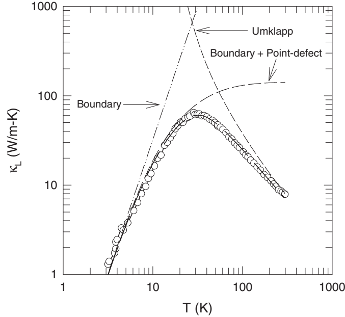
FIGURE 5 The lattice thermal conductivity versus temperature of a CoSb 3 sample from Ref. 21. The dots and the solid line represent the experimental data and the theoretical fit. The dashed curves are the theoretical limits imposed on the phonon heat transport by boundary scatterings, by a combination of boundary plus point defect scatterings, and by umklapp scatterings.
