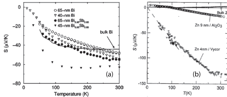
FIGURE 19 T dependence of the TEP comparing bulk and nanowire samples of (a) Bi 39 and (b) Zn. 8,40
