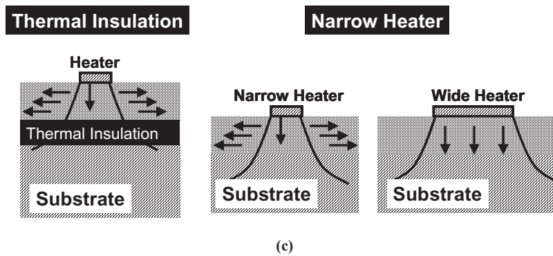
FIGURE 5 Major experimental methods for in plane thermal conductivity characterization: (a) configuration of the membrane method; (b) configuration of the bridge method; (c) in plane heat spreading methods using buried thermal barriers and narrow width heaters. A qualitative comparison between the spreading effects of narrow and wide heaters is shown.
