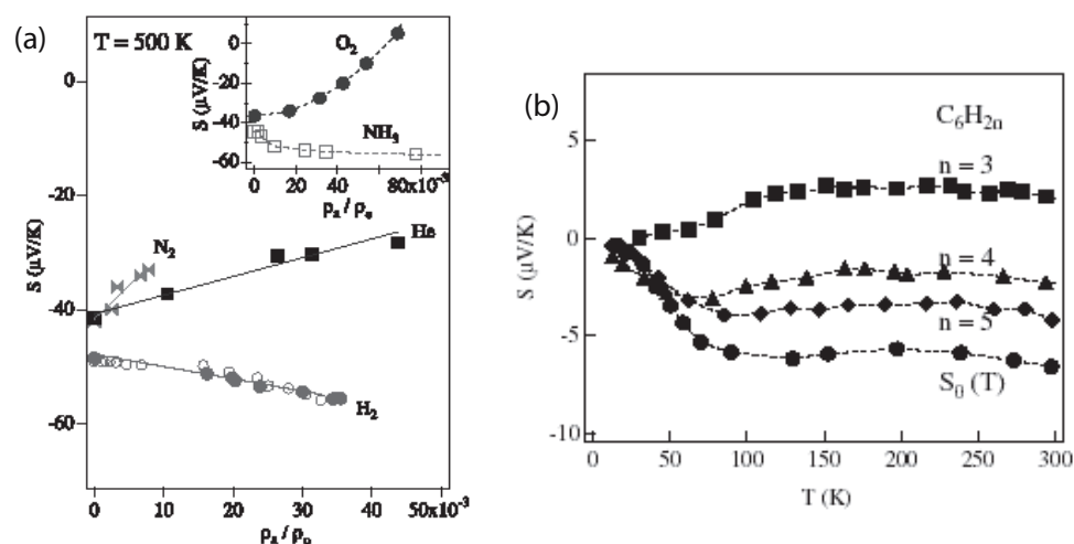
FIGURE 25 (a) Nordheim Gorter ( S vs. p ) plots demonstrating the sensitivity of nanotubes to exposure to various gases as well as indicating the type of adsorption process involved. 50 (b) S(T) data for a degassed SWNT mat and as it was exposed to different hydrocarbon vapors. 51
