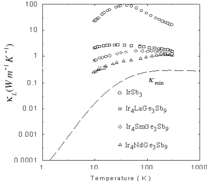
FIGURE 11. Lattice thermal conductivity versus temperature for the La, Sm, and Nd filled skutterudite samples as well as the unfilled IrSb 3 sample. The calculated values of \kappa_{\min} for IrSb 3 are also included. 44 (Reprinted from Ref. 44. Copyright 1996, American Institute of Physics.)
