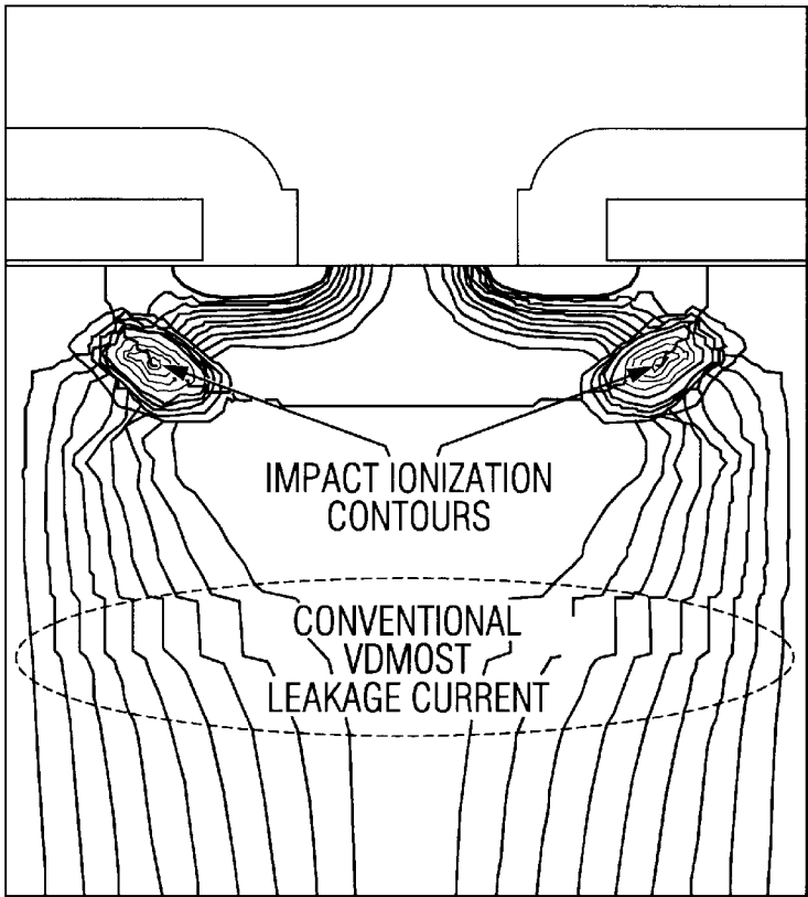
FIG. 3 PRIOR ART
