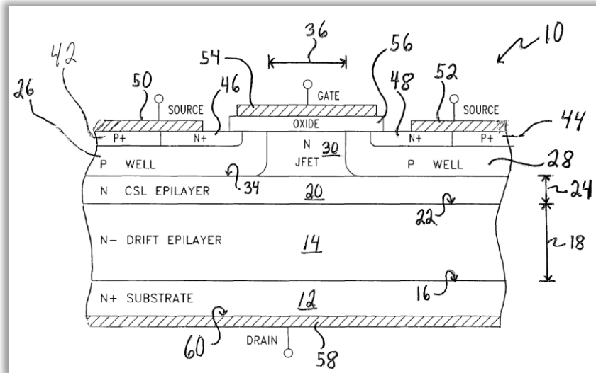
'633 Patent, FIG. 1
