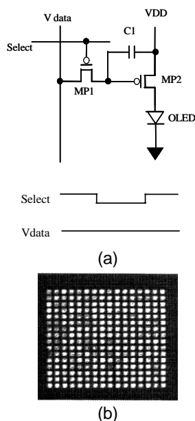
Figure 1 (a) Conventional AMOLED pixel circuit employing two transistors and one capacitor. (b) the brightness non-uniformity (17%) of the conventional 2-TFT pixel [2].
