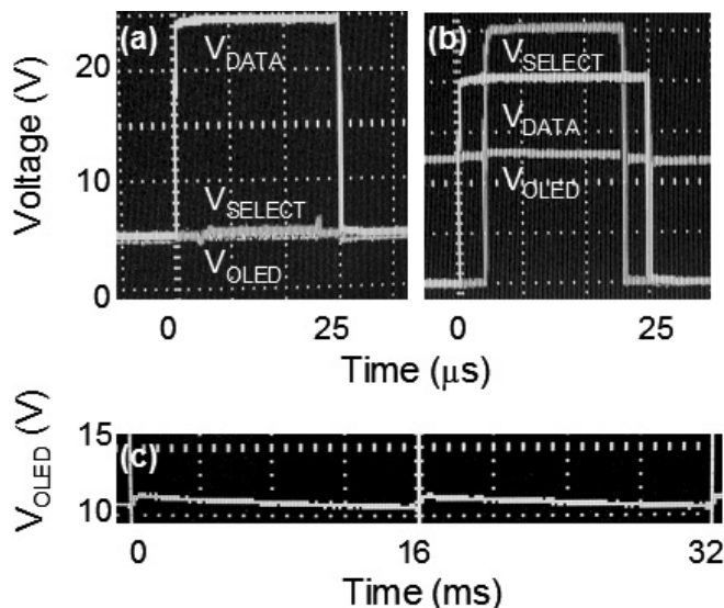
FIGURE 3 — Transient measurements of V_{\text{OLED}} using a 16-msec frame time and V_{\text{DATA}} width of 26 \mu\text{sec} and 20 V for (a) V_{\text{DATA}} = 25 V and V_{\text{SELECT}} = 0 V, (b) V_{\text{DATA}} = 20 V and V_{\text{SELECT}} = 25 V, and (c) two frames.
