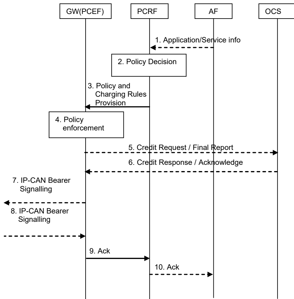
Figure 7.5: IP-CAN Session Modification; PCRF initiated
