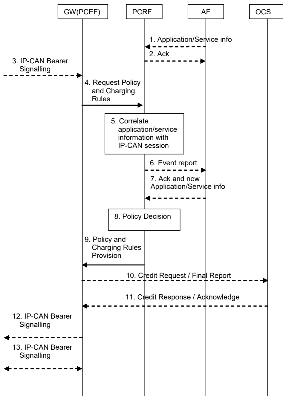
Figure 7.4: IP-CAN Session Modification; GW(PCEF) initiated
