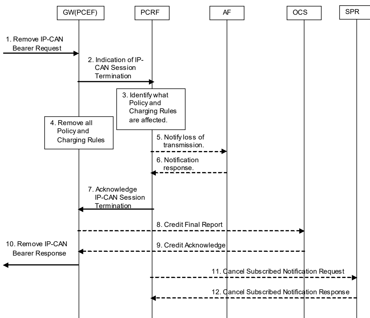
Figure 7.2: IP-CAN Session Termination
