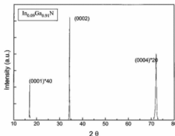
FIG. 6. X-ray \theta-2\theta patterns from \text{In}_{0.09}\text{Ga}_{0.91}\text{N} film showing the presence of the (0001) peak, indicating ordering.
