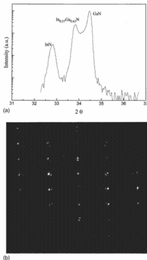
FIG. 1. (a) X-ray diffraction pattern from an InGaN film with 37% indium. (b) Cross-sectional SAD pattern along the [11-20] zone axis from the \text{In}_{0.37}\text{Ga}_{0.63}\text{N} film, showing two sets of superimposed diffraction patterns from InN and InGaN.
