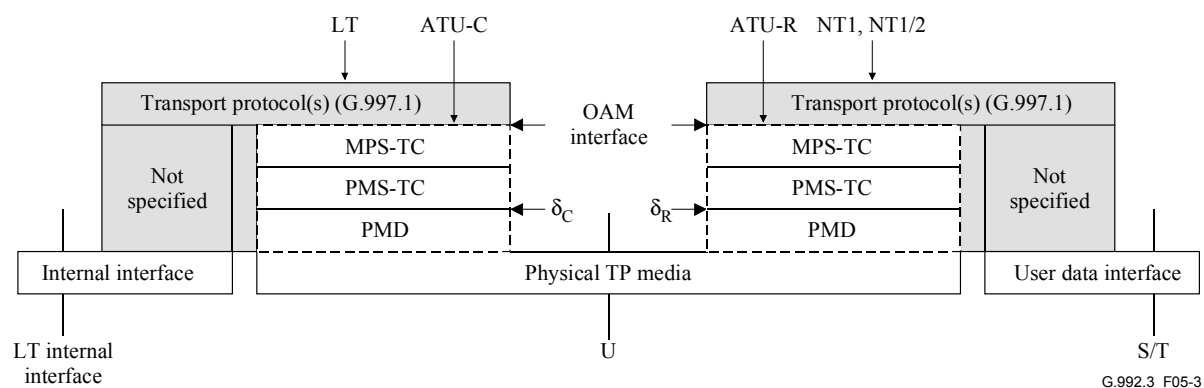
Figure 5-3/G.992.3 – Management plane protocol reference model
