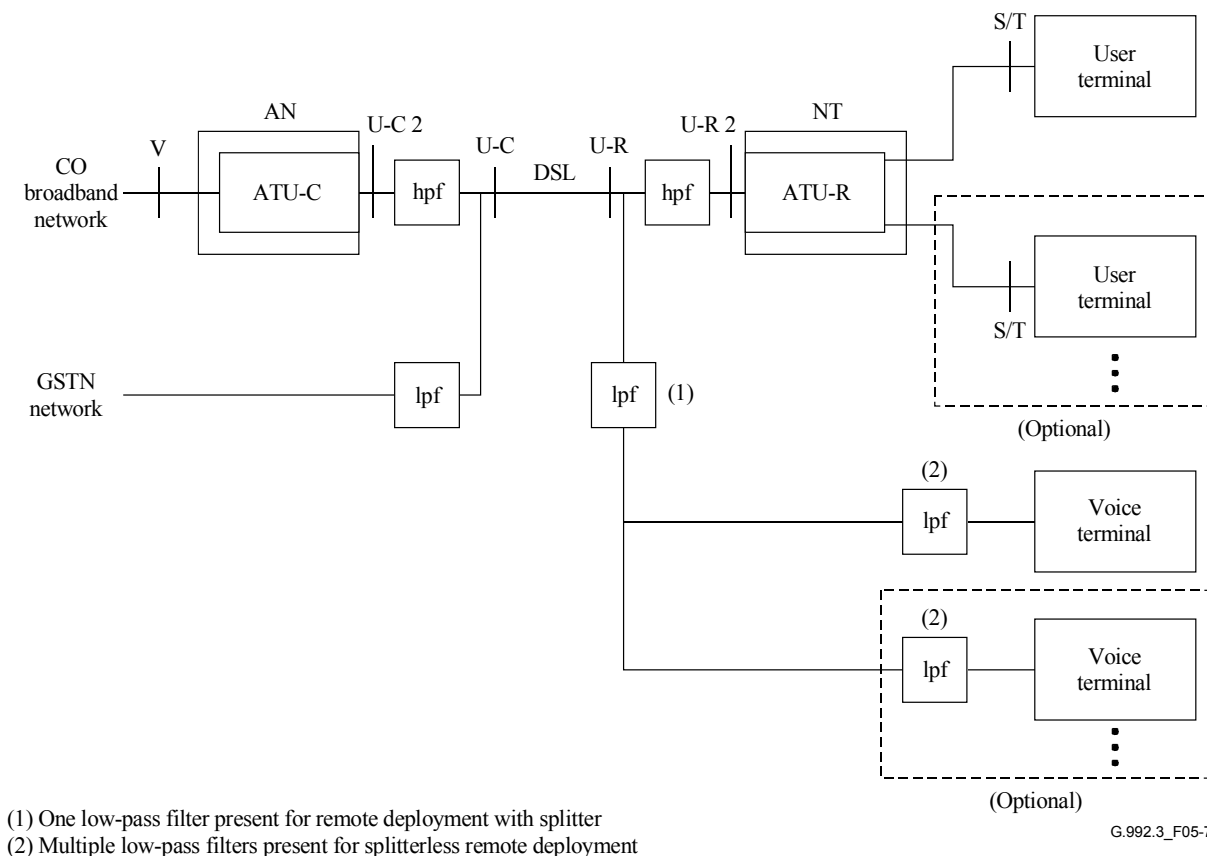
Figure 5-7/G.992.3 – Data with POTS service application model
