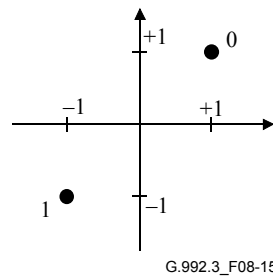
Figure 8-15/G.992.3 – Constellation labels for b = 1
