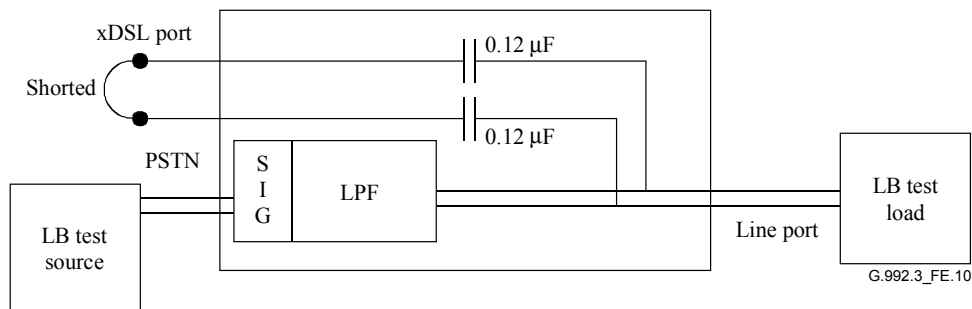
Figure E.10/G.992.3 – Longitudinal balance CO test setup
