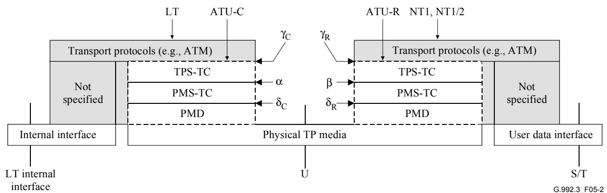
Figure 5-2/G.992.3 – User plane protocol reference model
