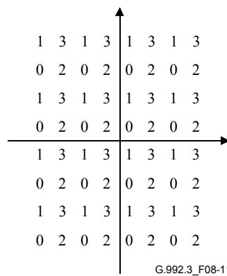
Figure 8-11/G.992.3 – Convolutional encoder
