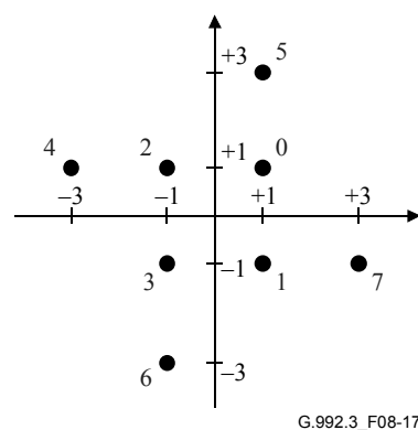
Figure 8-17/G.992.3 – Constellation labels for b = 3
