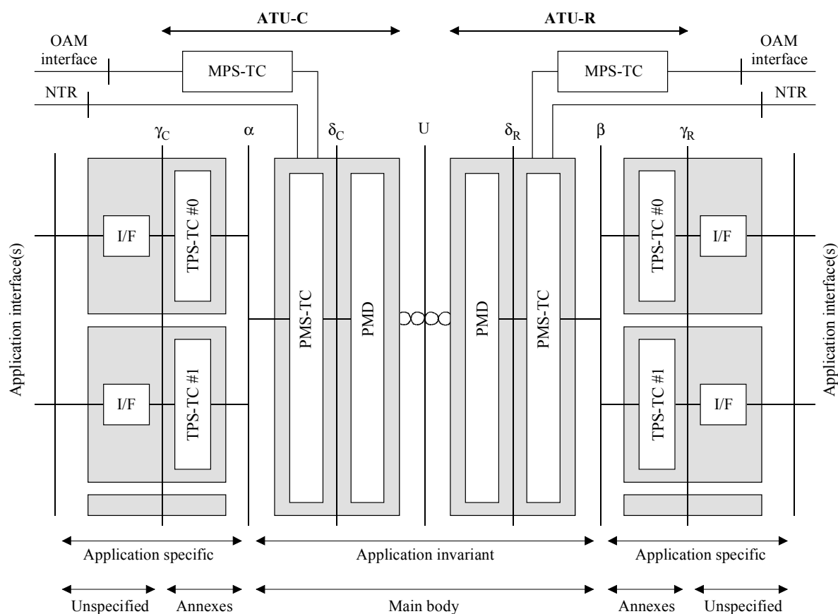
Figure 5-1/G.992.3 – ATU functional model
