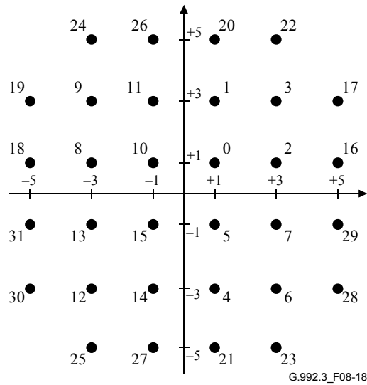
Figure 8-18/G.992.3 – Constellation labels for b = 5
