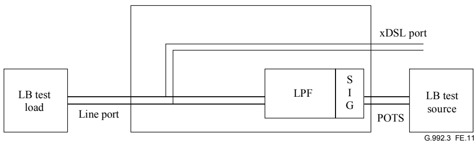
Figure E.11/G.992.3 – Longitudinal balance remote test setup
