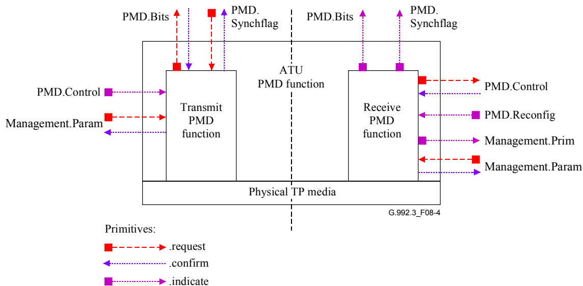
Figure 8-4/G.992.3 – Signals of the ATU PMD function
