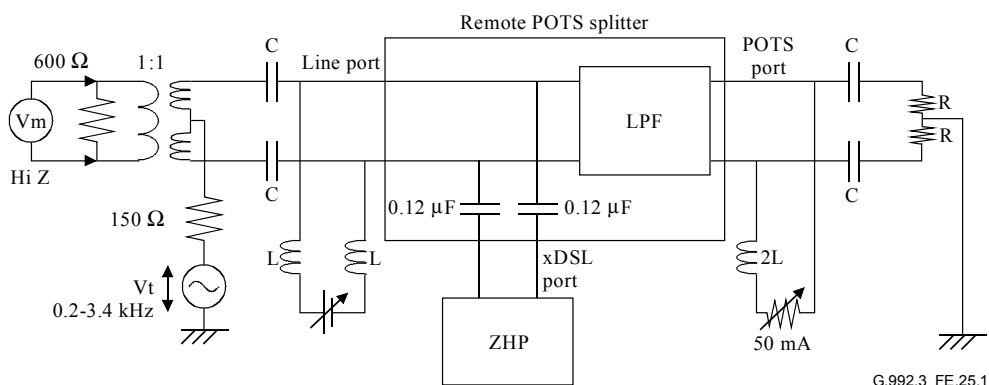
Figure E.24/G.992.3 – Longitudinal balance CO test setup
