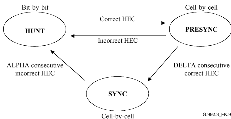
Figure K.9/G.992.3 – Cell delineation procedure state machine
