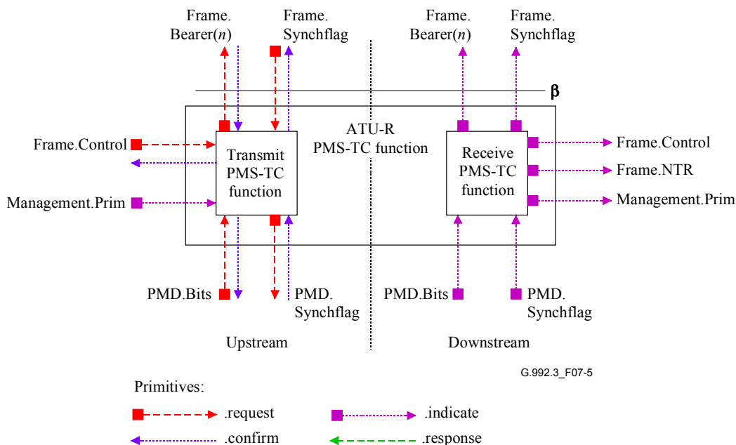
Figure 7-5/G.992.3 – Signals of the ATU-R PMS-TC function
