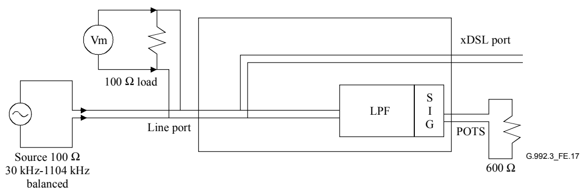
Figure E.17/G.992.3 – Measurement of loading effect of the remote splitter in the ADSL band
