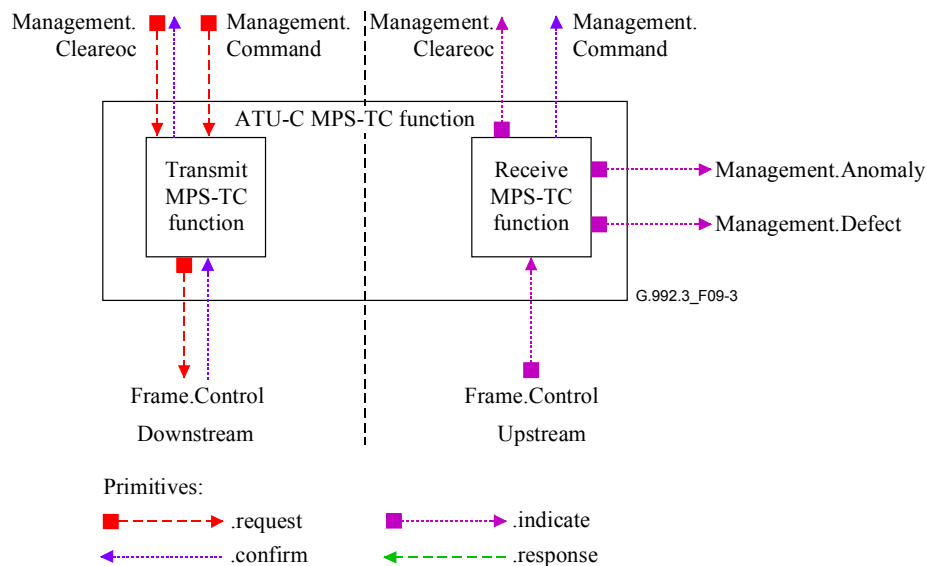
Figure 9-3/G.992.3 – Signals of the ATU-C MPS-TC function
