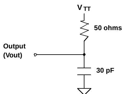
Figure 36: Timing Reference Load
