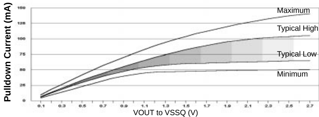
Figure a: Pulldown Characteristics
