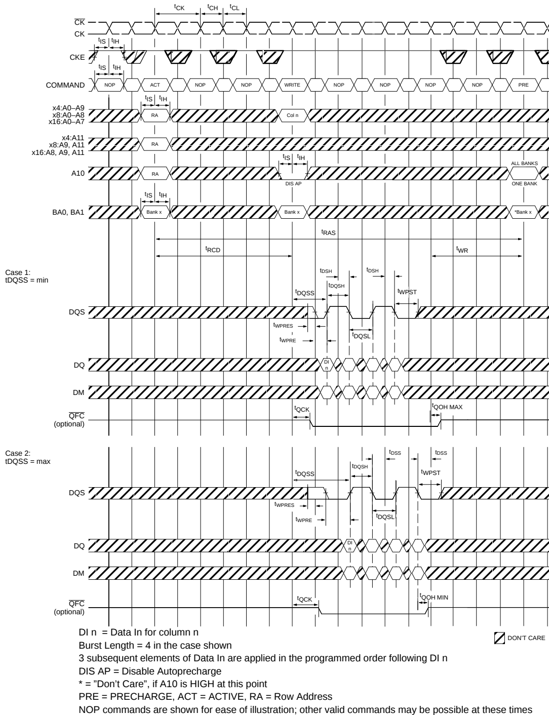
Figure 48 – BANK WRITE ACCESS
