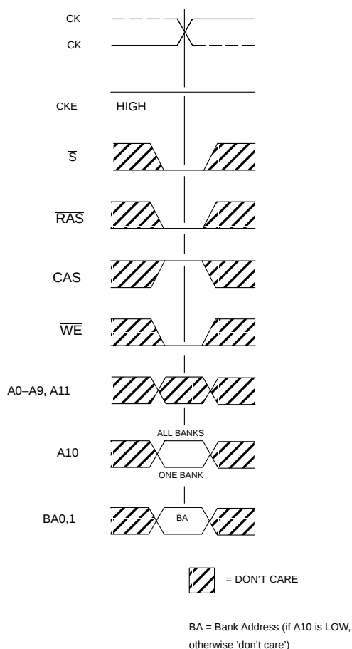
Figure 34 PRECHARGE COMMAND
