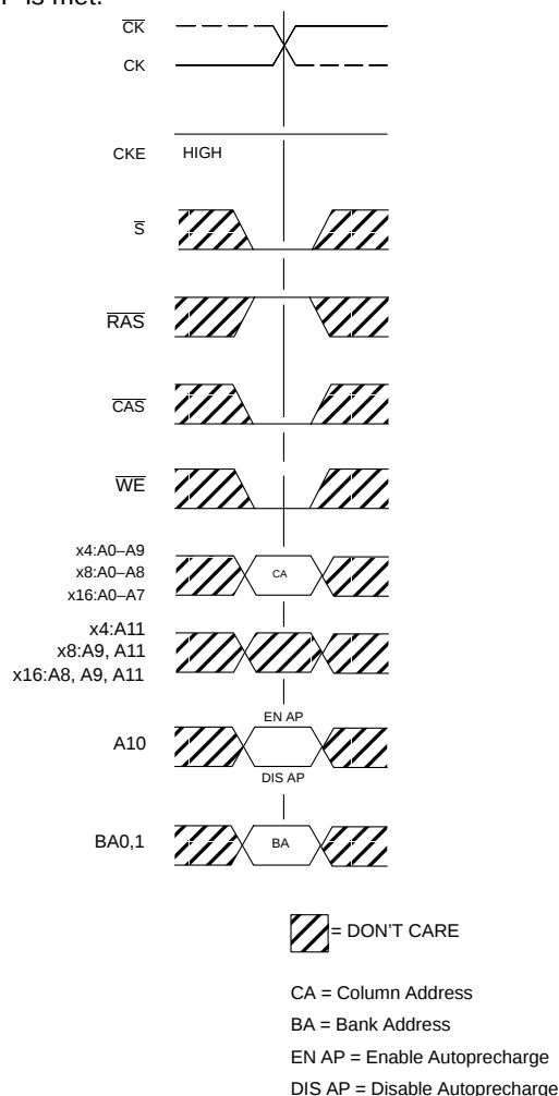
Figure 14 WRITE COMMAND
