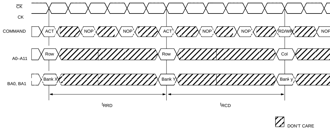
Figure 5 tRCD and tRRD Definition
