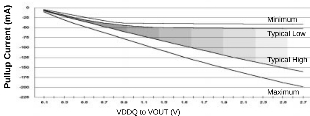
Figure b: Pull Up Characteristics
