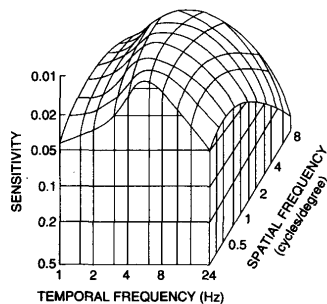
Fig. 11. Spatio-temporal sensitivity of the human visual system (after [100]).
