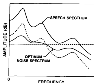
Fig. 26. Three generic forms of noise shaping in the coding of voiced speech (after [6], [65]).
