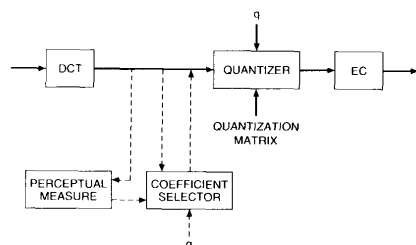
Fig. 42. ISO-JPEG algorithm with perceptual preprocessor.
