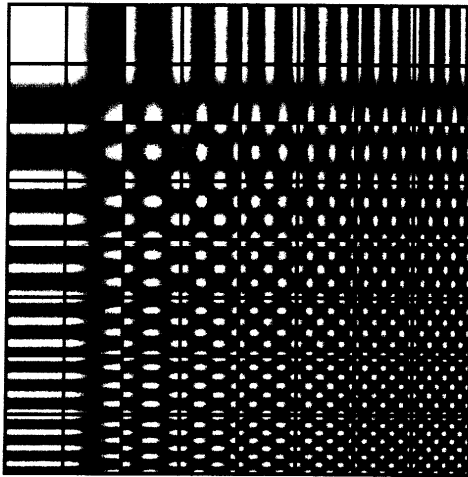
Fig. 13. Basis vectors of a 2D 8 \times 8 Discrete Cosine Transform (DCT).
