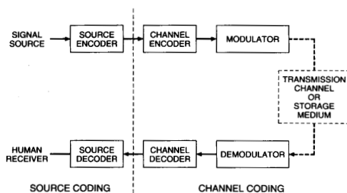
Fig. 2. Block diagram of a digital communication system.
