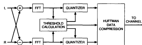
Fig. 35. Block diagram of joint stereo coding.
