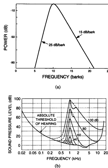
Fig. 30. (a) The spreading function for auditory noise masking. (b) The elevation of auditory threshold due to a critical-band noise masker of varying intensity at 1 kHz.
