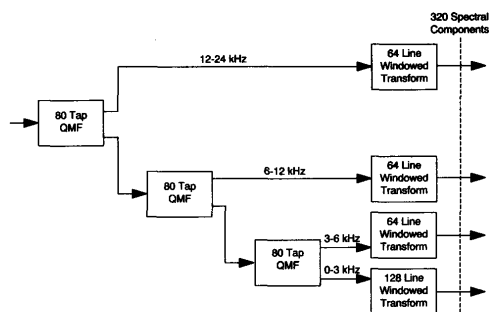
Fig. 34. A hybrid subband-transform analysis system for audio [68].
