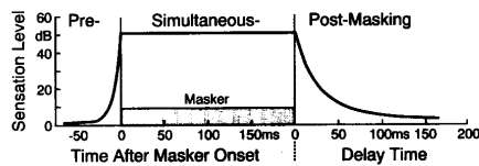
Fig. 32. Temporal masking in the human auditory system.
