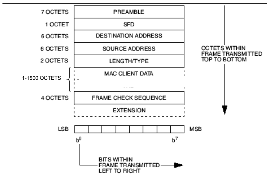
Figure 27: Layer 2 Framing
