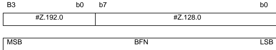
Figure 18: BFN mapping
