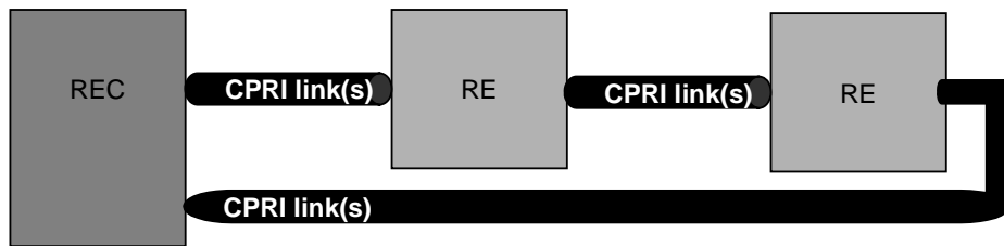
Figure 5C: Ring topology
