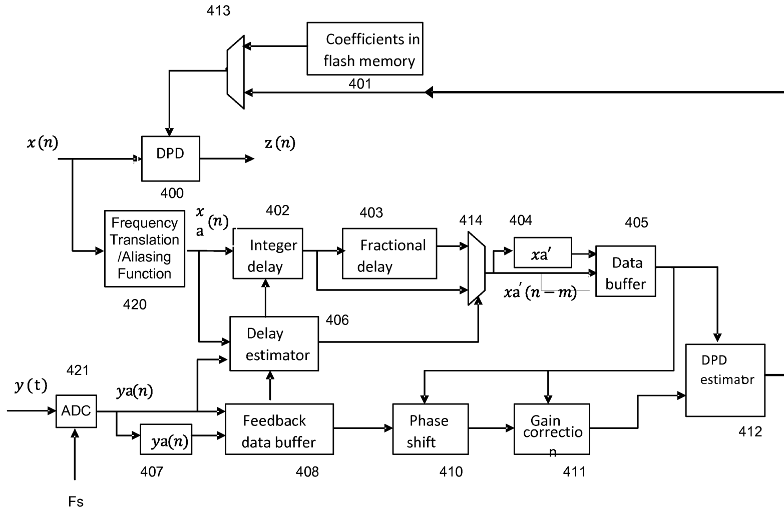
FIG. 4. Digital Predistortion Direct Learning Algorithm
