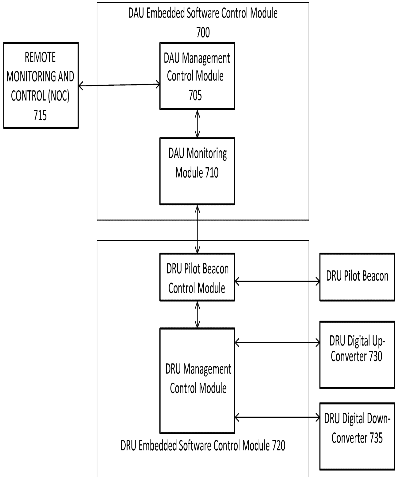
Figure 7: Embedded Software Control Modules
