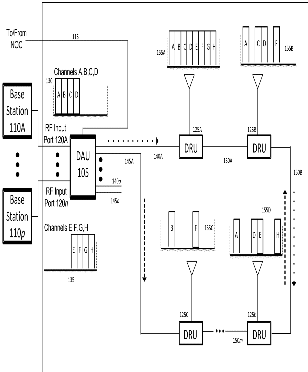
Figure 1: Example of Uni-directional Channels for Downlink
