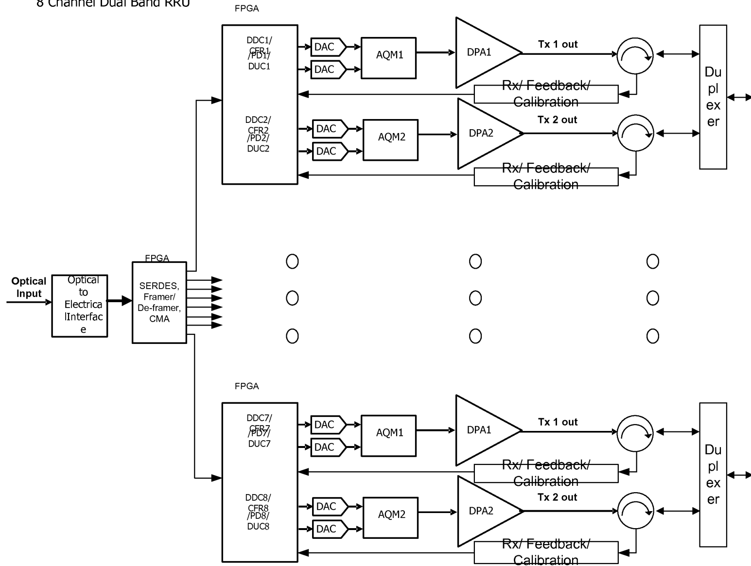
Figure 12 8 Channel Dual Band RRU
