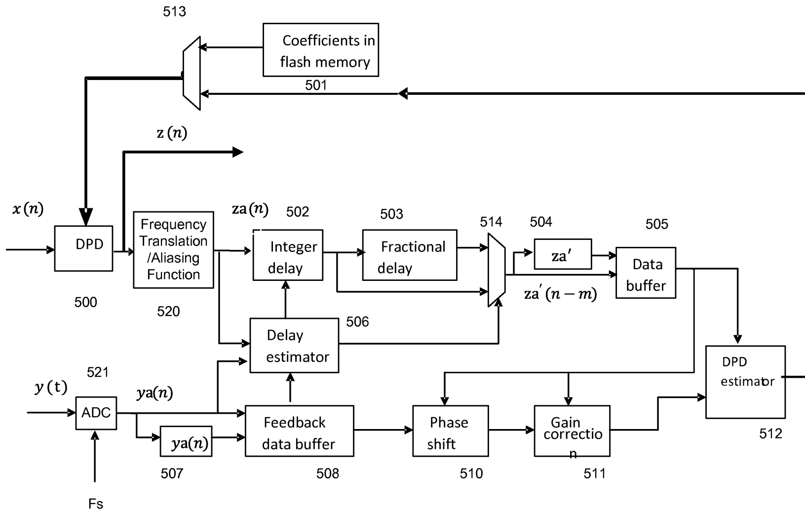
FIG. 5. Digital Predistortion Indirect Learning Algorithm
