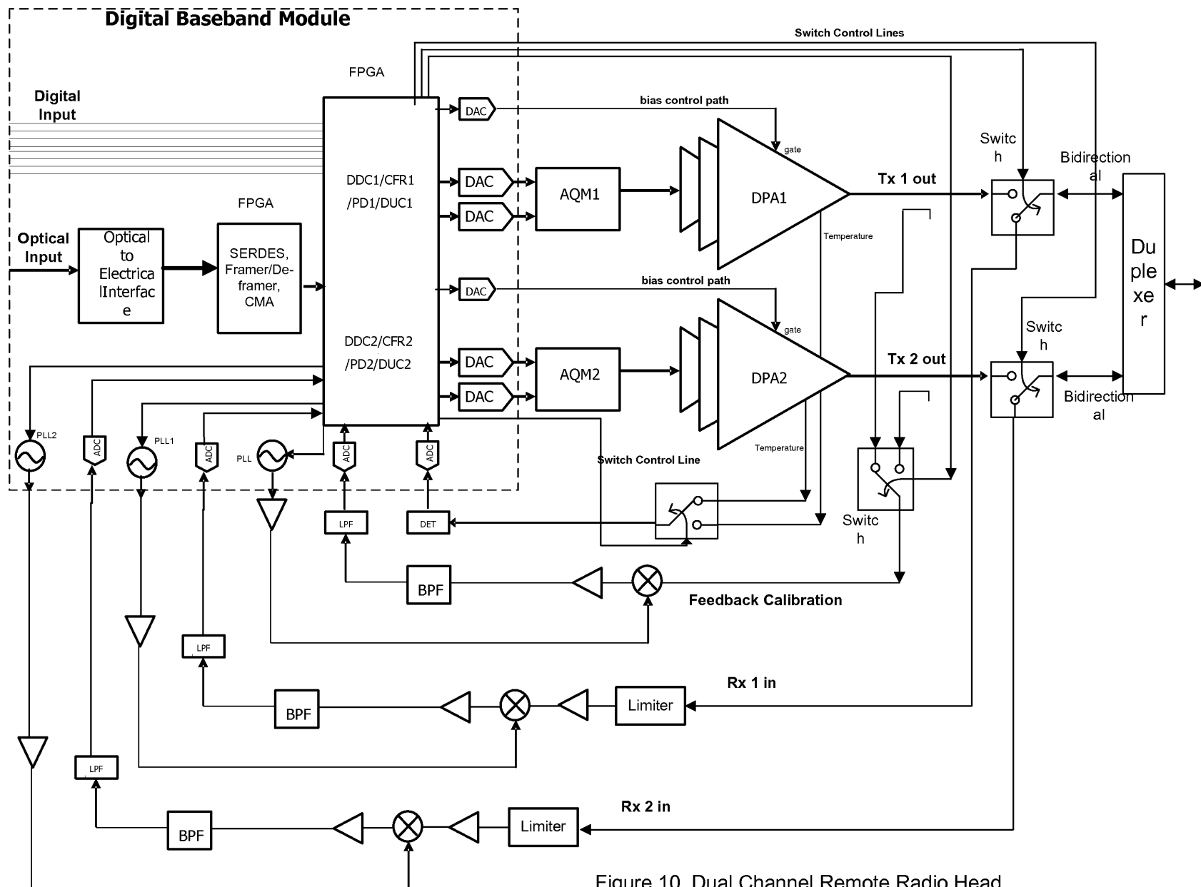
Figure 10 Dual Channel Remote Radio Head
