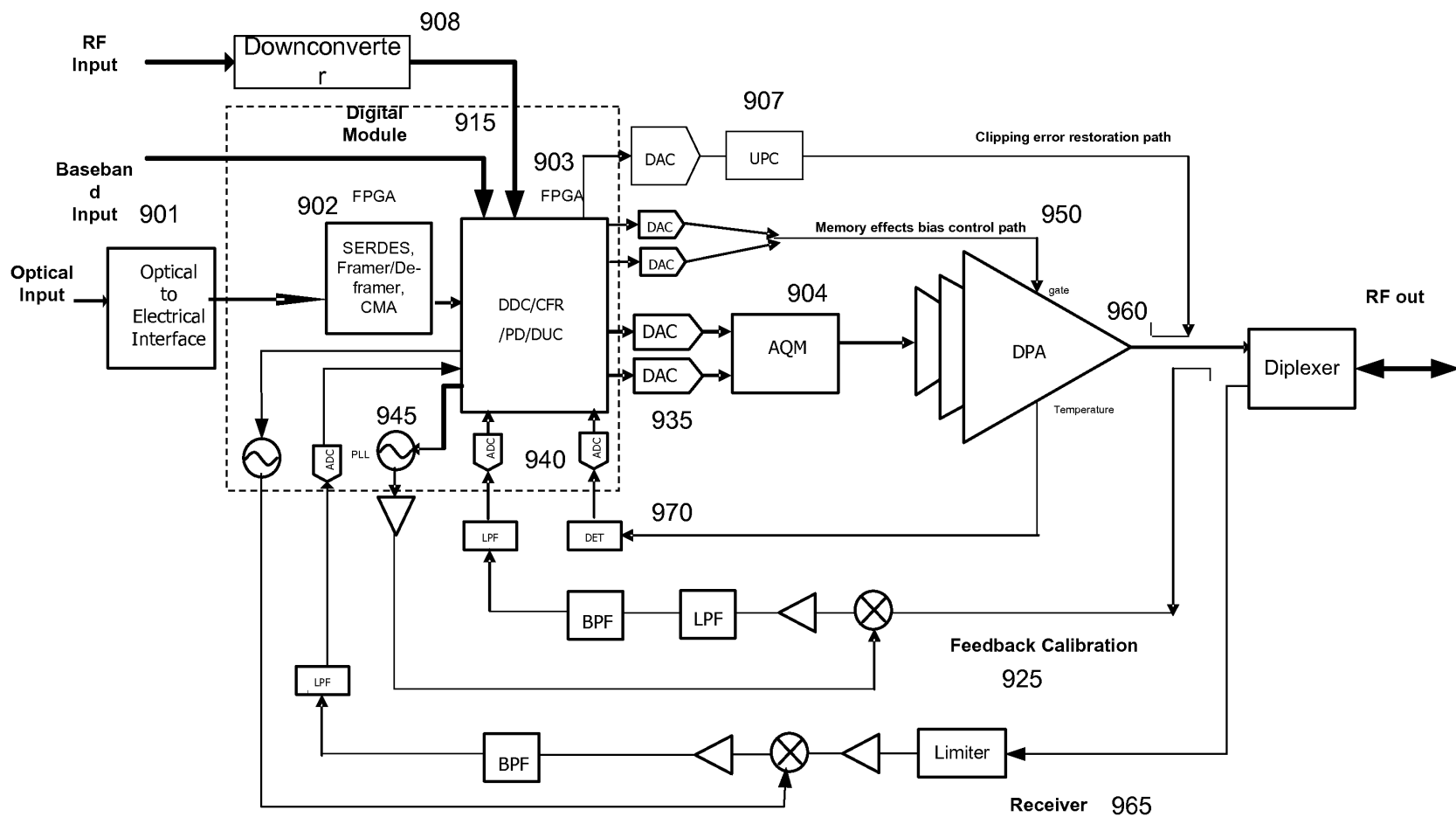
Figure 9 Digital Hybrid Module
