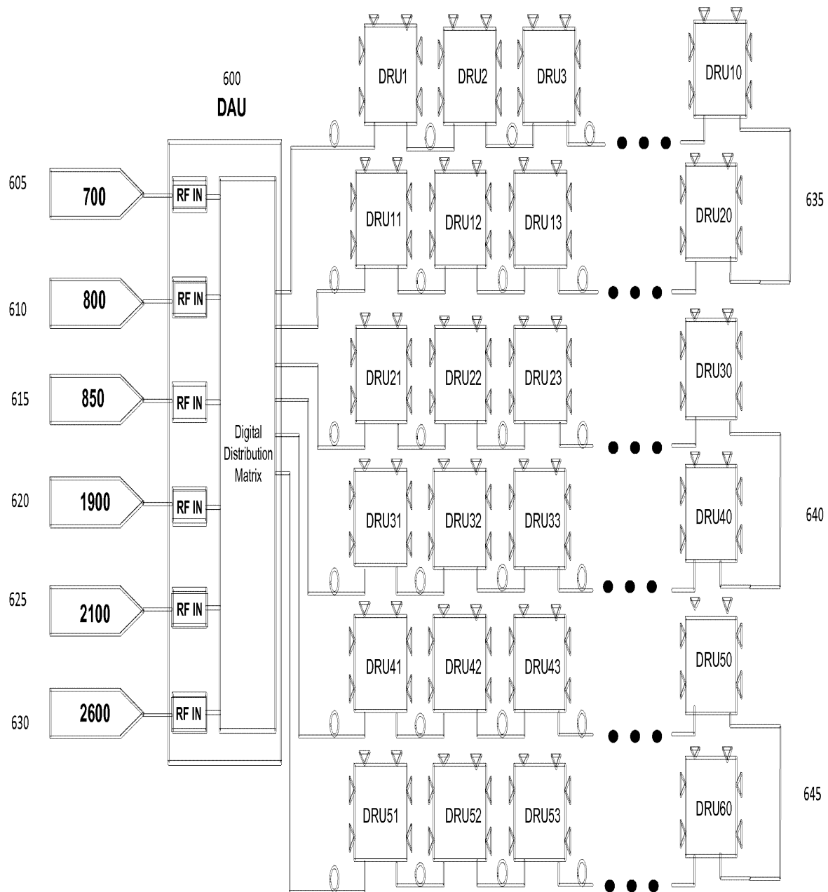
Figure 6. An embodiment of a multi-band system illustrating one DAU supporting up to six different services operating at different frequency bands, with three optical rings of DRU's 1-60.
