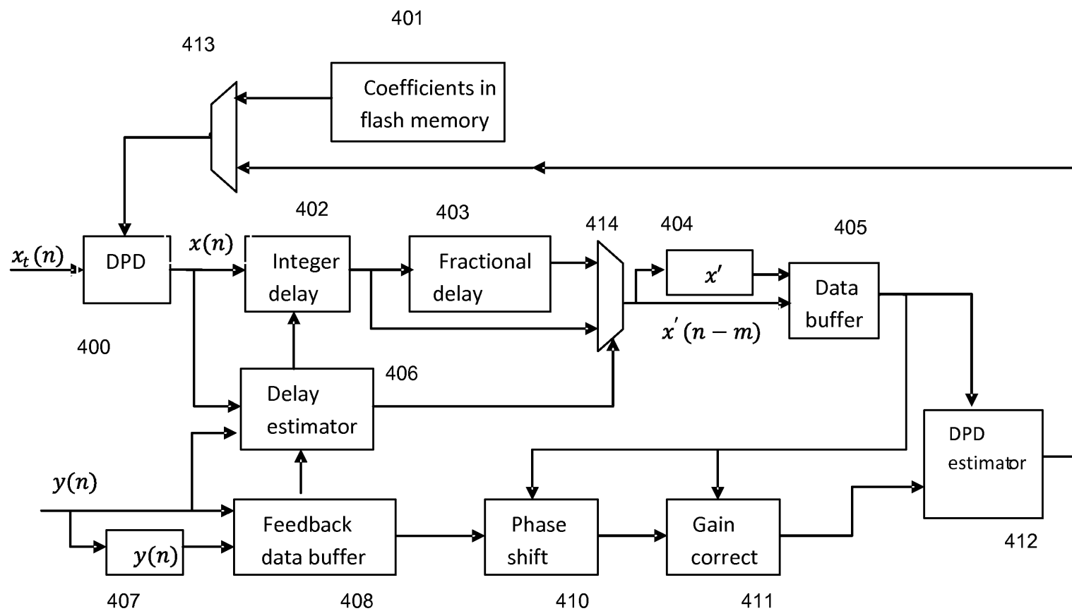
FIG. 4. Digital Predistortion Algorithm
