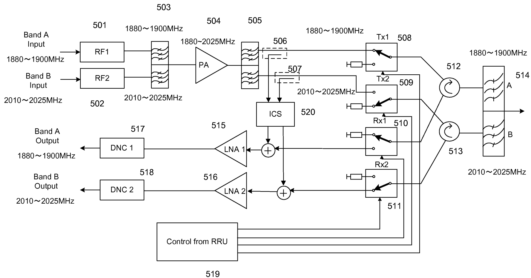
Figure 2: Dual Band TD-SCDMA RRU with Interference Cancellation System
