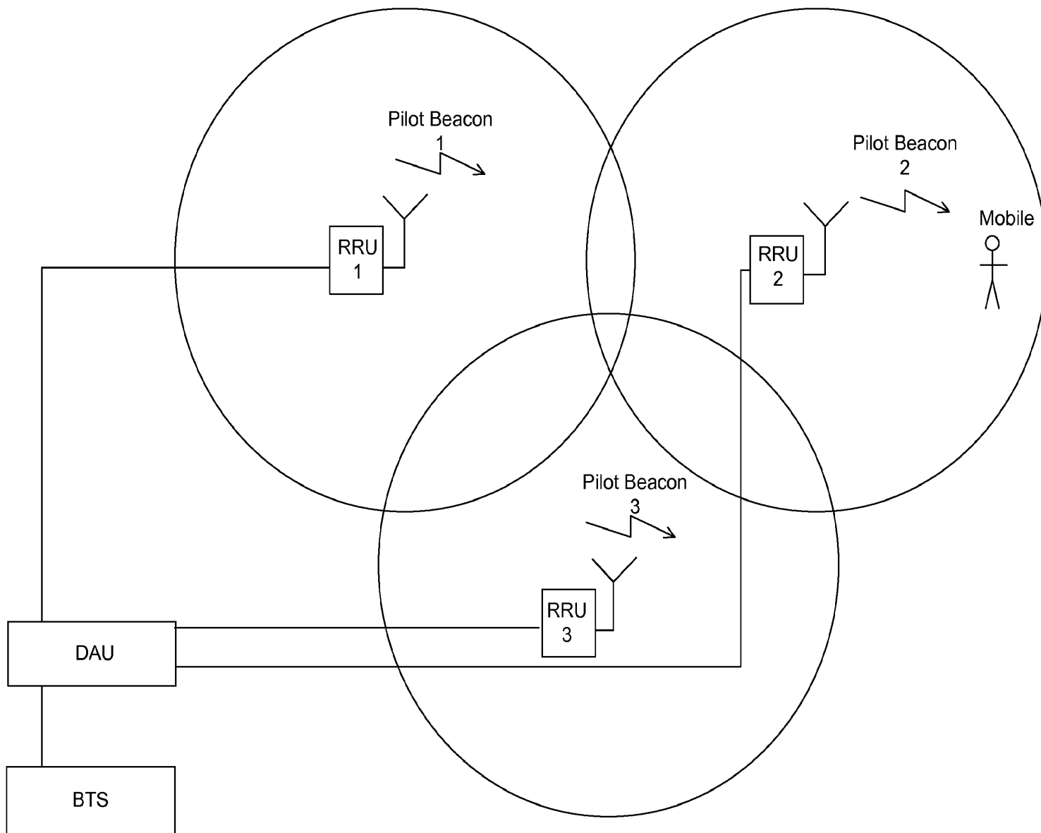
Figure 3 Pilot Beacon Indoor Localization System for CDMA and WCDMA
