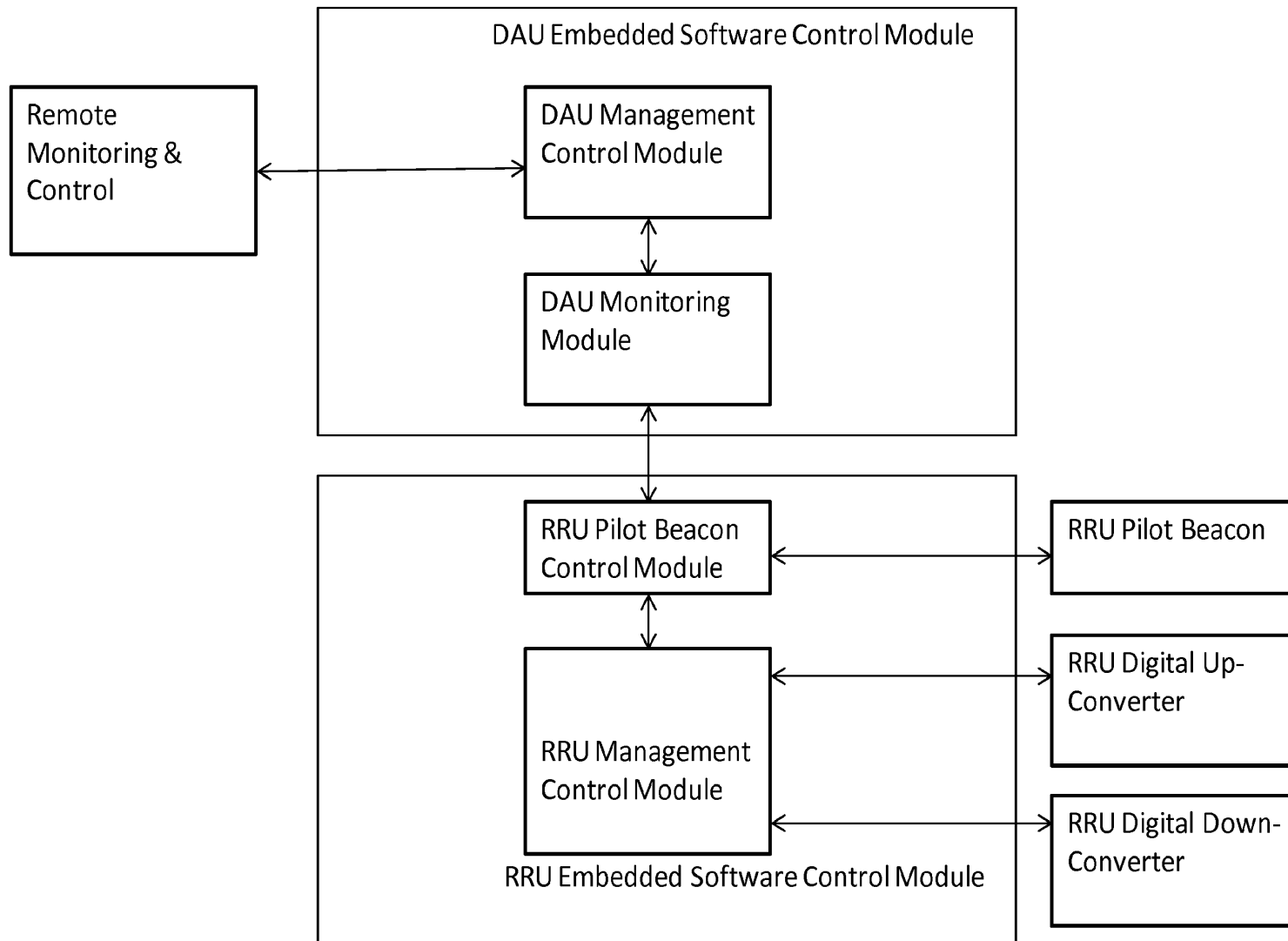
Figure 7: Embedded Software Control Modules
