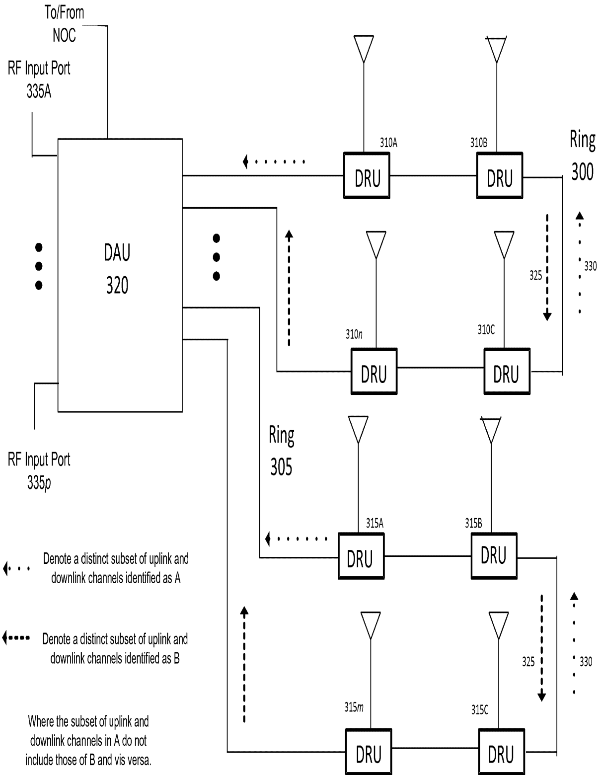
Figure 3: Example of Daisy Chain Ring Network for Uplink
