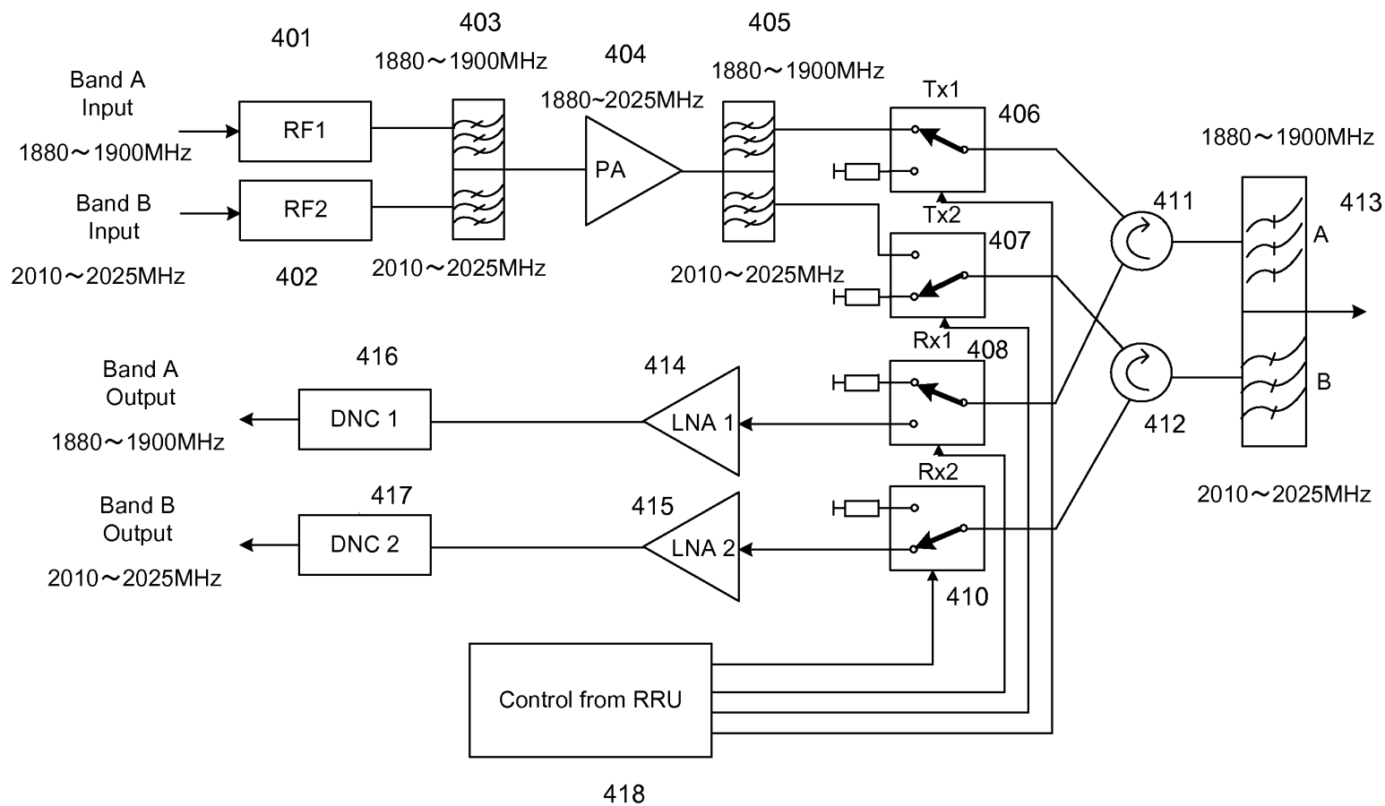
Figure 1: Dual Band TD-SCDMA RRU
