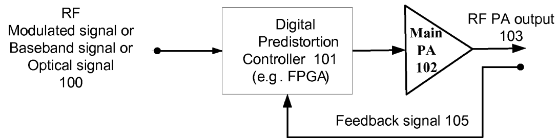
FIG. 1. Basic Digital Hybrid Mode Power Amplifier System
