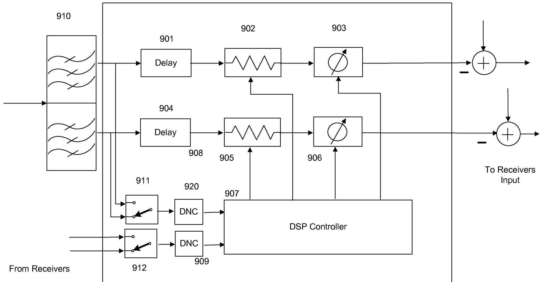
Figure 6: Dual-Band Interference Cancellation System using Correlation
