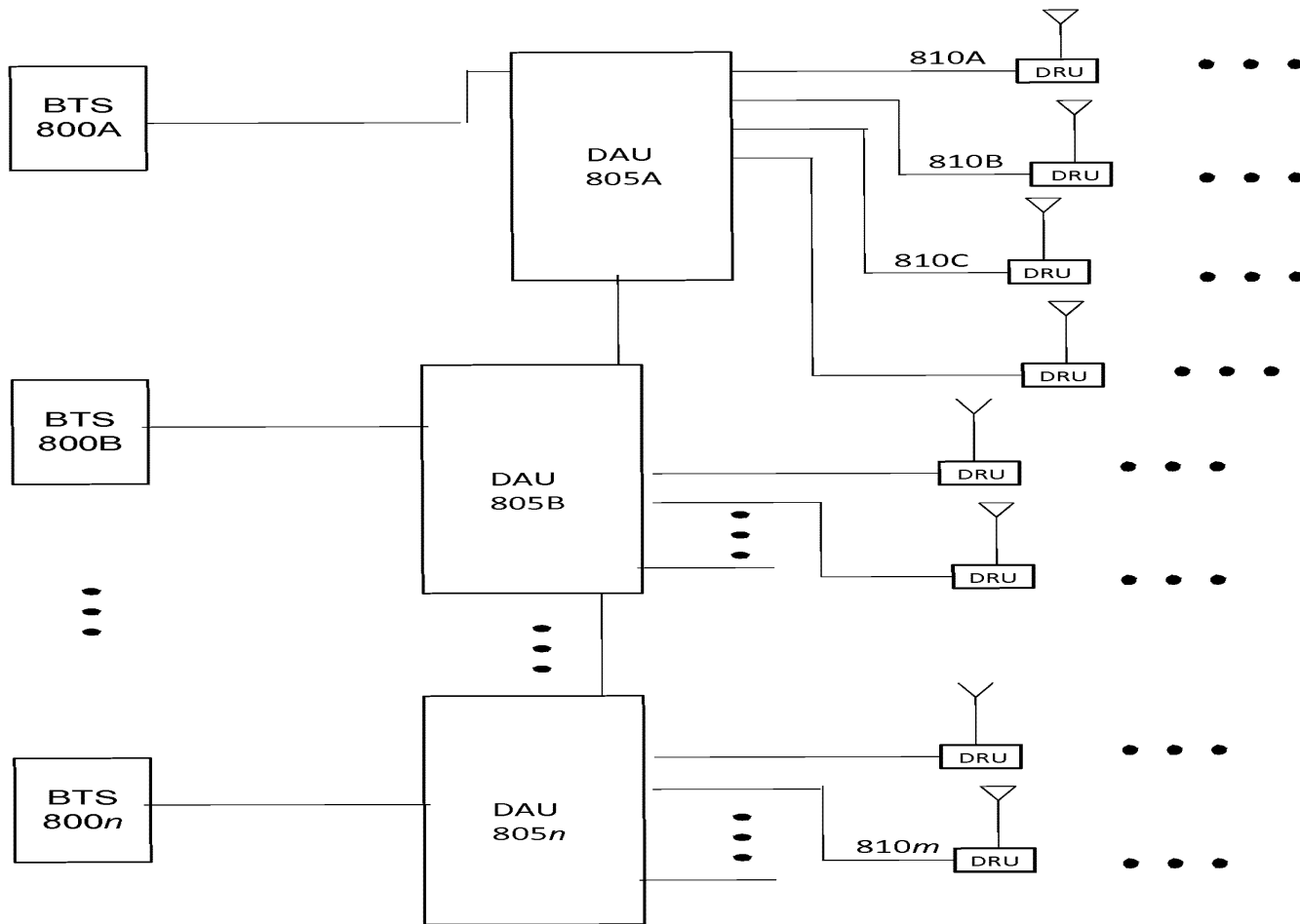
Figure 8 Daisy Chained DAUs
