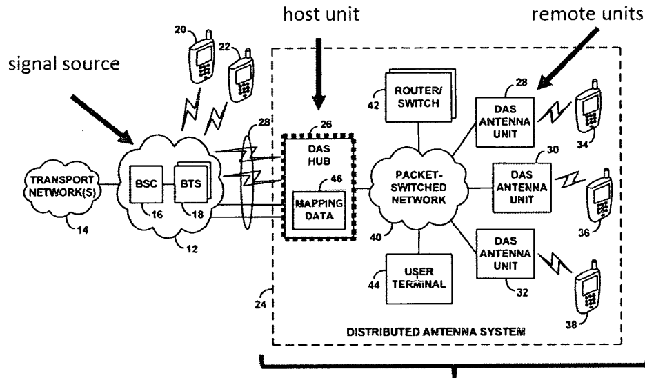
FIG. 1 system transporting wireless communication
