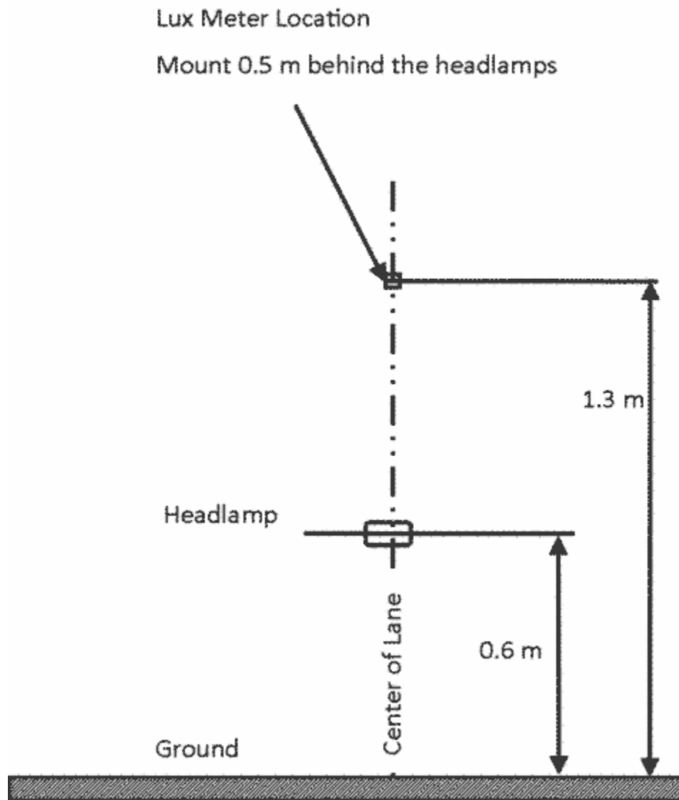
Motorcycle opposite direction stimulus test fixture dimensions
