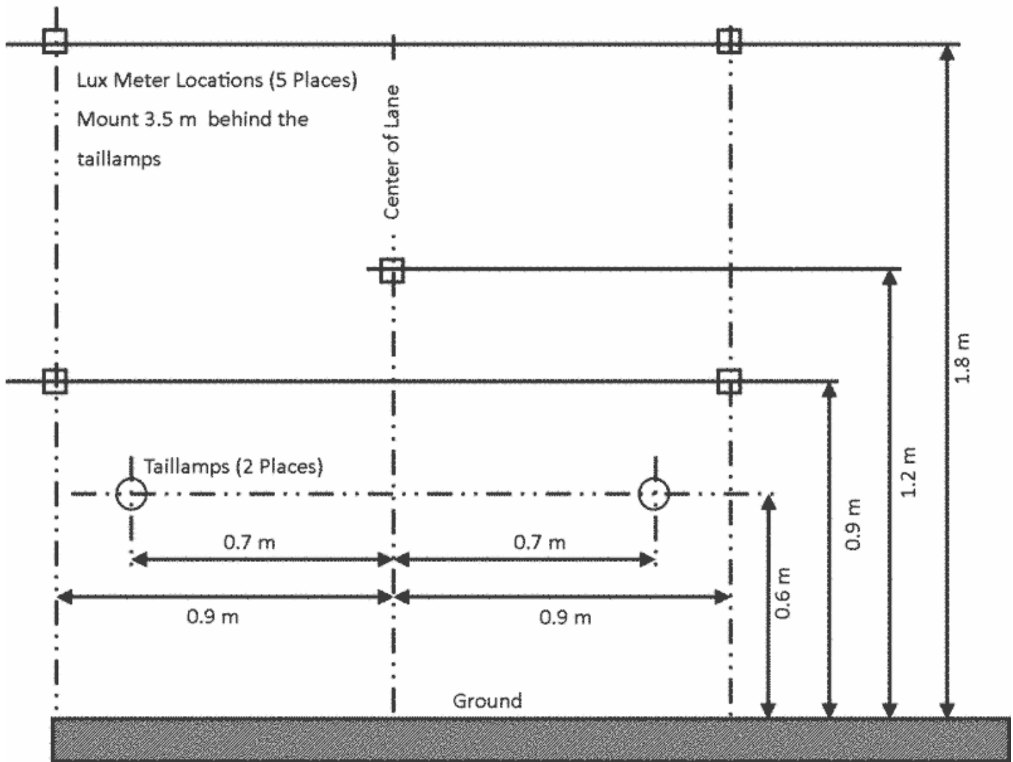
Car / Truck same direction stimulus fixture dimensions
