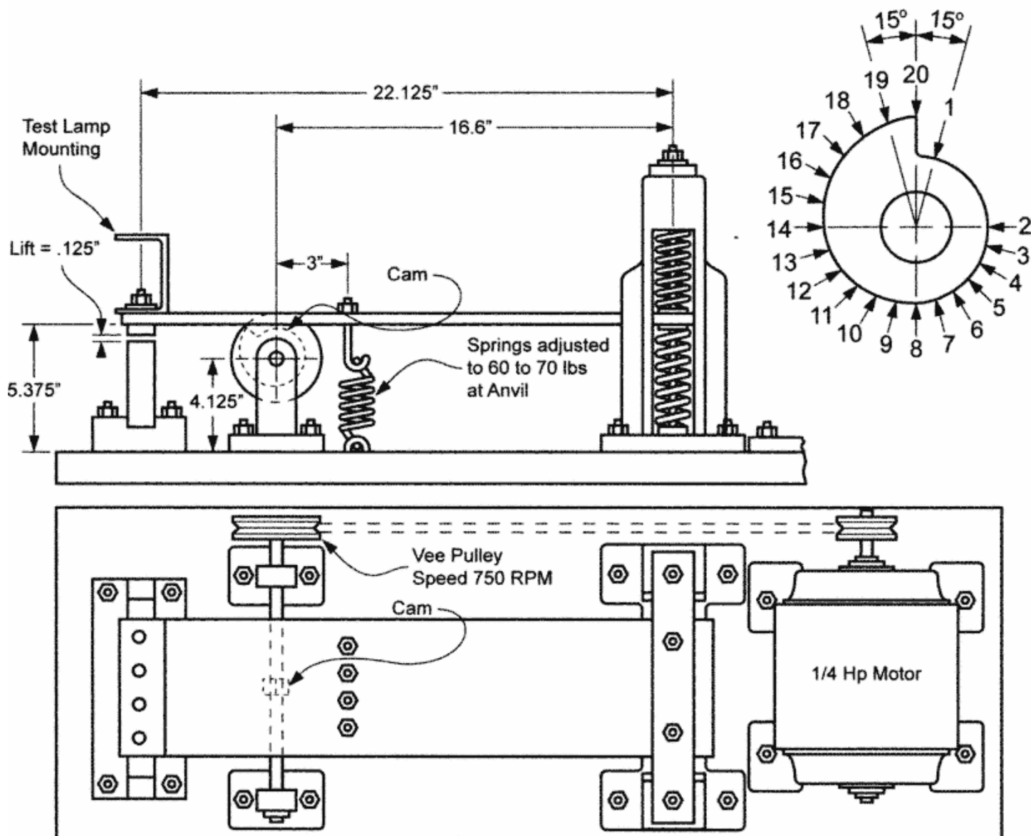
FIGURE 21 VIBRATION TEST MACHINE
