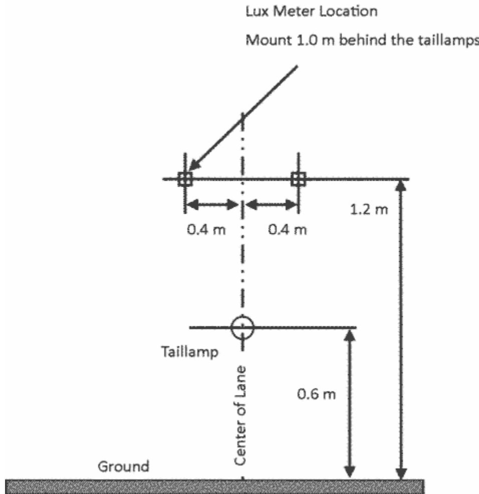
Motorcycle same direction stimulus test fixture dimensions
