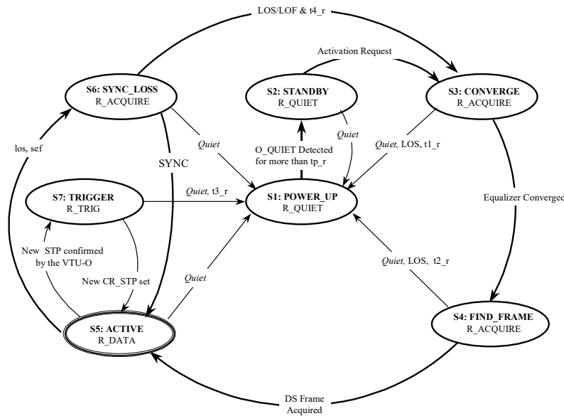
Figure 61: VTU-R Activation/Deactivation State Machine
