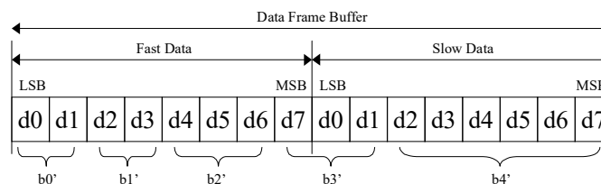
Figure 10: Bit extraction after tone ordering
