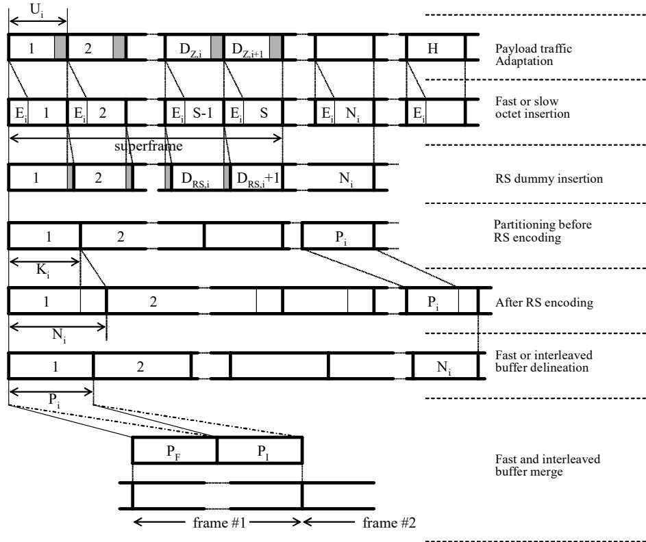
Figure 34: Framing description
