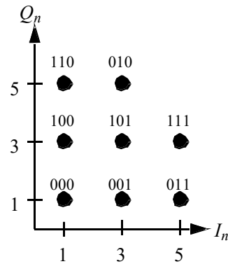
Figure 17: 8-point Constellation and Bit Mapping
