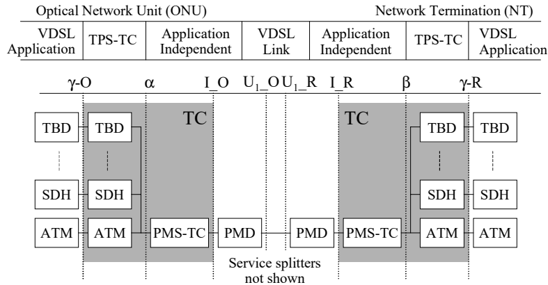
Figure 3: Functional decomposition
