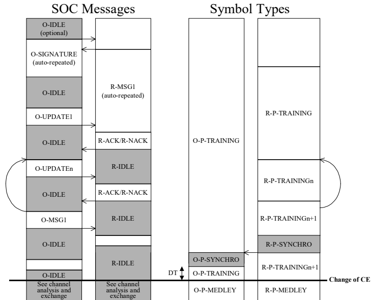
Figure 53: Timeline of training phase
