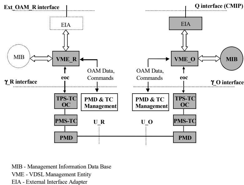
Figure 48: eoc functional model
