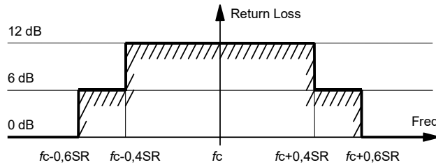
Figure 24: Return Loss Mask
