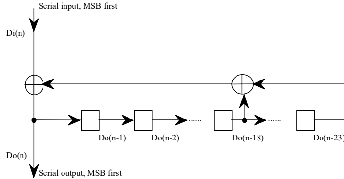
Figure 40: Randomiser
