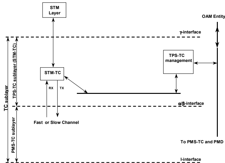
Figure 27: Functional Model of STM Transport
