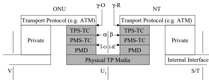
Figure 2: VDSL protocol layer model
