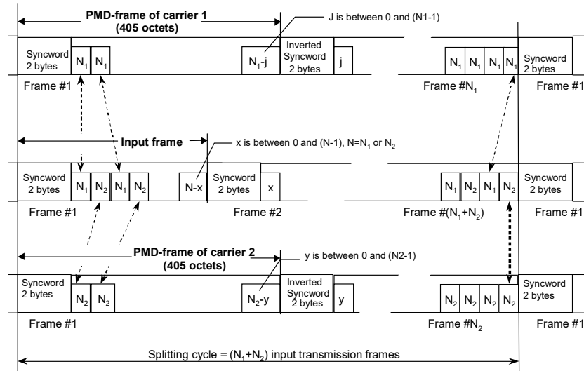
Figure 12: PMD-frame Format
