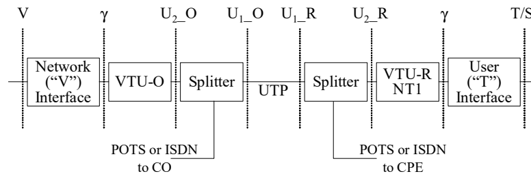
Figure 1: Interface reference model
