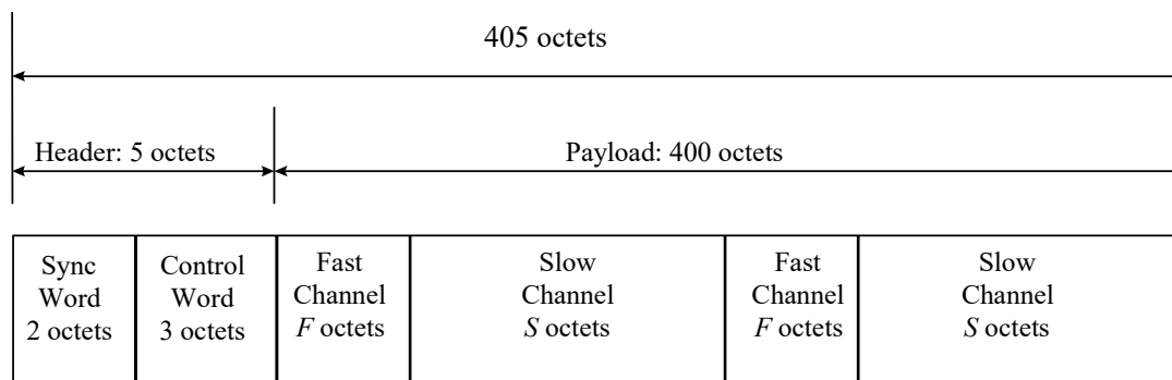
Figure 36: Transmission Frame Format
