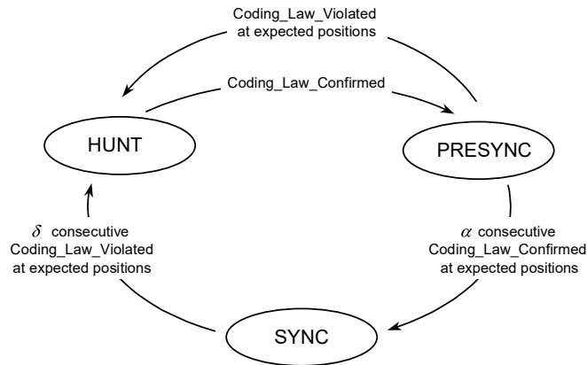
Figure 29: ATM Cell Delineation State Machine
