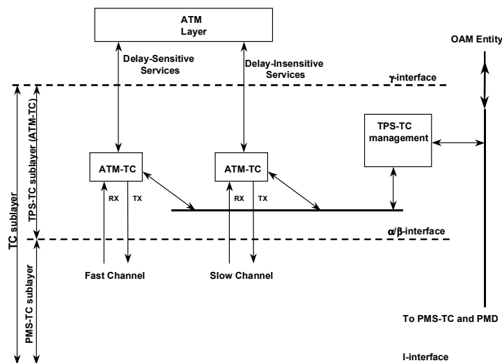
Figure 26: Functional Model of ATM Transport
