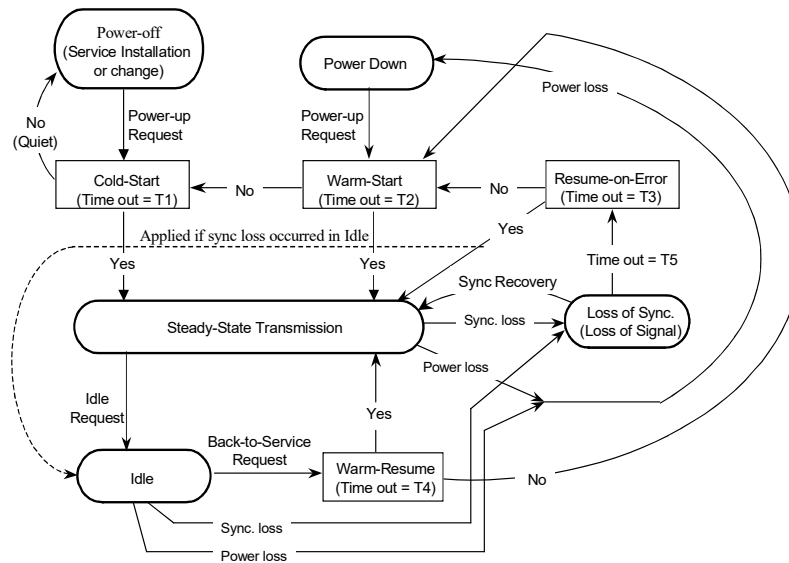
Figure 57: Link State and Timing Diagram
