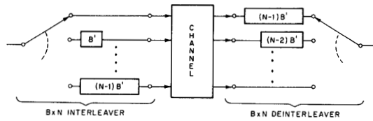
Fig. 2. Periodic interleaver and corresponding deinterleaver ( B' = B/N ).
