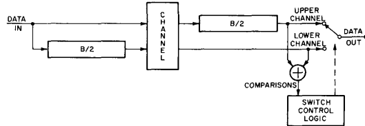
Fig. 6. Zegers' time-diversity scheme.
