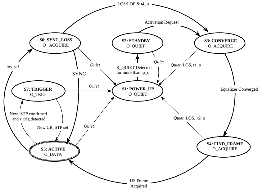
Figure 59: VTU-O Activation/De-activation State Machine
