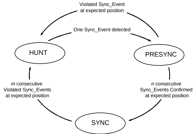
Figure B.1: Frame Delineation State Machine
