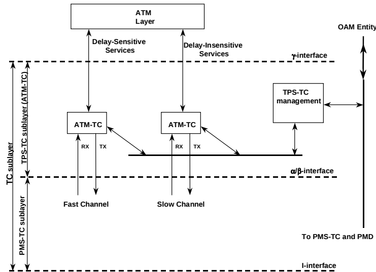
Figure 26: Functional Model of ATM Transport
