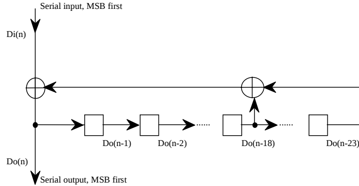
Figure 40: Randomiser
