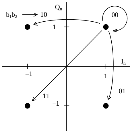
Figure 16: 4-point Constellation with Differential Bit Encoding
