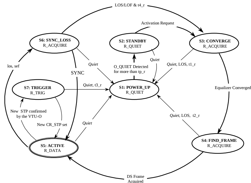
Figure 61: VTU-R Activation/Deactivation State Machine
