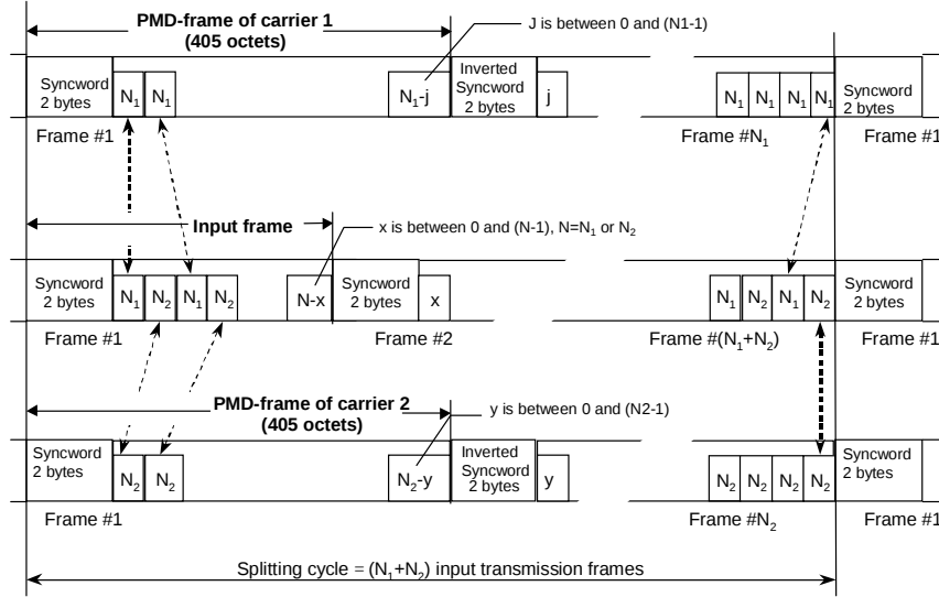
Figure 12: PMD-frame Format
