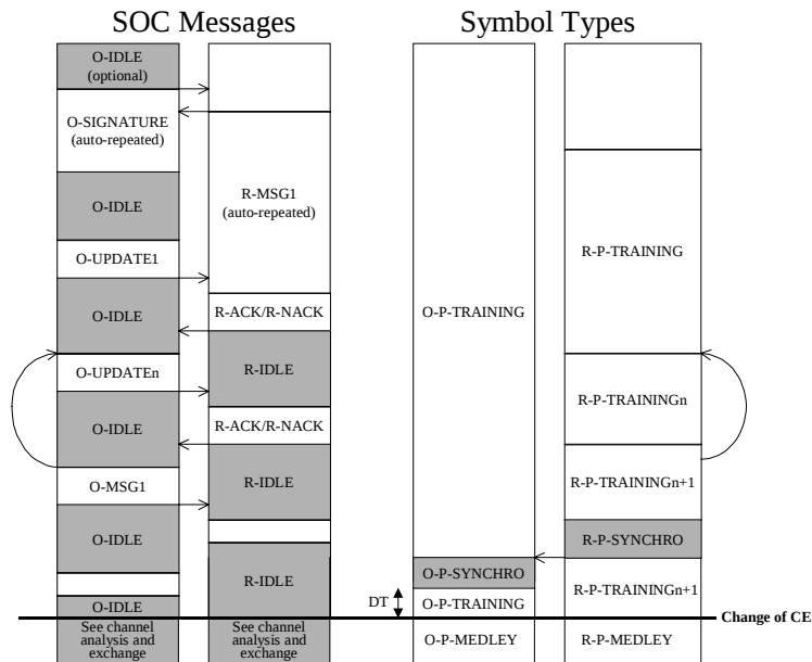
Figure 53: Timeline of training phase
