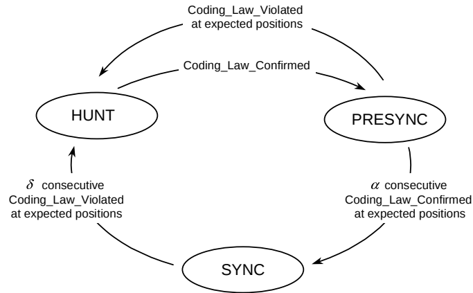
Figure 29: ATM Cell Delineation State Machine
