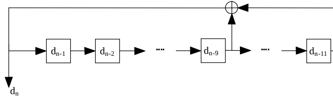
Figure 54: Pseudo-random bit generator
