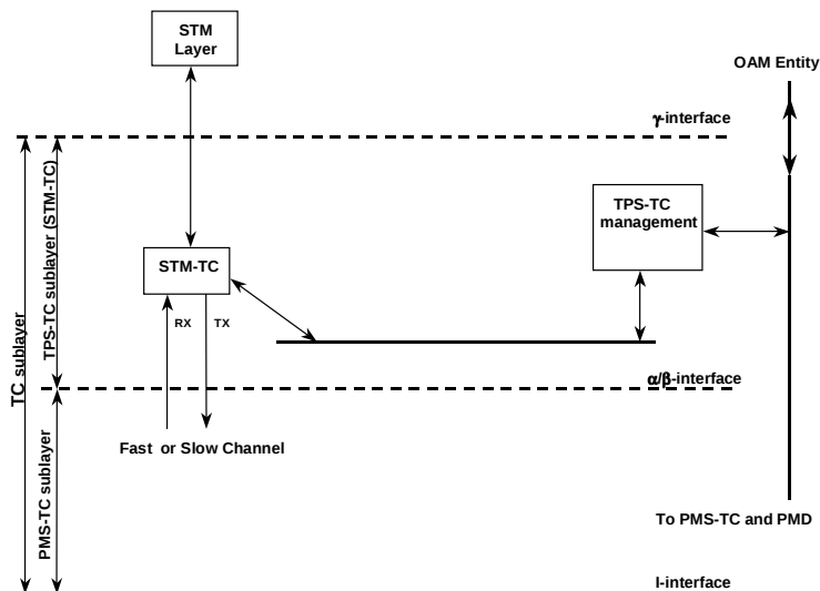
Figure 27: Functional Model of STM Transport
