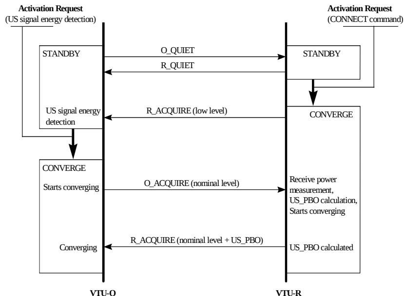
Figure 63: Activation From the VTU-R
