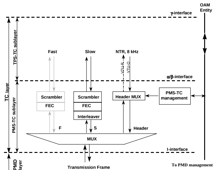
Figure 32: PMS-TC functional model
