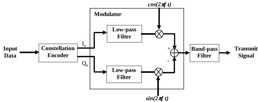
Figure 14: Block Diagram of a SCM Transmitter Using BSS
