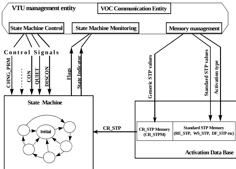
Figure 58: VTU- Activation/Deactivation Functional Diagram
