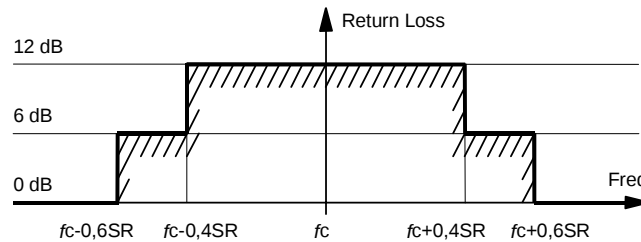
Figure 24: Return Loss Mask
