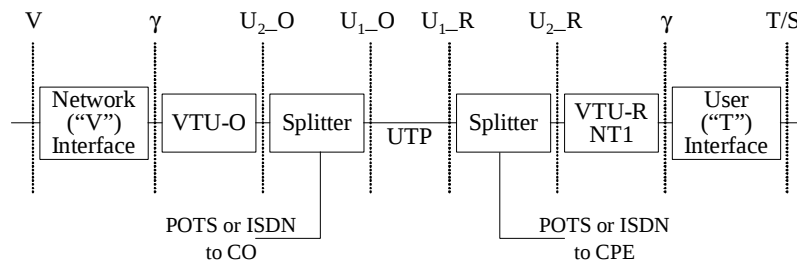
Figure 1: Interface reference model
