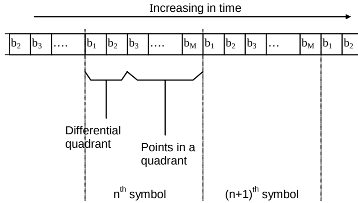
Figure 15: Bit to symbol mapping
