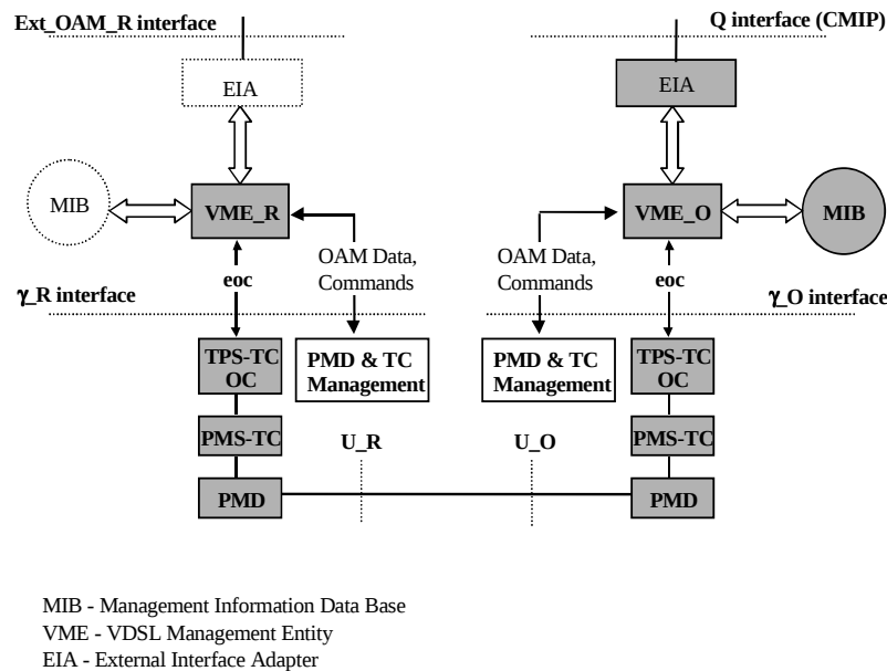
Figure 48: eoc functional model
