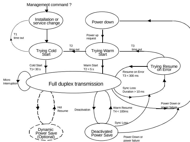
Figure 49: Activation/de-activation state and timing diagram
