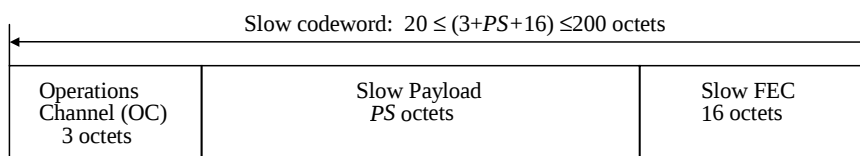
Figure 38: Structure of Slow Codeword
