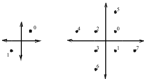
Figure 8: Constellation labels for b = 1 and b = 3
