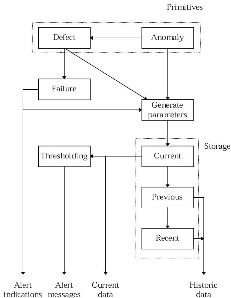
Figure 42: Performance monitoring process
