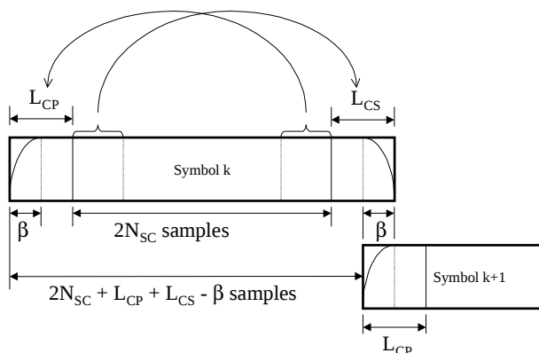
Figure 6: Cyclic extensions, windowing and overlap of DMT symbols
