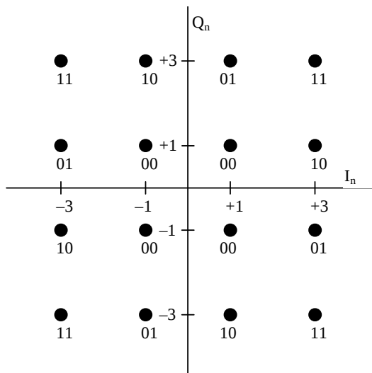
Figure 18: 16-point Constellation and Bit Mapping
