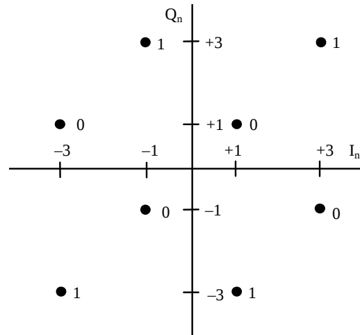
Figure 17: 8-point Constellation and Bit Mapping
