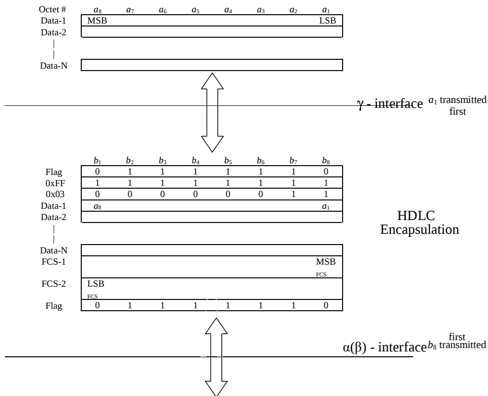
Figure 31: PTM-TC data flow
