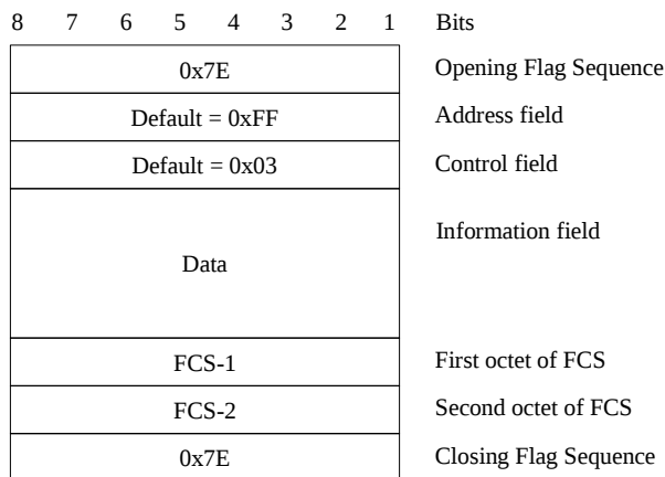
Figure 30: PTM-TC frame format
