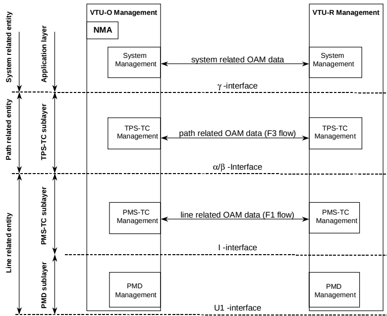
Figure 44: OAM Functional Model
