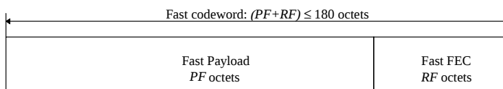
Figure 37: Structure of Fast Codeword
