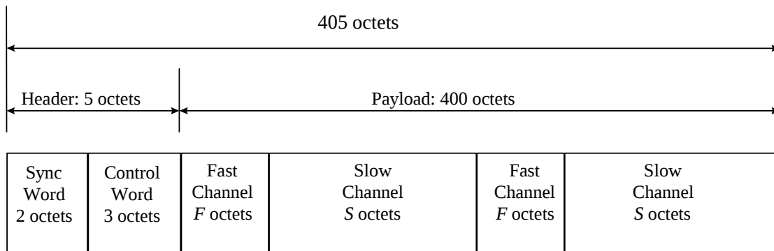
Figure 36: Transmission Frame Format
