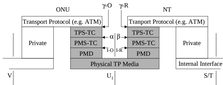
Figure 2: VDSL protocol layer model
