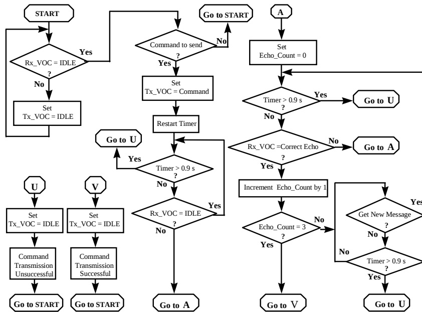
Figure 46: VTU-O Handshaking Flow Chart
