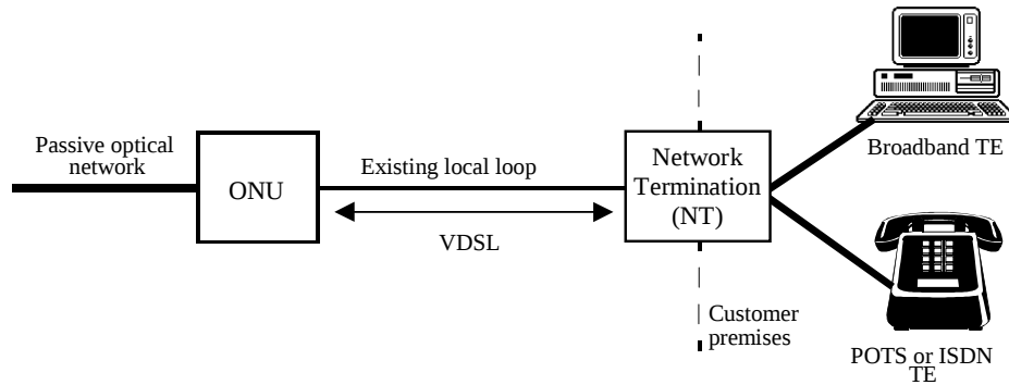
Figure 4: General fibre-to-the-node architecture for VDSL
