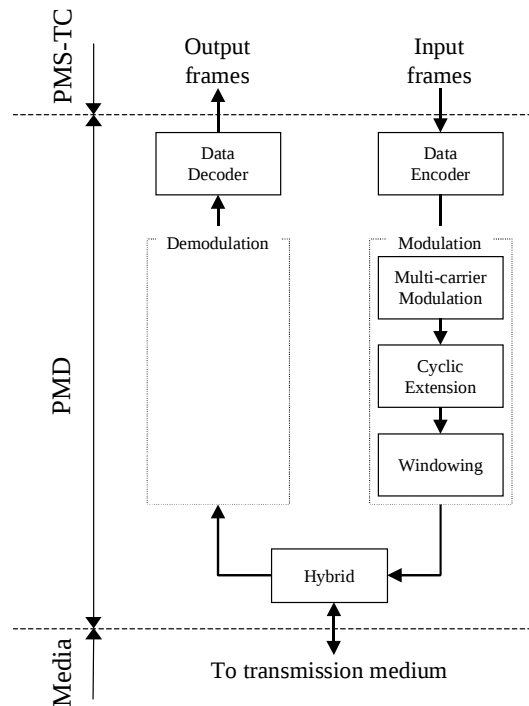
Figure 5: Functional model of PMD Sub-layer
