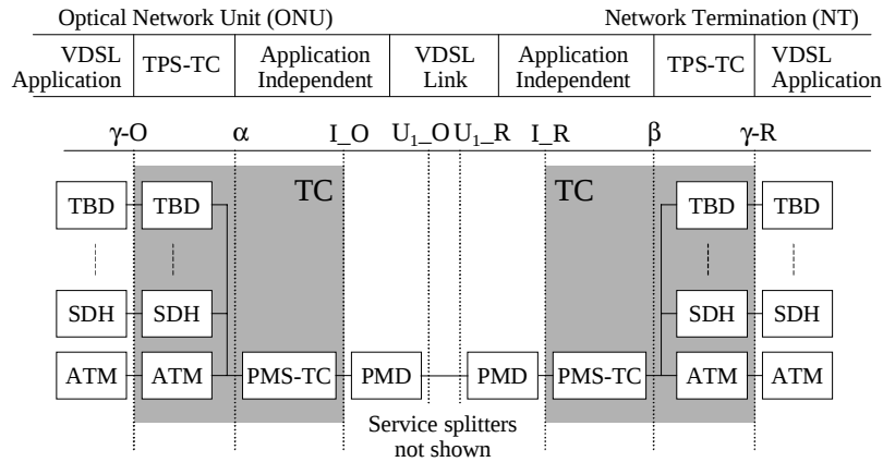
Figure 3: Functional decomposition
