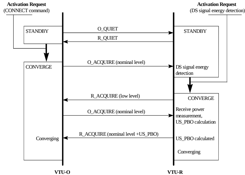
Figure 62: Activation From the VTU-O
