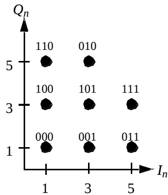
Figure 17: 8-point Constellation and Bit Mapping
