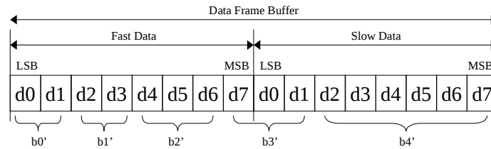
Figure 10: Bit extraction after tone ordering
