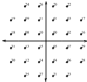
Figure 9: Constellation labels for b = 5
