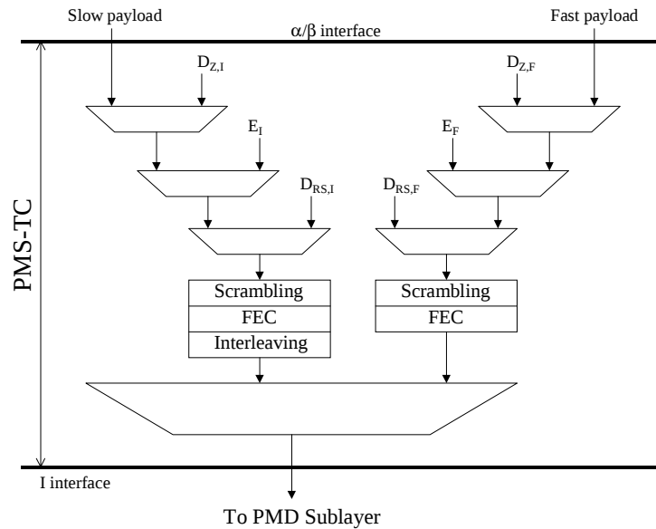
Figure 33: PMS-TC block diagram
