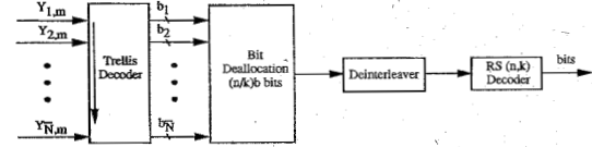
Fig. 3. Coded DMT receiver.
