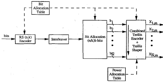
Fig. 9. Coded and shaped multicarrier encoder.
