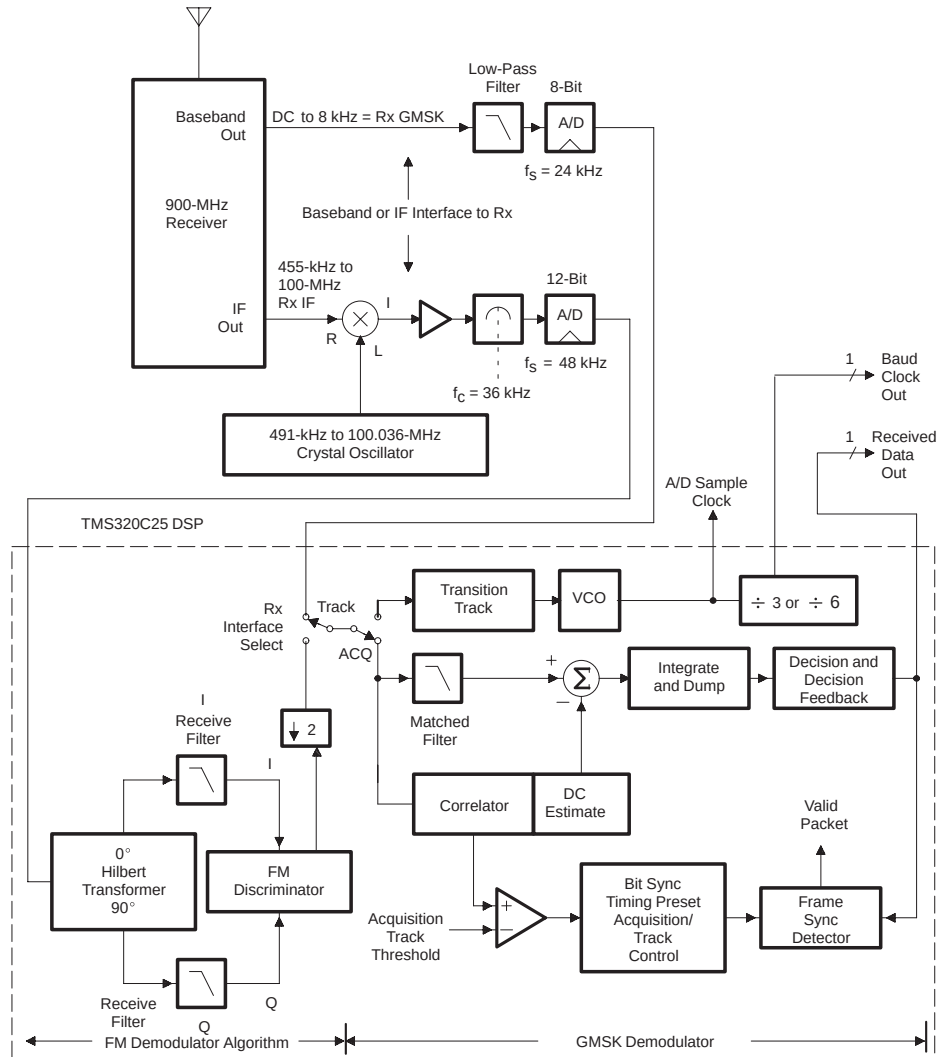
Figure 6. GMSK Demodulator DSP Implementation
