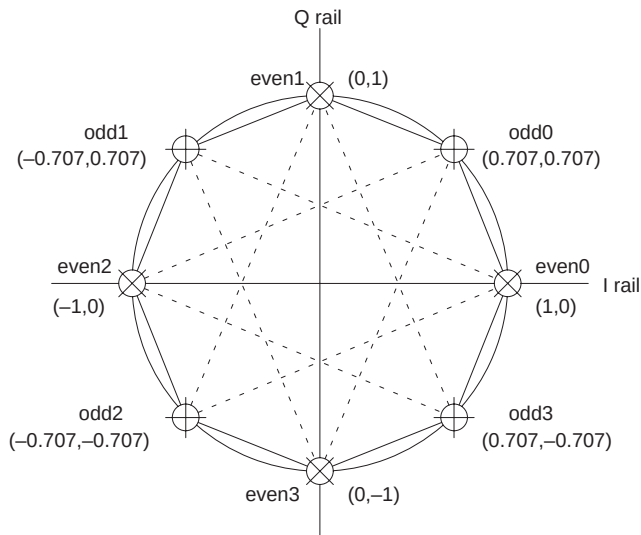
Figure 1. \pi/4 -Shifted QPSK Signal Constellation
