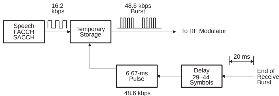
Figure 10. Burst Generator
