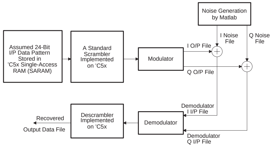
Figure 5. Modem Test Configuration
