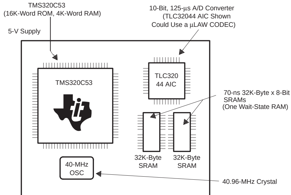
Figure 2. A Minimal TMS320C53 HMM System
