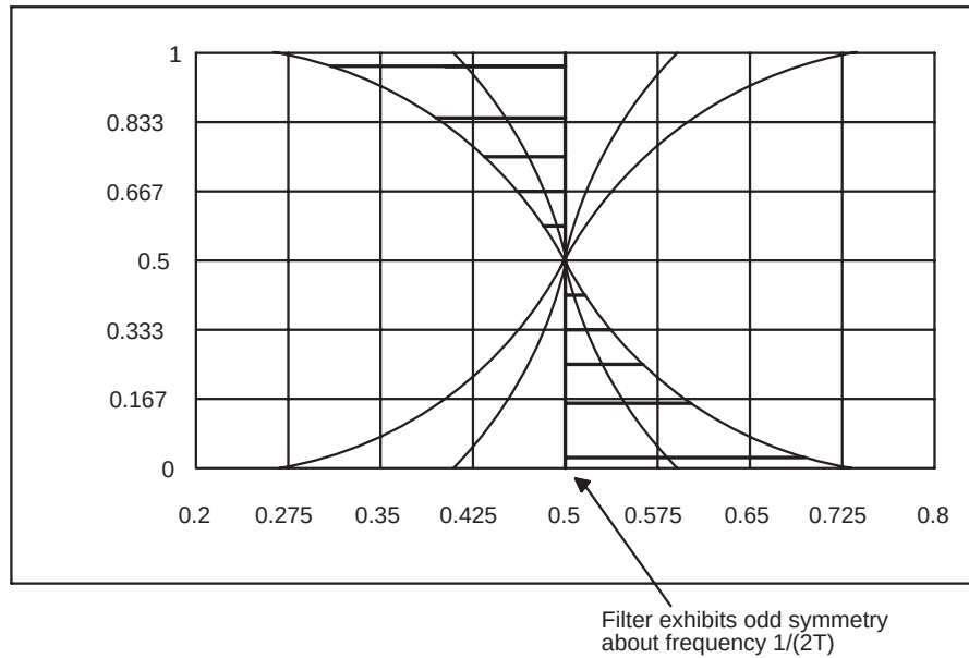
Figure 6. Odd Symmetry
