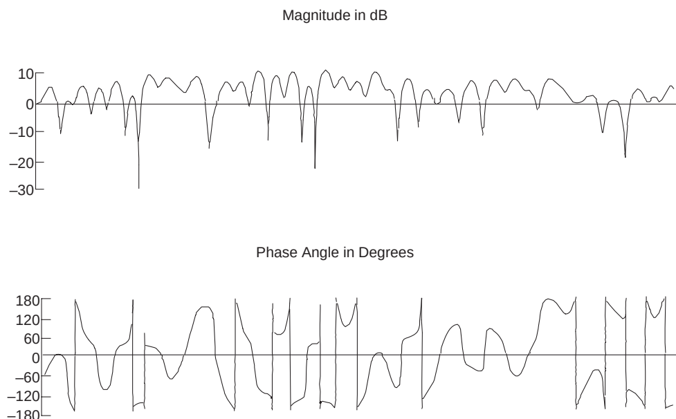
Figure 3. Rayleigh Fading
