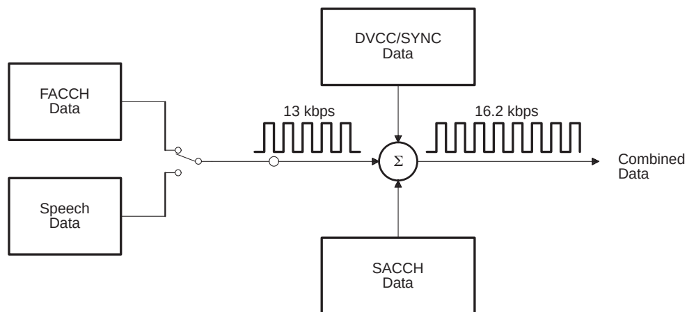
Figure 9. Control-Signal Multiplexing
