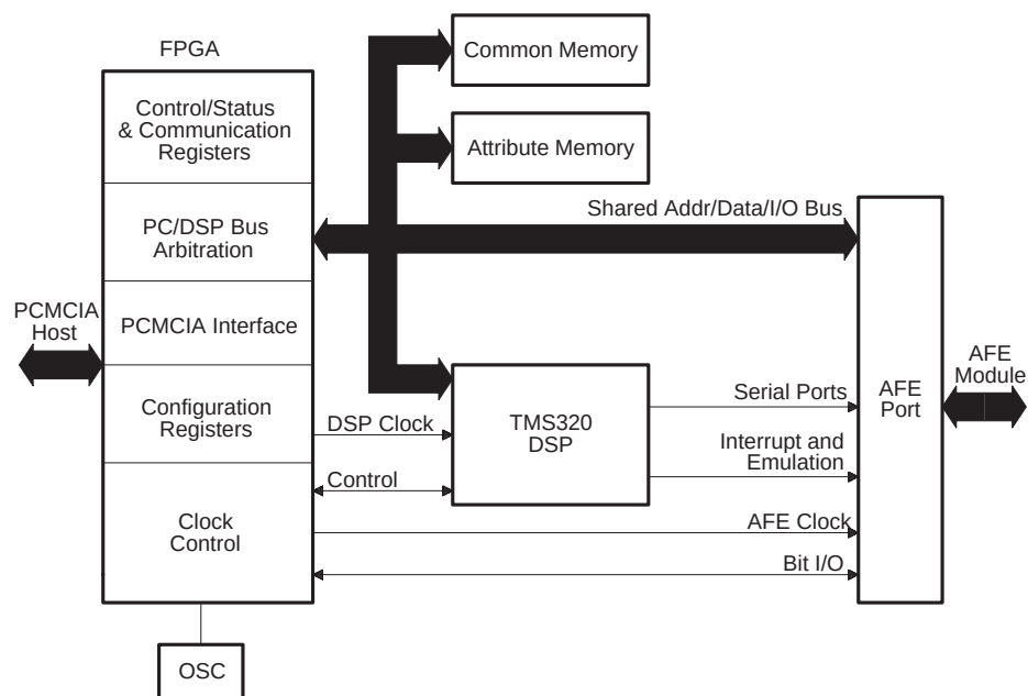
Figure 2. DSP Card Architecture
