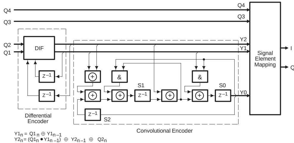
Figure 2. V.32 Encoder
