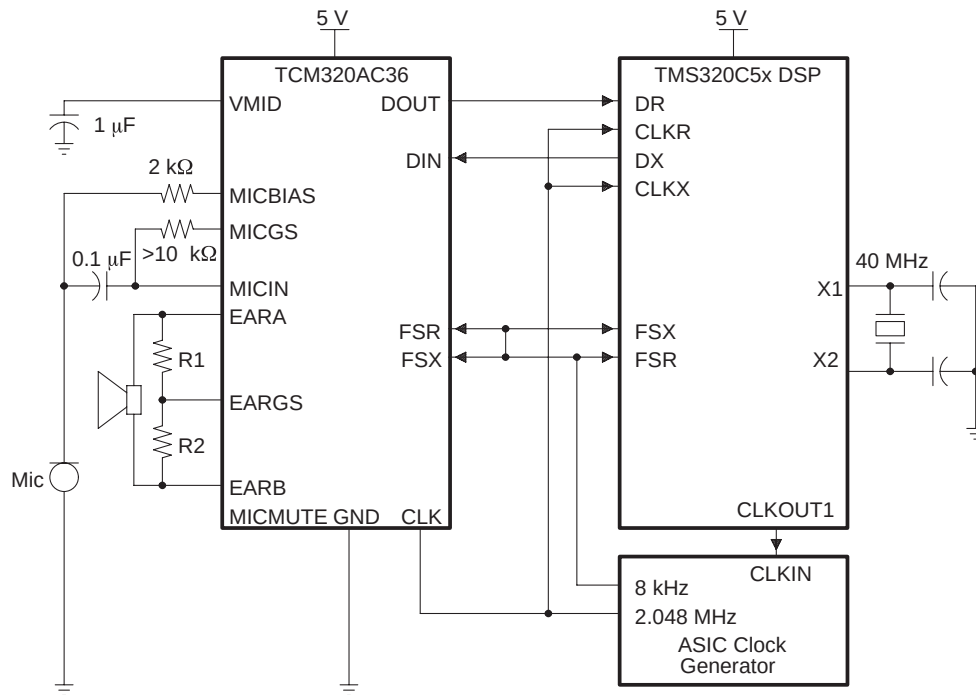
Figure 3. VBAP Interfaced to a 'C5x DSP
