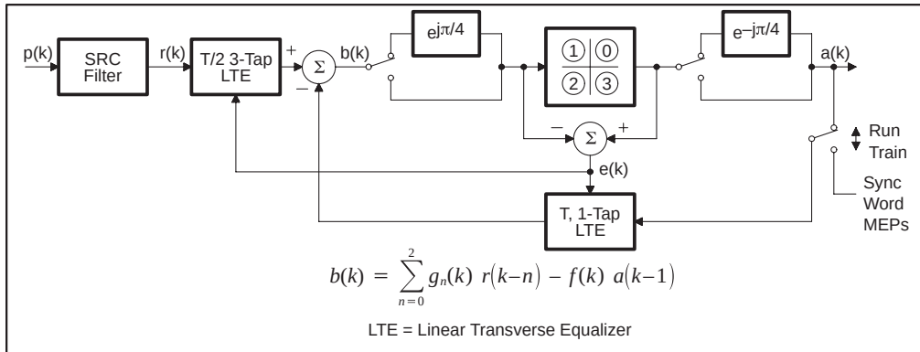
Figure 5. Block Diagram of a Decision-Feedback Equalizer
