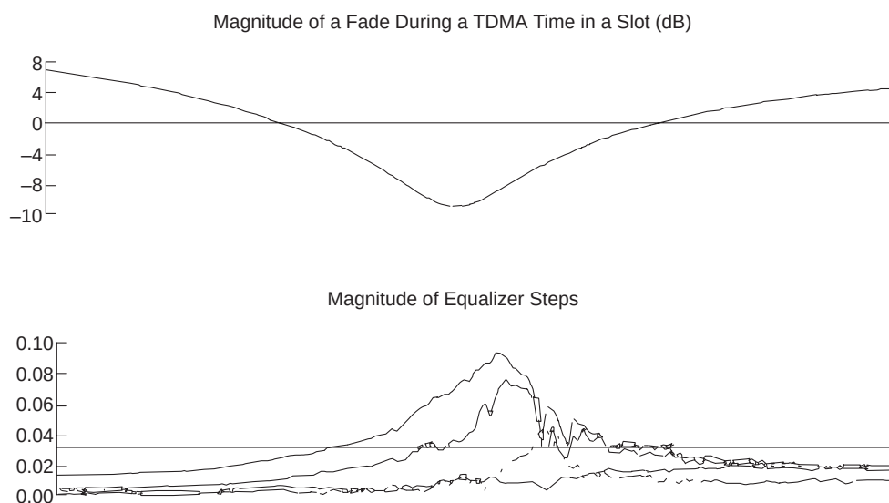
Figure 6. Equalizer Taps Responding to a Fade
