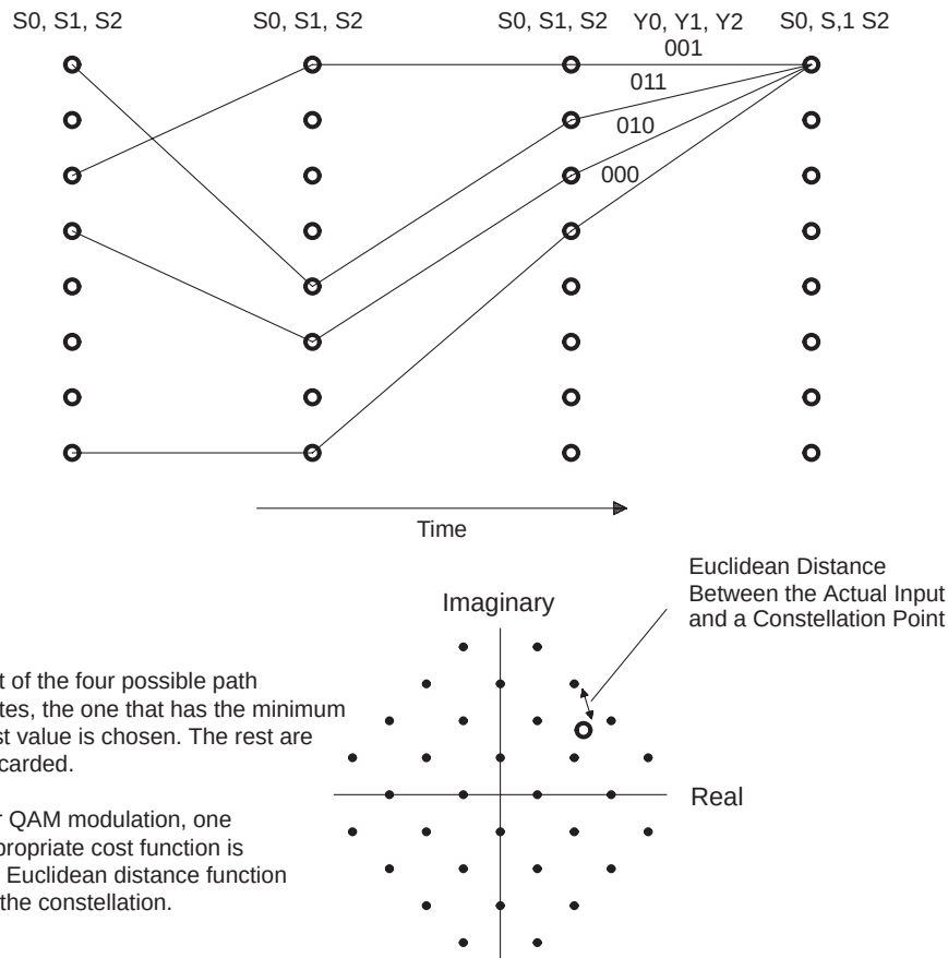
Figure 5. Viterbi Decoding — Output Tracking and Cost Function
