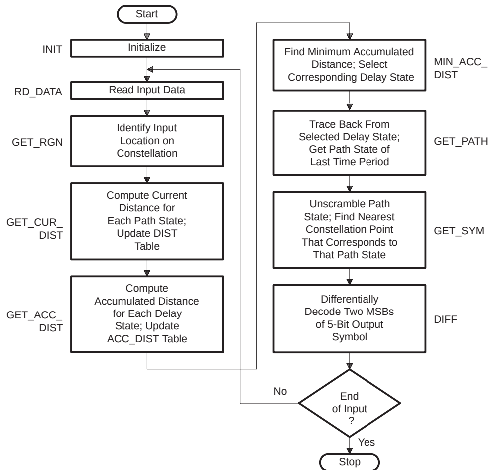
Figure 9. Decoder Flowchart
