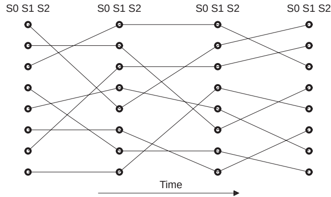
Figure 7. Viterbi Decoding — Dynamic Programming
