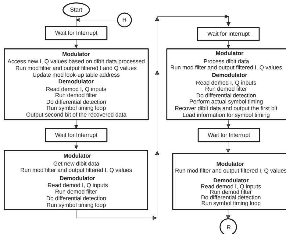
Figure 4. Interrupt Organization
