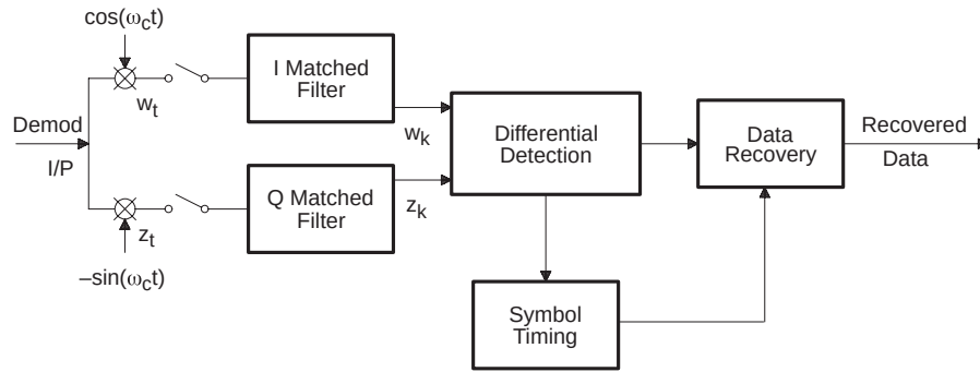
Figure 3. Demodulator Block Diagram
