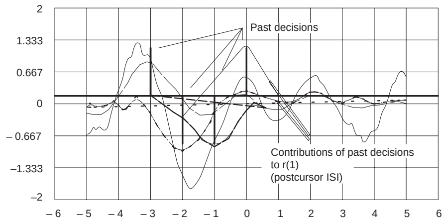
Figure 17. Received Signal Including Additive Noise Effects
