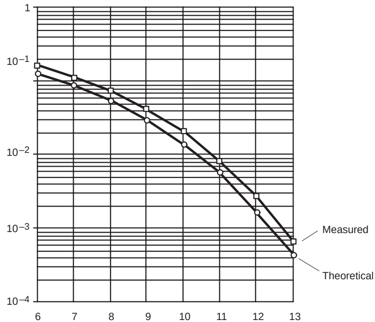
Figure 2. Bit Error Rate Versus E_b/N_0 Modem Performance
