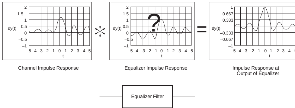
Figure 12. Equalization Process
