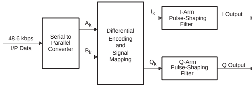
Figure 2. Modulator Block Diagram
