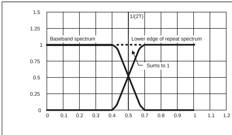
Figure 7. Spectral Response at 1/(2T)
