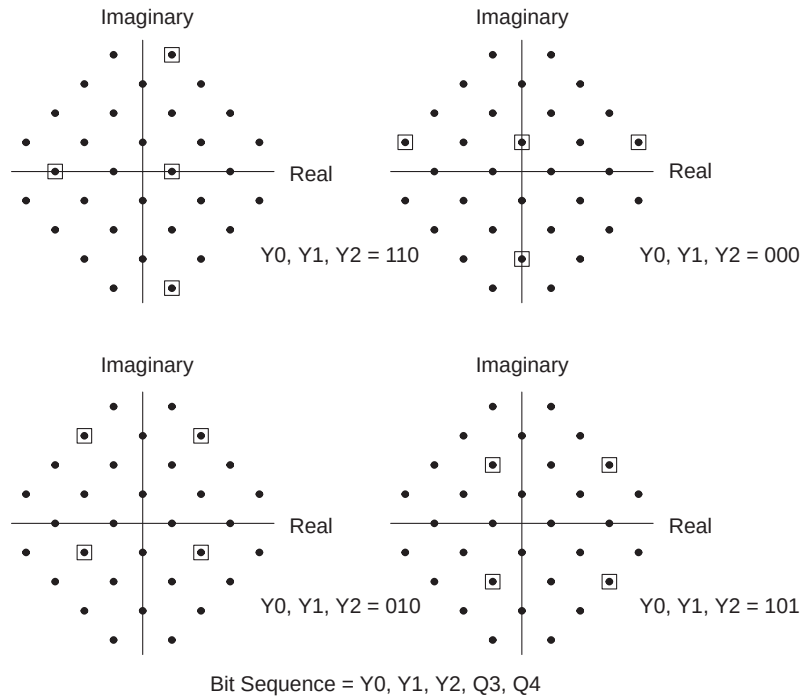
Figure 6. V.32 Modem — Signal Element Mapping
