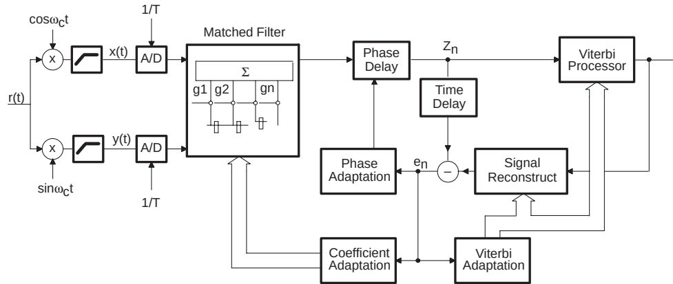
Figure 16. An MLSE Adaptive Equalizer
