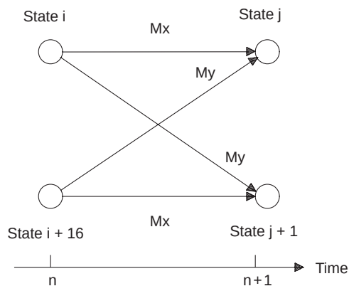
Figure 4. Representative Trellis Section for VSELP Convolutional Encoder
