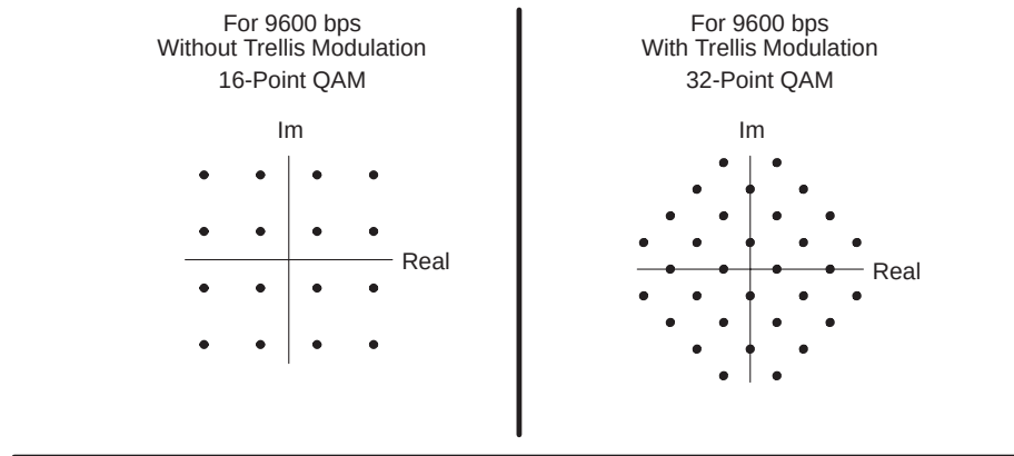
(b) V.32 Modems Constellation Regions
