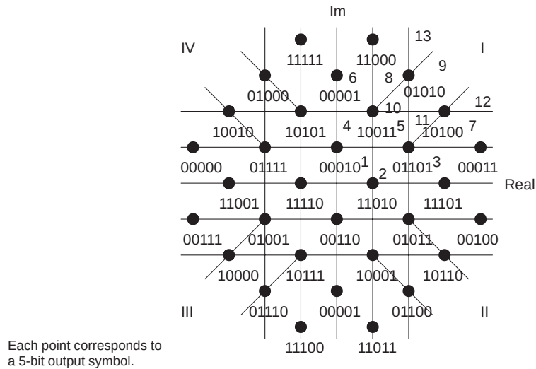
(b) V.32 Modems Constellation Regions
