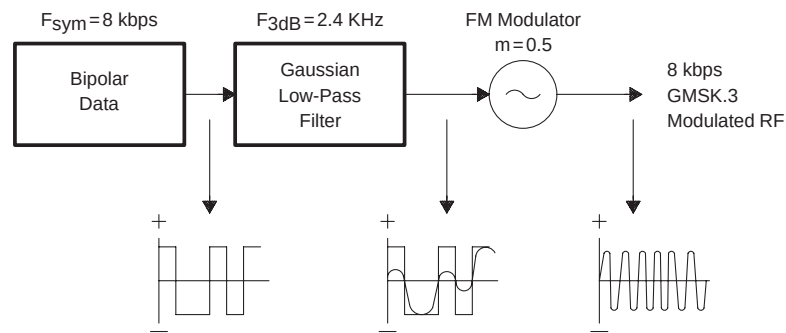
Figure 3. Idealized GSMK.3 Generation
