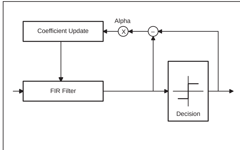
Figure 16. Decision-Directed Equalization
