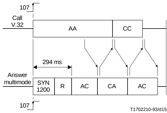
FIGURE I.5/V.32
