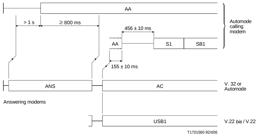
FIGURE A.1/V.32
