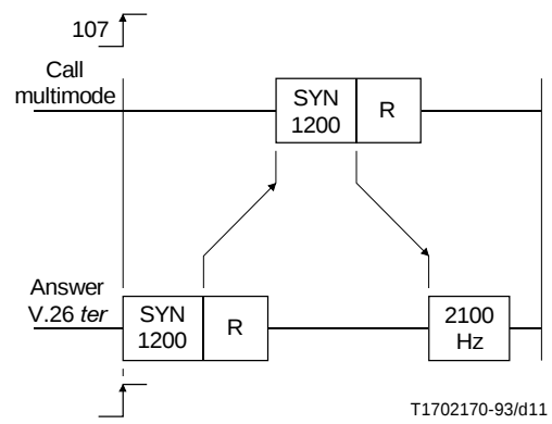
FIGURE I.1/V.32
