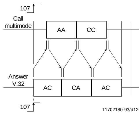
FIGURE I.2/V.32
