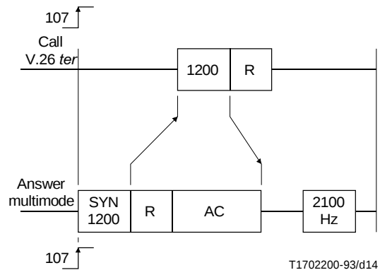
FIGURE I.4/V.32
