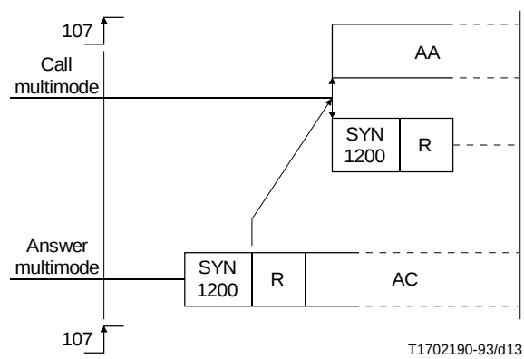
FIGURE I.3/V.32
