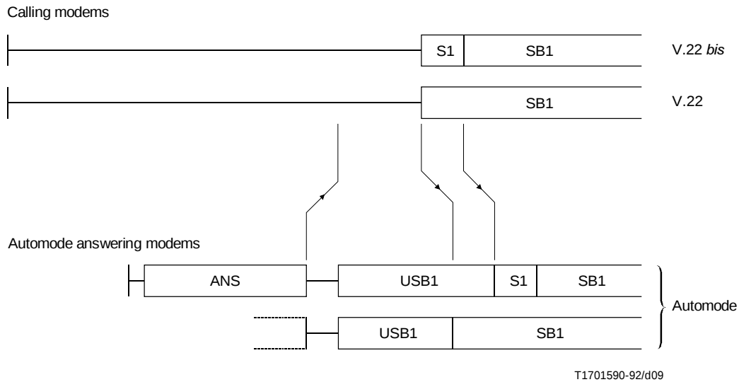
FIGURE A.4/V.32 Answering automode modem interworking with a calling V.22 bis or V.22 modem
