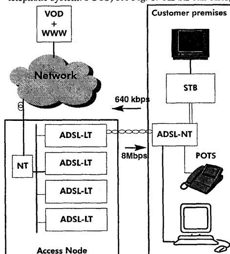
Fig. 1: ADSL network.
