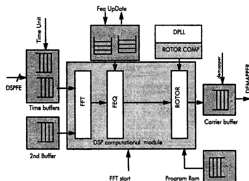
Fig. 5: Receive FFT.
