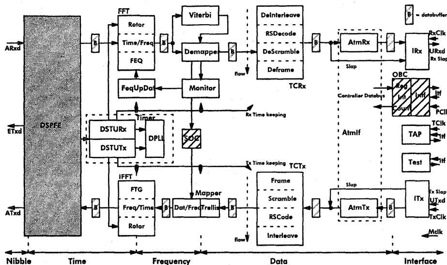
Fig. 3: SACHEM architecture.
