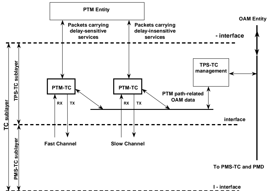
Figure 28: Functional model of PTM transport
