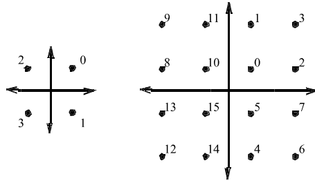
Figure 7: Constellation labels for b = 2 and b = 4
