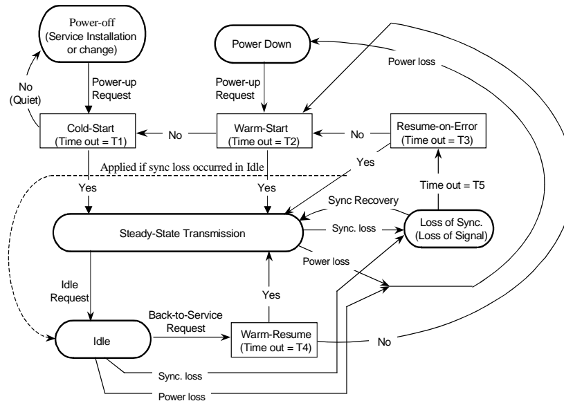
Figure 57: Link State and Timing Diagram
