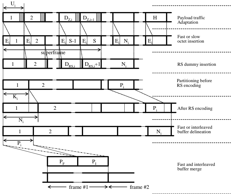
Figure 34: Framing description
