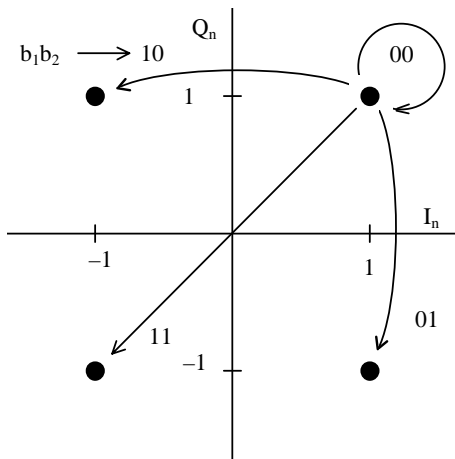
Figure 16: 4-point Constellation with Differential Bit Encoding
