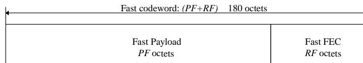
Figure 37: Structure of Fast Codeword
