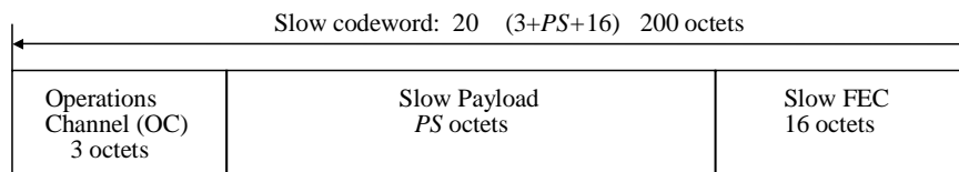
Figure 38: Structure of Slow Codeword
