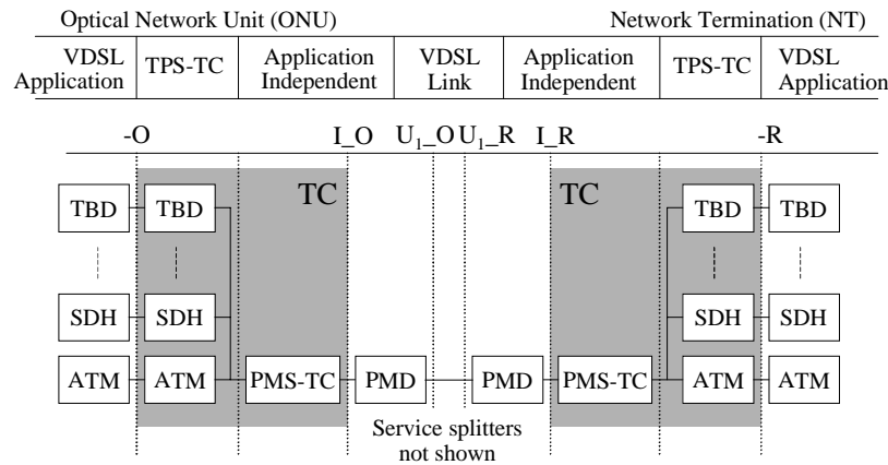
Figure 3: Functional decomposition
