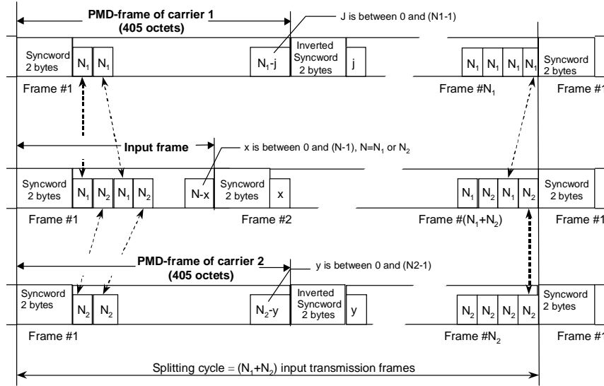
Figure 12: PMD-frame Format
