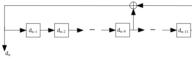
Figure 54: Pseudo-random bit generator
