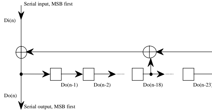
Figure 40: Randomiser
