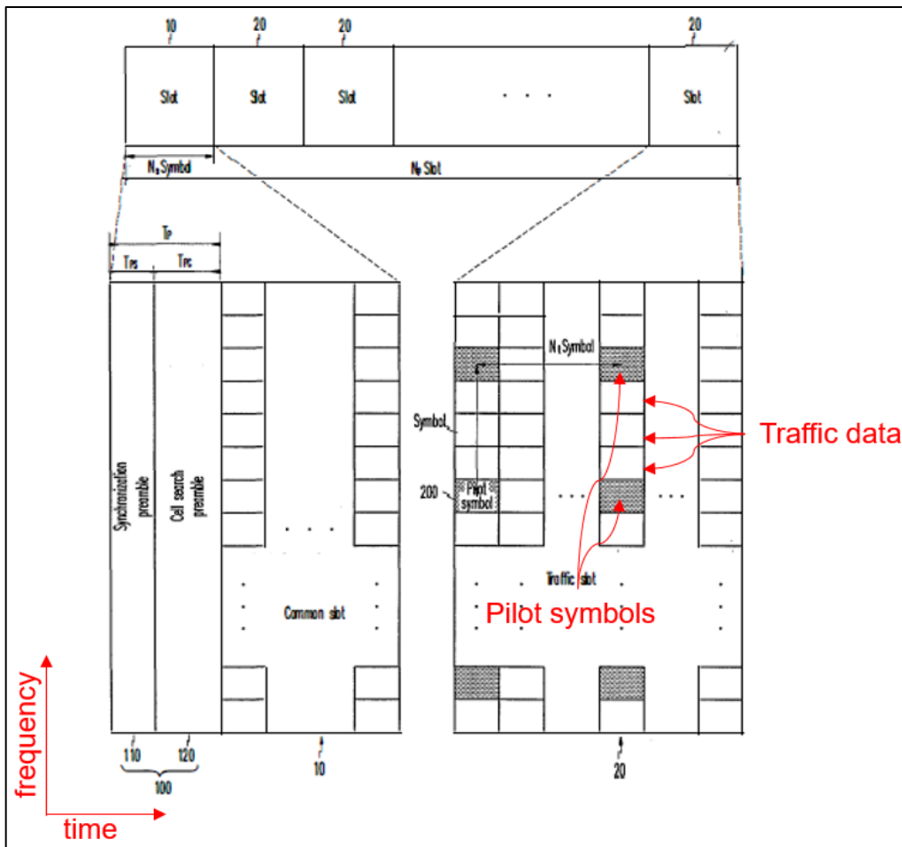
EX1004, FIG. 1 (annotated).
