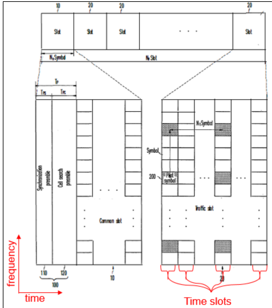
EX1004, FIG. 1 (annotated).
