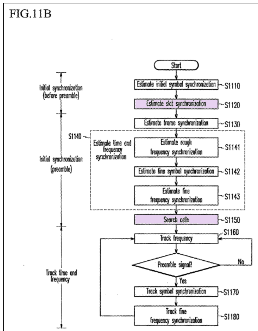
EX1004, FIG. 11B (annotated).
