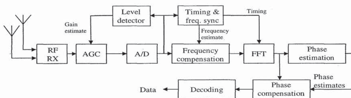
Figure 10.5 OFDM receiver.
