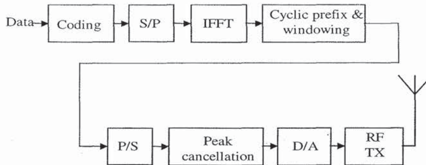
Figure 6.15 OFDM transmitter with peak cancellation.
