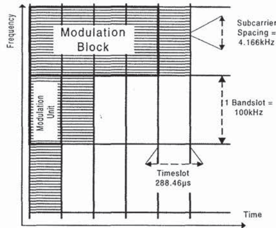
Figure 9.4 Time-frequency grid.
