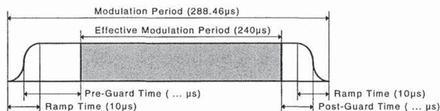
Figure 9.6 OFDM modulation burst.
