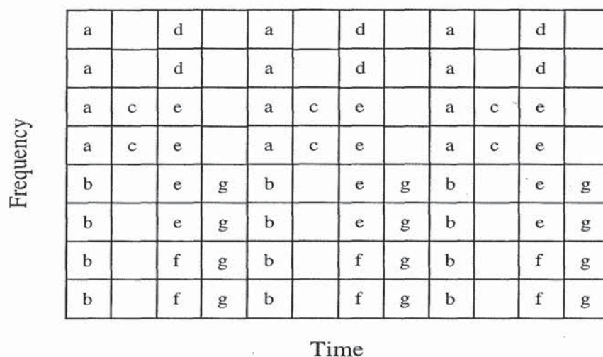
Figure 9.1 Example of the time-frequency grid with seven OFDMA users, a to g, which all have a fixed set of subcarriers every four timeslots.
