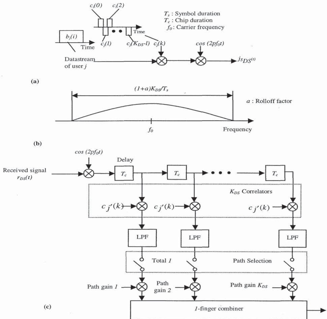
Figure 8.2 DS-CDMA system: (a) transmitter, (b) power spectrum of its transmitted signal, and (c) RAKE receiver.
