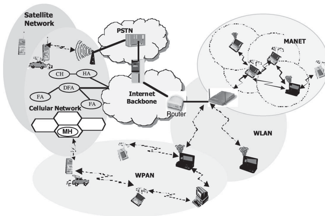
Fig. 1. 4G networks.
