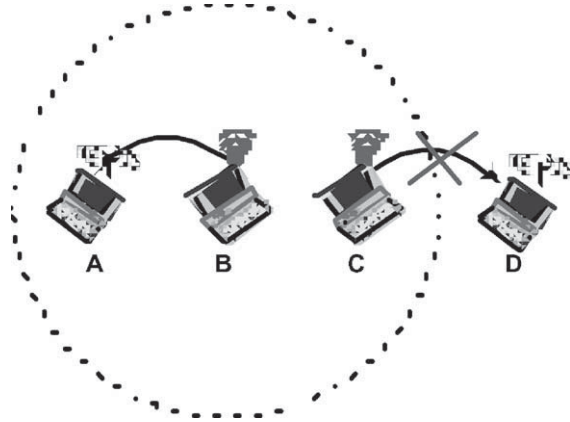
Fig. 5. Exposed-station problem.
