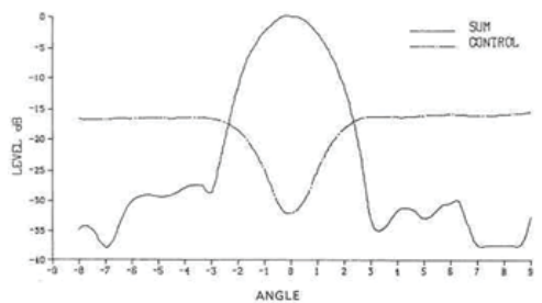
Normal Antenna Patterns
