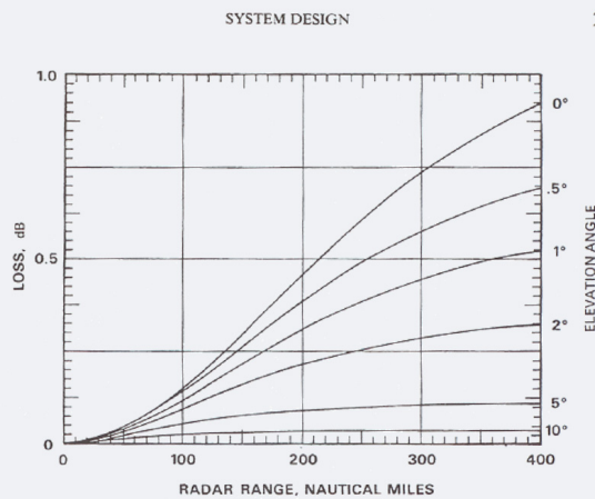
Fig. 10.4 Lens loss for various signal elevation angles (from ref. 10.1).
