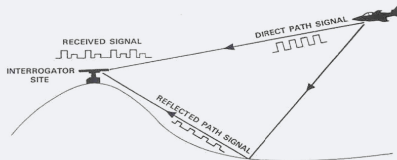
Fig. 7.10 Geometry of direct and reflected reply paths.
