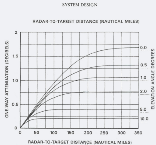
Fig. 10.2 Atmospheric absorption versus range for various signal elevation angles
