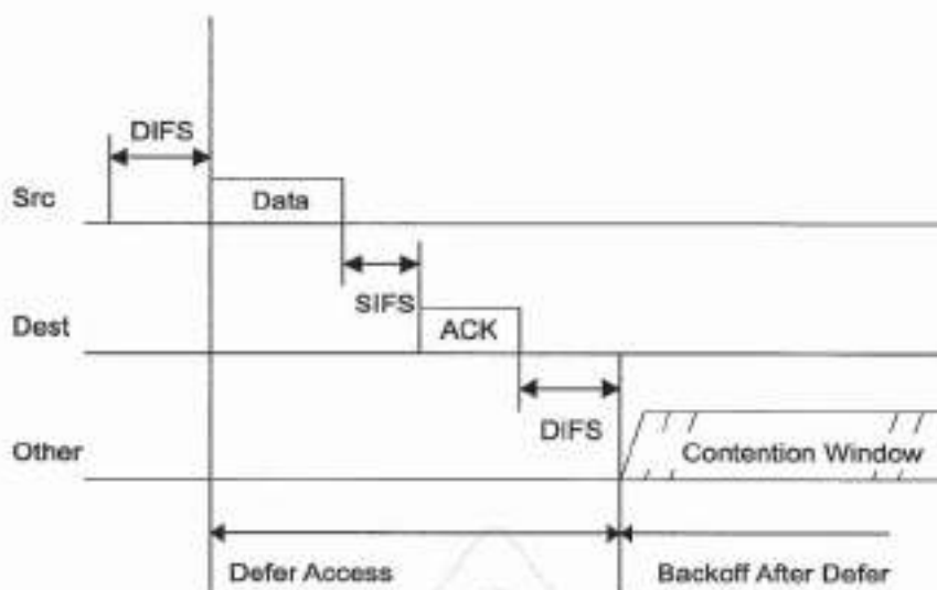
Figure 57—Directed data/ACK MPDU
