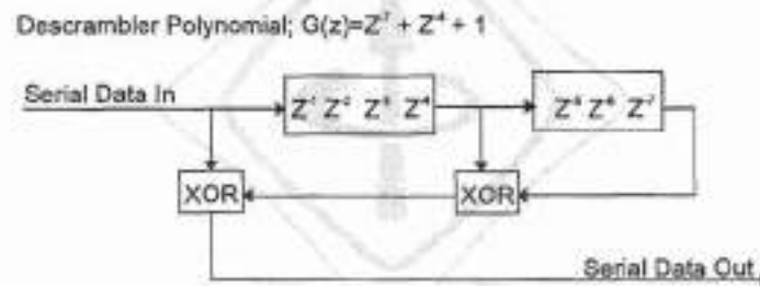
Figure 90—Data descrambler
