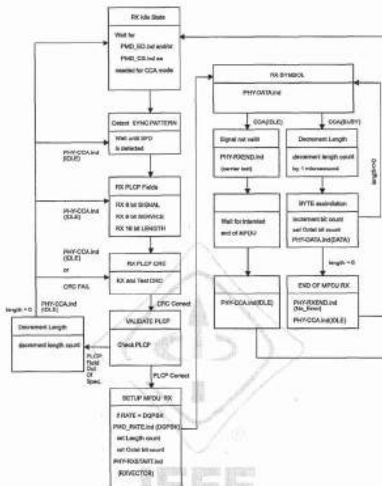
Figure 94—PLCP receive state machine
