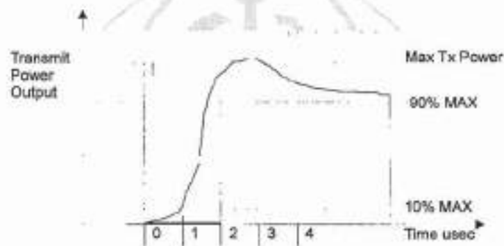
Figure 96—Transmit power-on ramp
