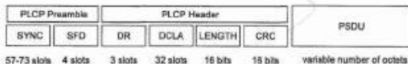
Figure 101—PLCPDU frame format
