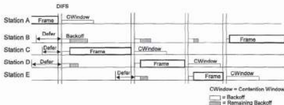
Figure 52—Backoff procedure
