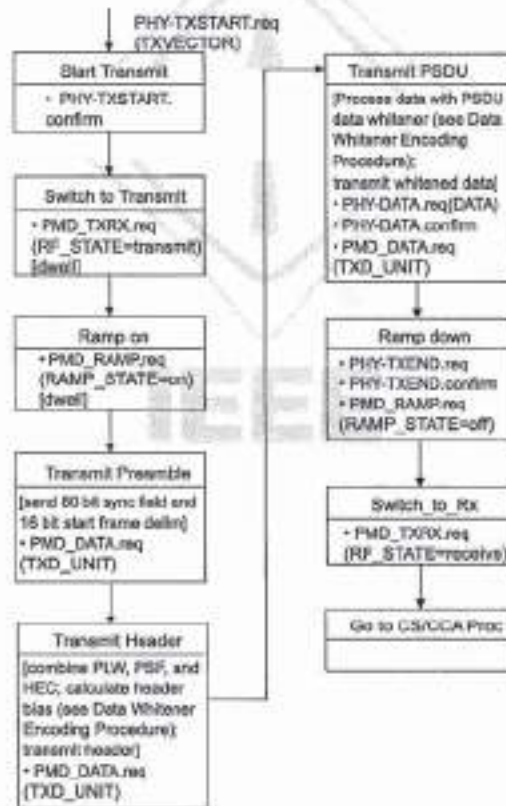
Figure 74—Transmit state machine
