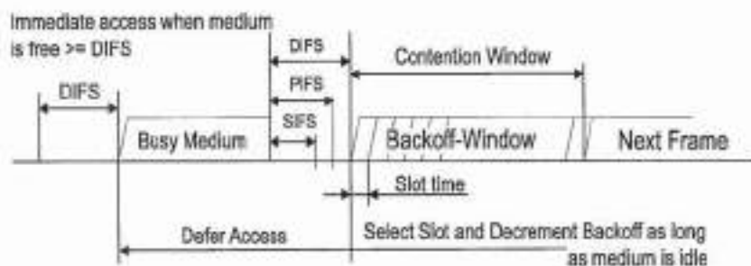
Figure 51—Basic access method
