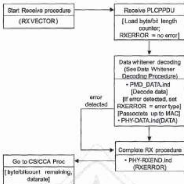
Figure 79—Receive state machine
