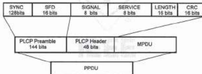
Figure 86—PLCP frame format
