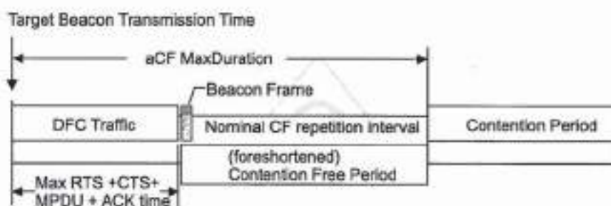
Figure 61—Example of delayed beacon and foreshortened CFP
