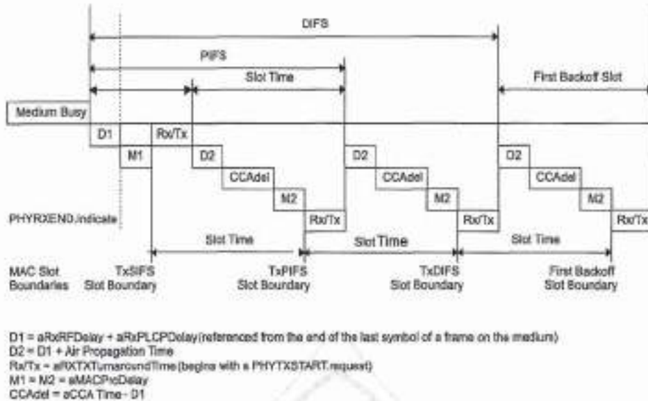
Figure 58—DCF timing relationships
