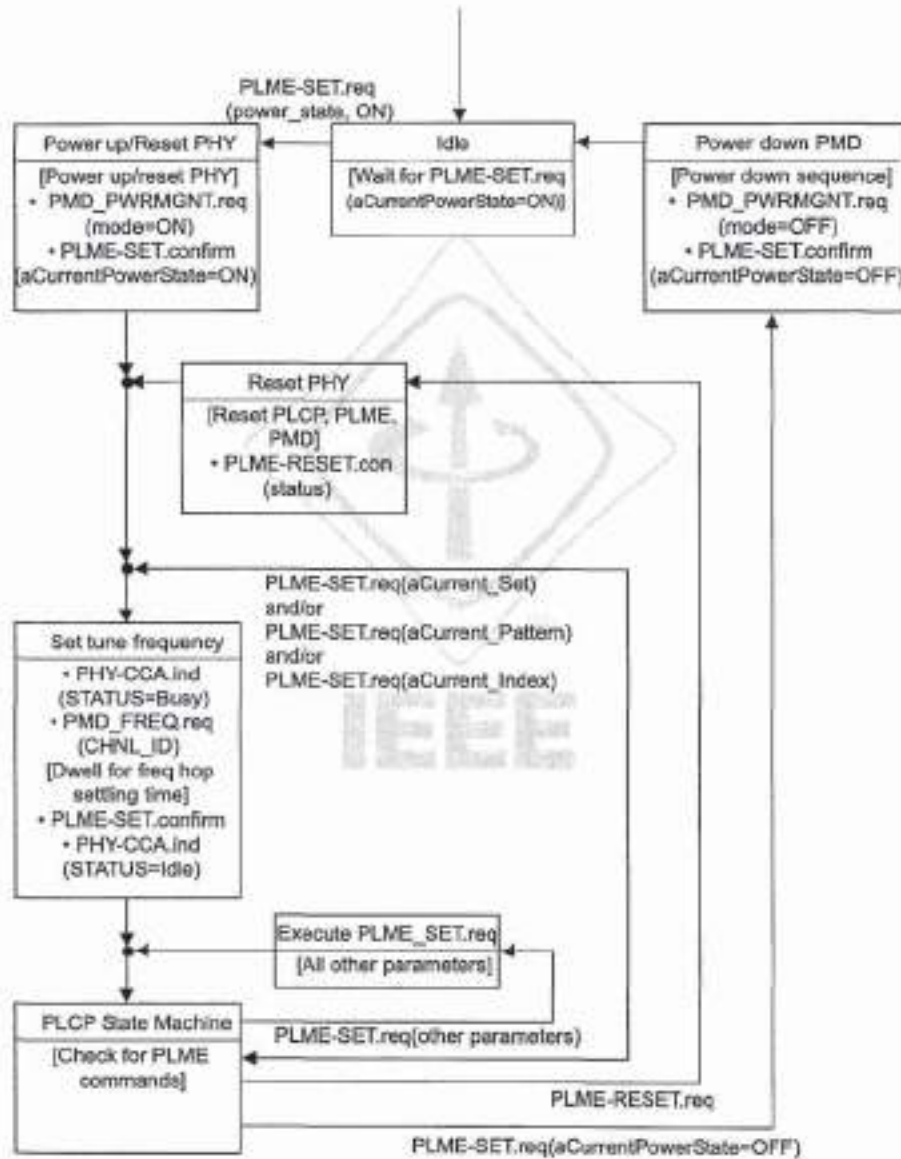
Figure 82—PLME state machine
