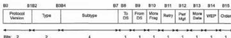
Figure 13—Frame Control field
