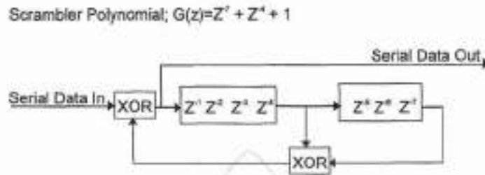
Figure 89—Data scrambler
