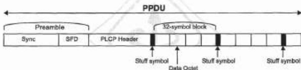
Figure 72—PLCP data whitener format
