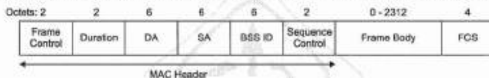
Figure 23—Management frame format
