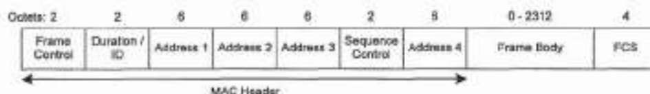
Figure 22—Data frame
