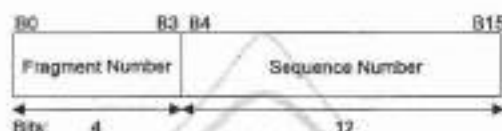
Figure 14—Sequence Control field
