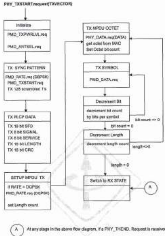
Figure 92—PLCP transmit state machine
