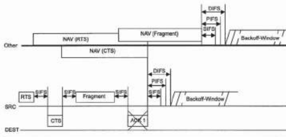
Figure 56—RTS/CTS with transmitter priority and missed acknowledgment
