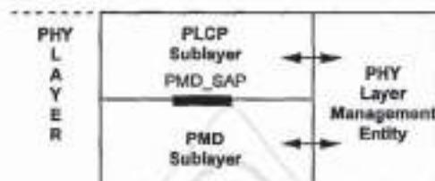
Figure 83—PMD layer reference model
