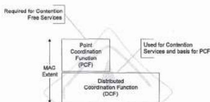
Figure 47—MAC architecture
