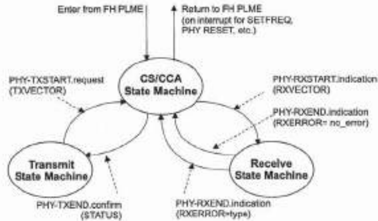
Figure 73—PLCP top-level state diagram
