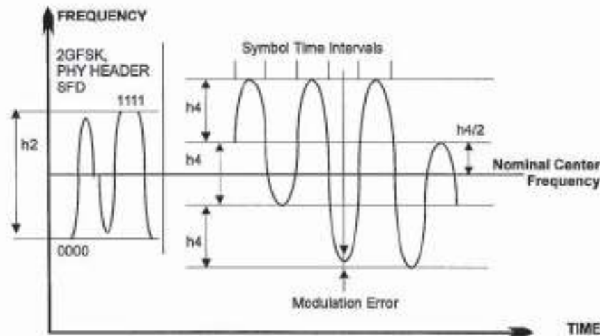
Figure 85—Four-Level QFSK transmit modulation
