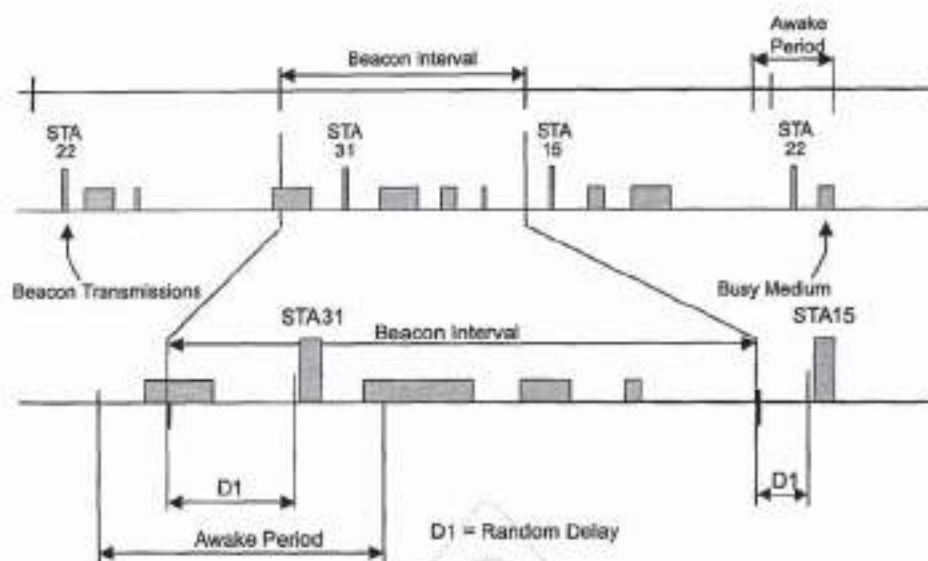
Figure 65—Beacon transmission in an IBSS
