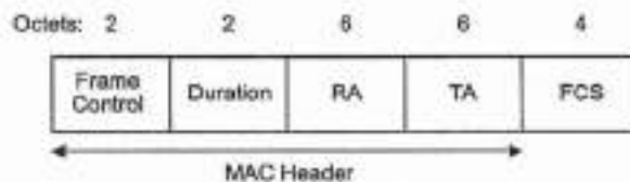
Figure 16—RTS frame
