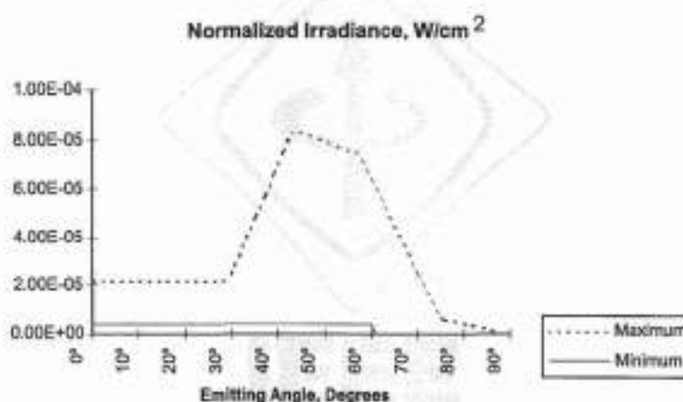
Figure 103—Emitter radiation pattern mask 1
