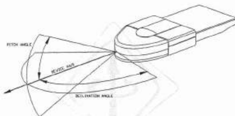
Figure 104—Mask 2 device orientation drawing
