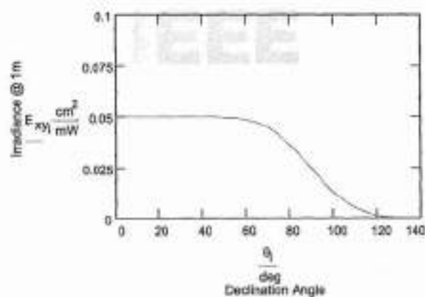
Figure 105—Emitter radiation pattern mask 2
