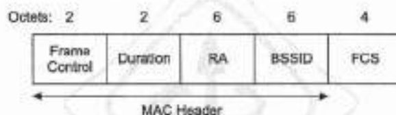
Figure 20—CF-End frame
