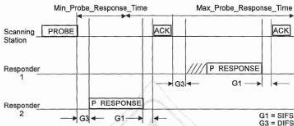
Figure 66—Probe response
