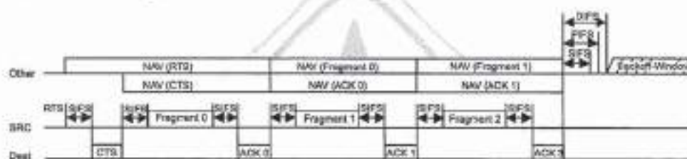
Figure 55—RTS/CTS with fragmented MSDU
