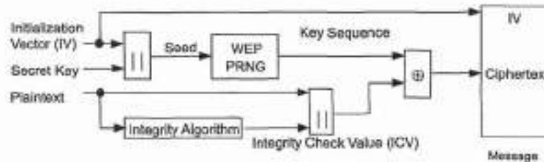
Figure 44—WEP encipherment block diagram
