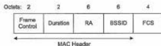
Figure 21—CF-End + CF-Ack Frame
