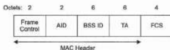
Figure 19—PS-Poll frame
