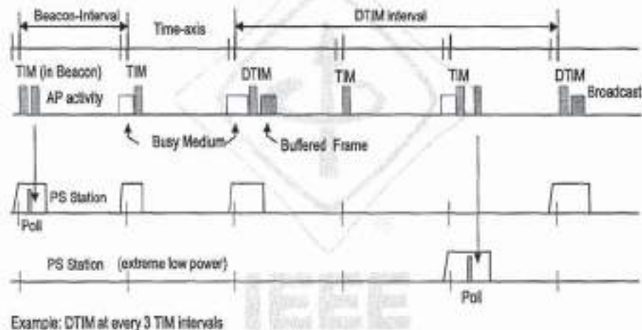
Figure 67—Infrastructure power management operation (no PCF operating)
