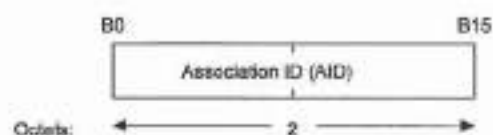
Figure 31—AID fixed field
