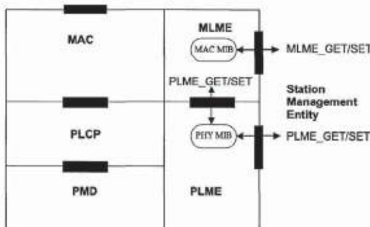
Figure 63—GET and SET operations
