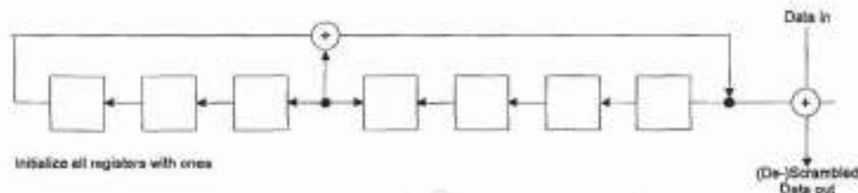
Figure 71—Frame synchronous scrambler/descrambler
