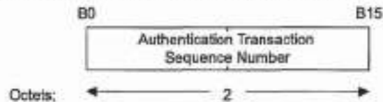
Figure 25—Authentication Transaction Sequence Number fixed field
