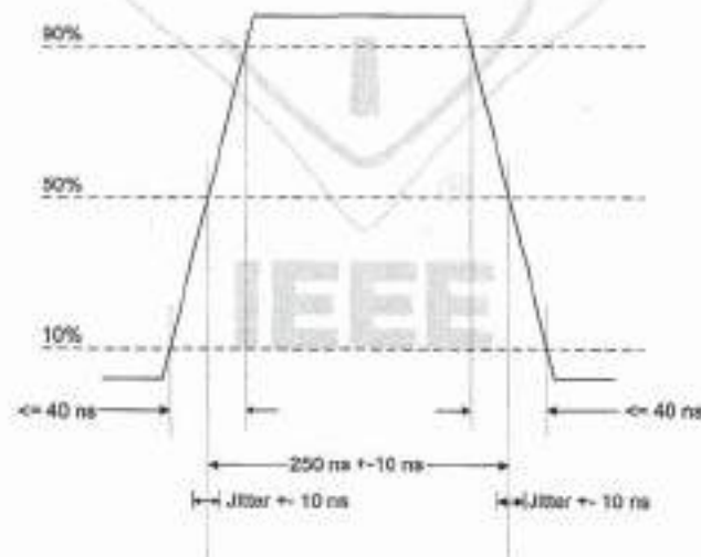
Figure 102—Basic pulse shape
