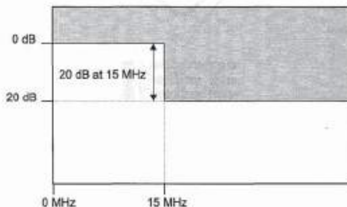
Figure 106—Transmit spectrum mask
