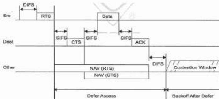
Figure 53—RTS/CTS/data/ACK and NAV setting
