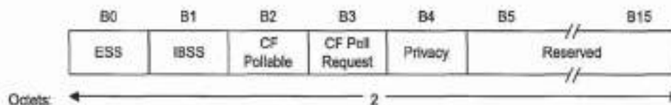
Figure 27—Capability Information fixed field
