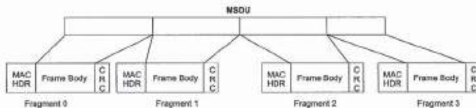
Figure 48—Fragmentation
