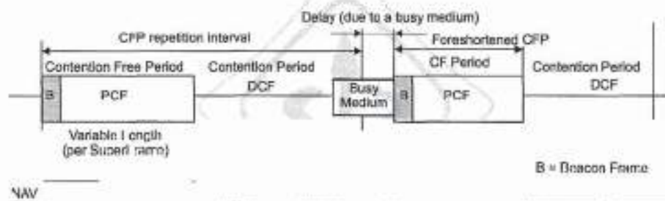
Figure 59—CFP/CP alternation
