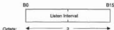
Figure 29—Listen Interval fixed field
