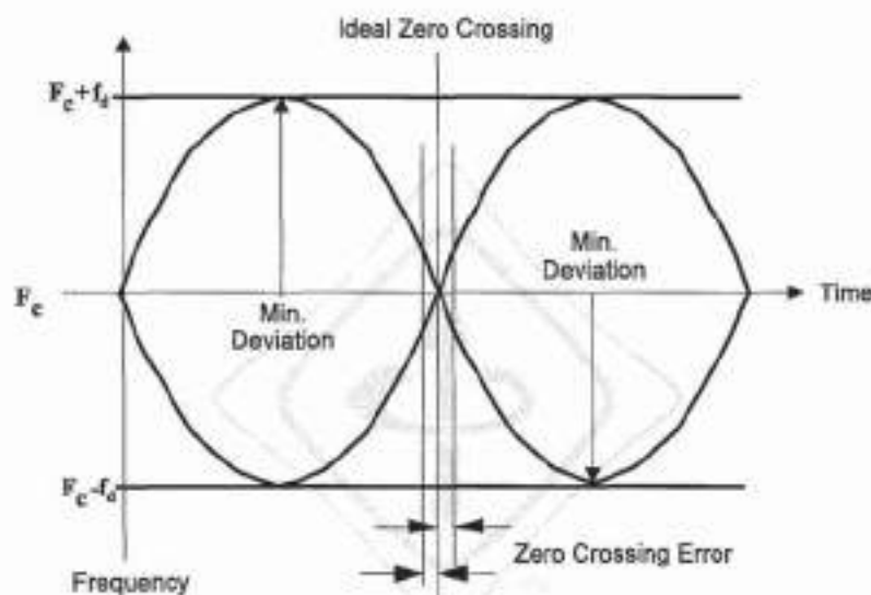
Figure 84—Transmit modulation mask
