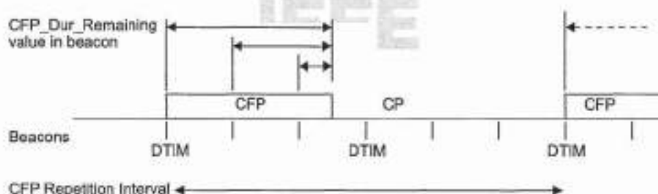
Figure 60—Beacons and CFPs
