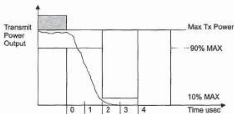
Figure 98—Transmit power-down ramp
