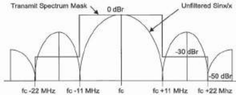
Figure 95—Transmit spectrum mask
