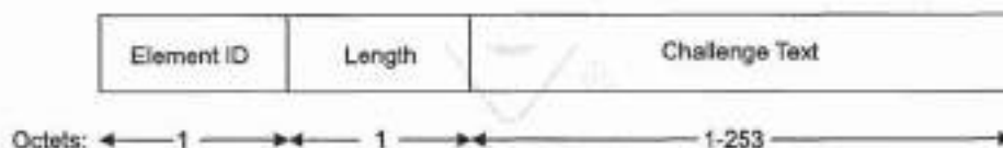
Figure 42—Challenge Text element format
