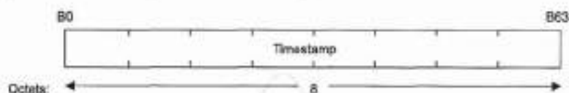
Figure 33—Timestamp fixed field
