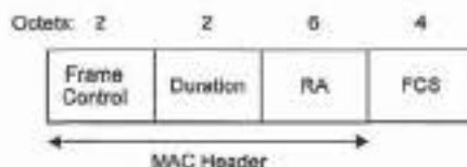
Figure 17—CTS frame
