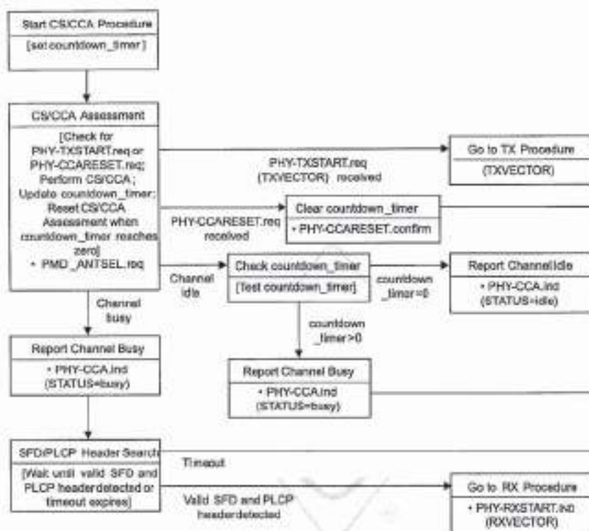
Figure 77—CS/CCA state machine
