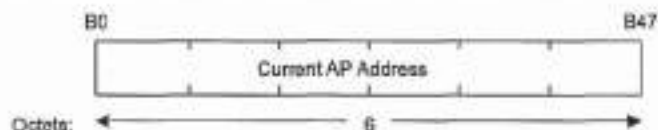
Figure 28—Current AP Address fixed field
