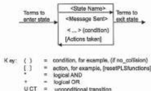
Figure 69—State diagram notation example
