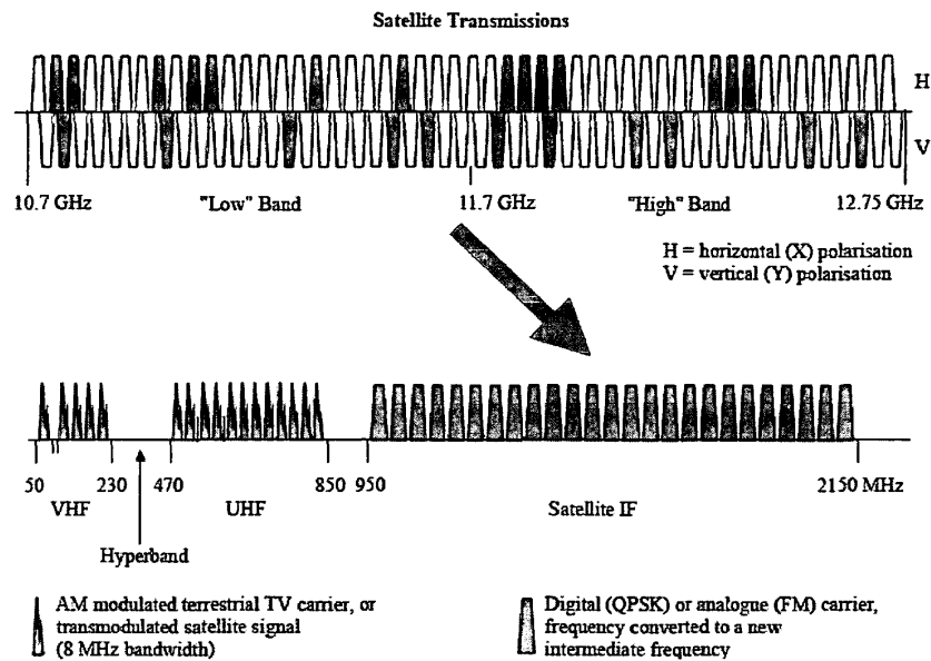
Figure 7 : Broadband Signal Spectrum for an IF-IF Distribution Network
