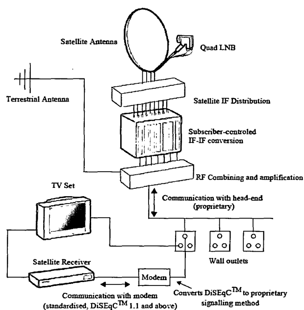
Figure 11 : Architecture of a System with a Remote Controlled Head-End
