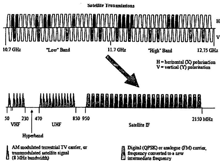
Figure 7 : Broadband Signal Spectrum for an IF-IF Distribution Network
