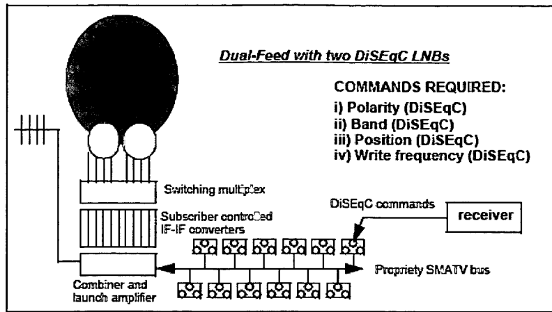
Figure 19: Subscriber controlled SMATV Headend
