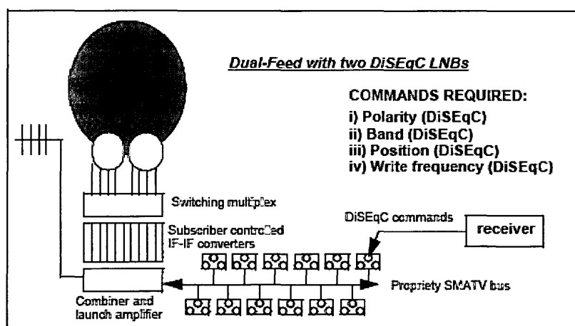
Figure 19: Subscriber controlled SMATV Headend
