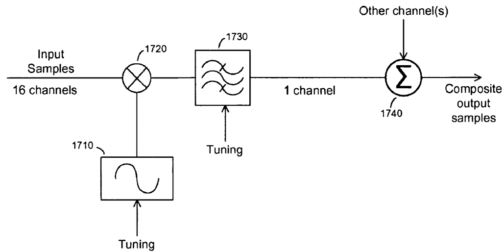
Digital Frequency translator and filter with summer
