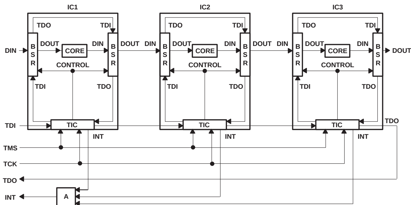
Figure 2. IEEE 1149.1 Architecture
