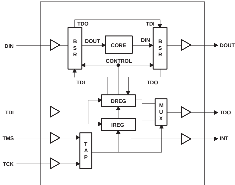
Figure 1. IEEE 1149.1 Architecture
