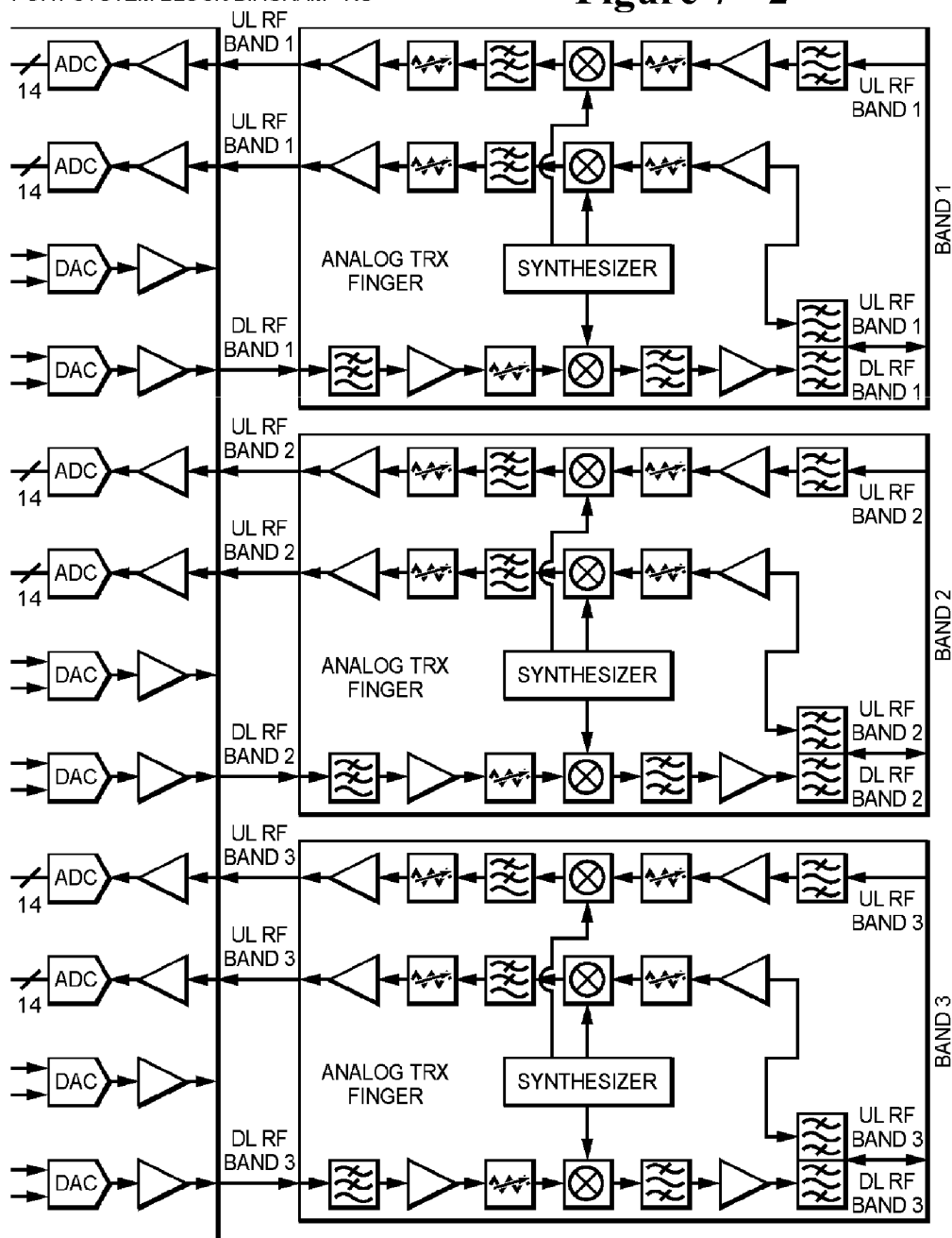
PORT SYSTEM BLOCK DIAGRAM - RU
