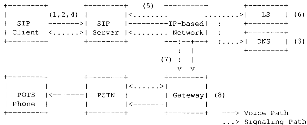
Figure 2 Call from IP-based Network to PSTN
