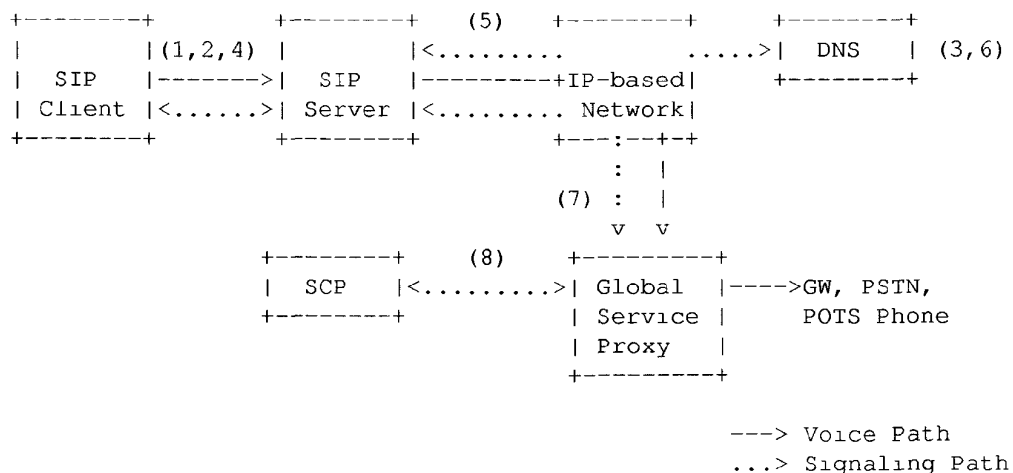
Figure 3 Global Service Call from IP-based Network to PSTN
