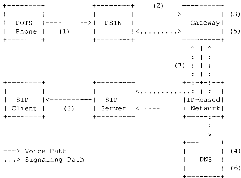
Figure 1 Call From PSTN to IP-based Network
