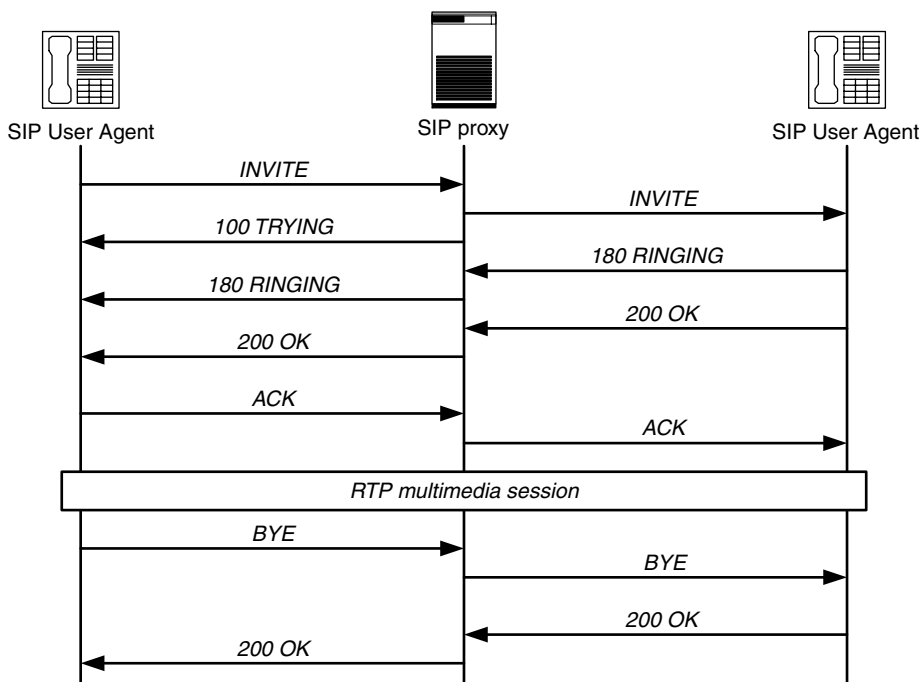
Figure 9.10 SIP call via proxy
