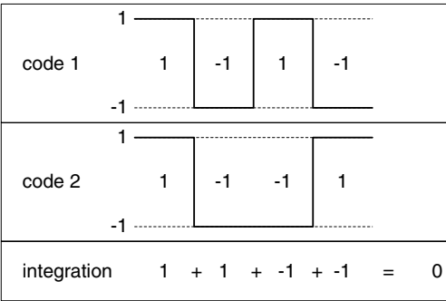
Figure 2.16 CDMA cross-correlation
