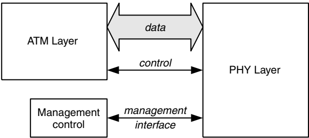
Figure 7.11 UTOPIA model
