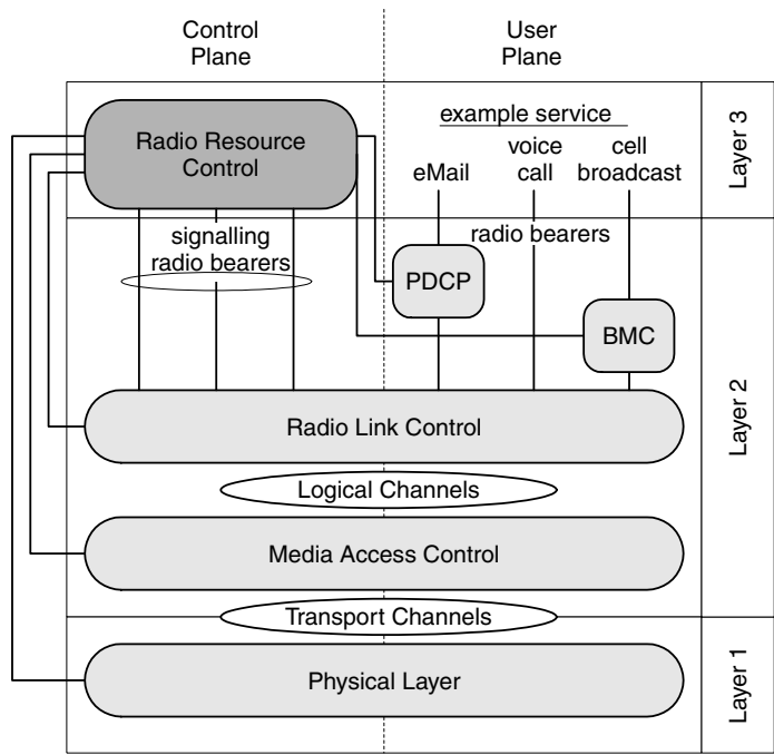
Figure 6.43 Radio interface protocols
