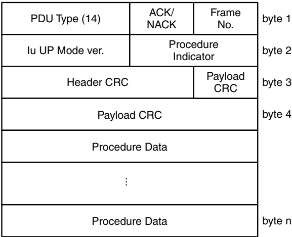
Figure 6.92 Control PDU general format
