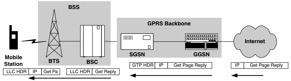
Figure 4.42 IP transport across GPRS infrastructure
