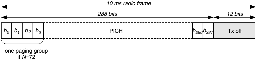
Figure 6.26 PICH structure
