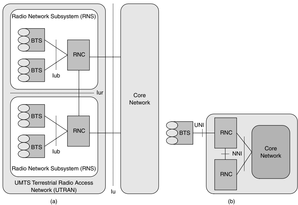
Figure 6.7 UTRAN architecture
