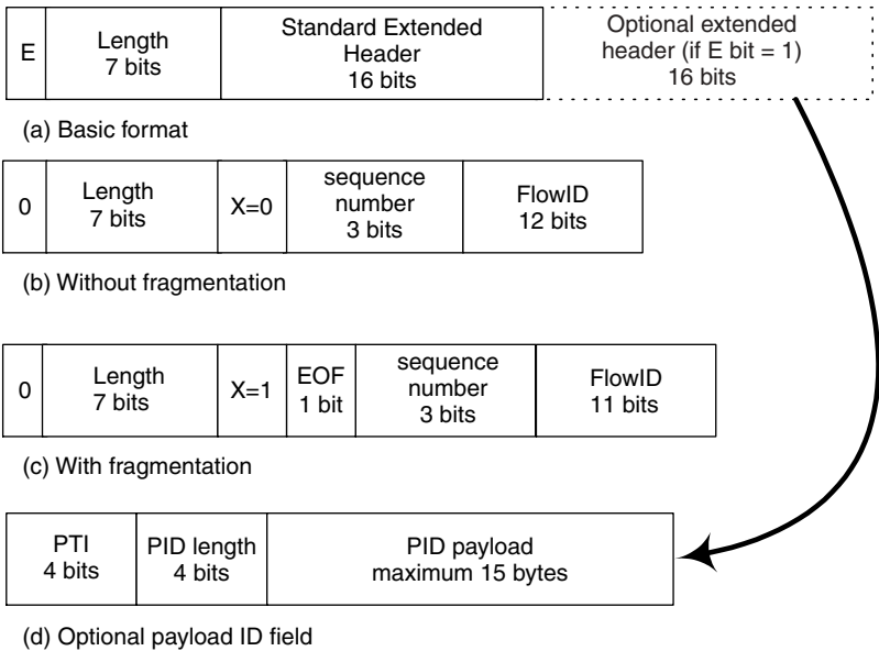
Figure 9.40 LIPE multiplexed header
