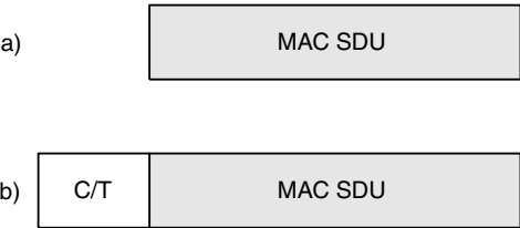
Figure 6.53 MAC format for dedicated transport channels
