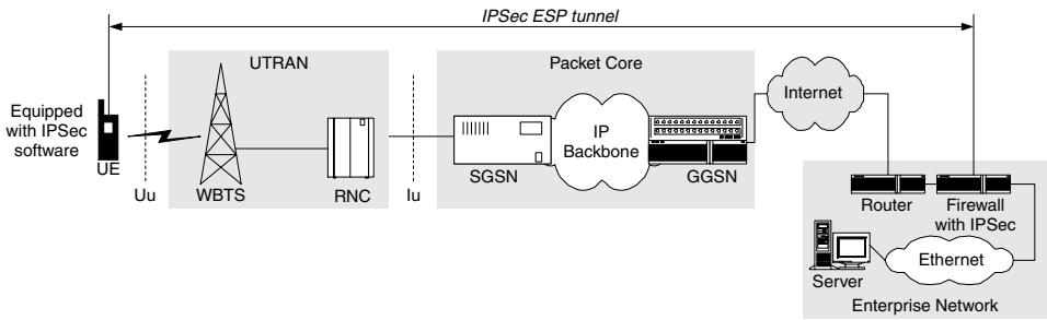
Figure 5.53 GRPS VPN solution
