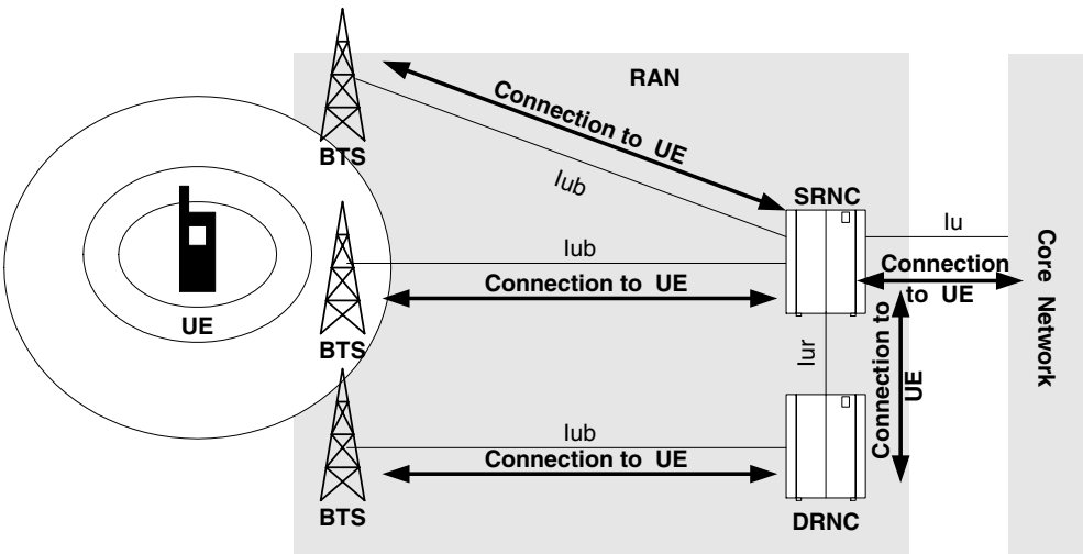
Figure 6.15 Soft handover
