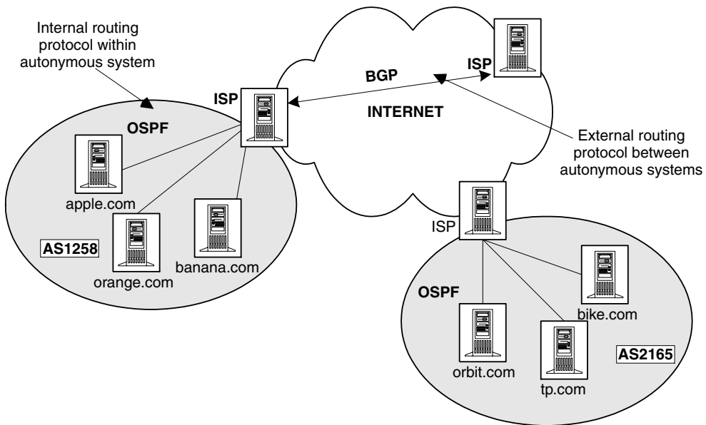
Figure 5.11 Internal and external routing protocols
