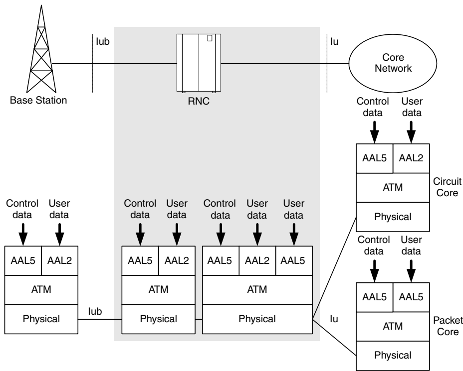
Figure 7.65 Control and user planes in UMTS
