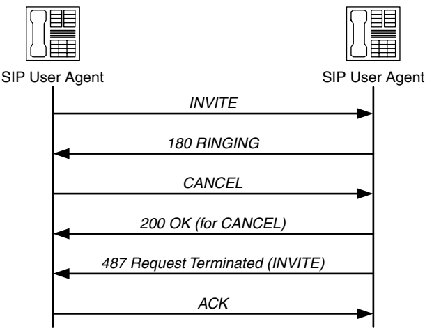
Figure 9.9 CANCEL example
