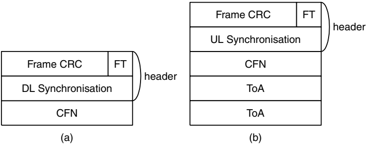
Figure 6.78 Downlink synchronization
