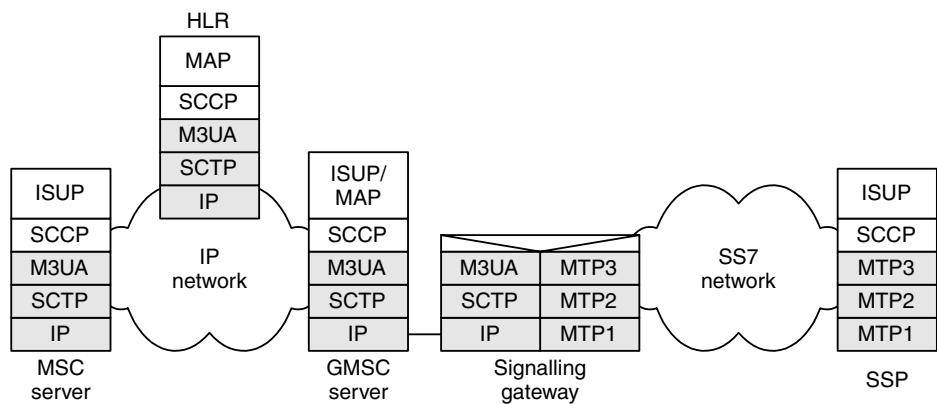
Figure 8.28 M3UA service
