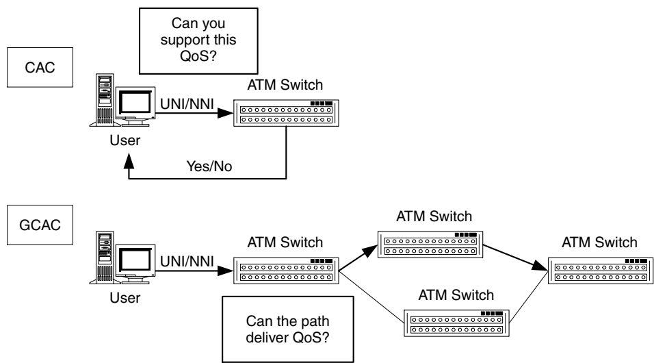
Figure 7.75 GCAC
