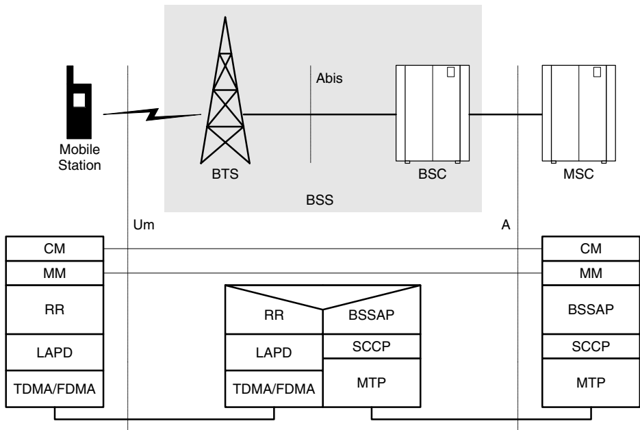
Figure 3.20 GSM protocols
