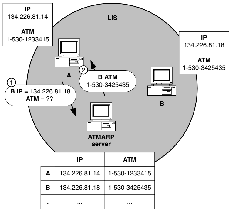
Figure 7.86 Address resolution
