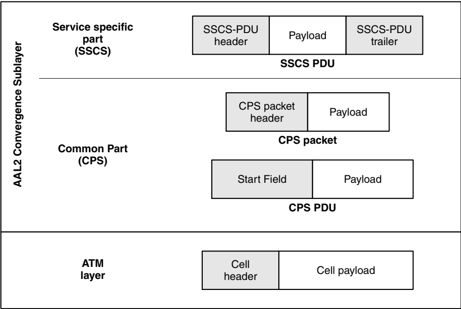
Figure 7.28 AAL2 structure
