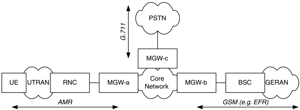
Figure 8.26 UMTS transcoding
