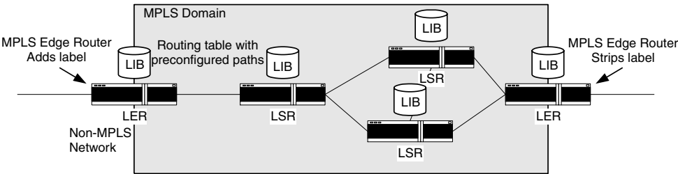
Figure 9.47 MPLS domain
