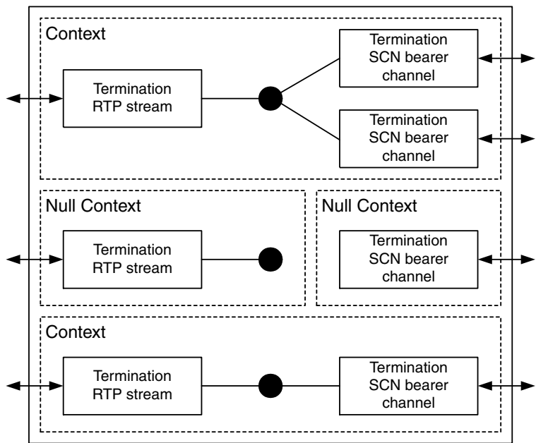
Figure 8.9 MEGACO terminations and contexts
