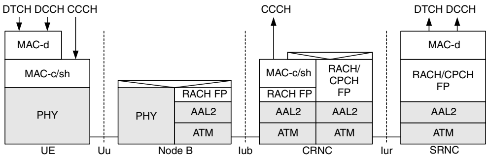
Figure 6.87 RACH protocol stack for separate CRNC and SRNC
