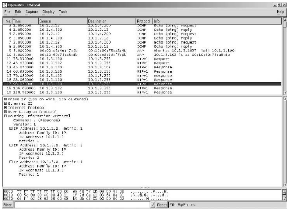
Figure 5.18 RIP router advertisement
