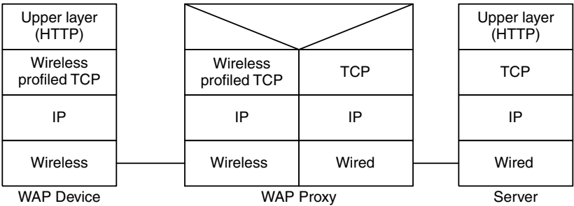
Figure 5.27 Wireless profiled TCP
