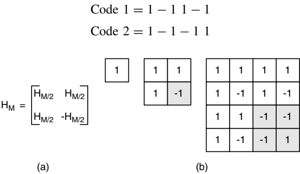
Figure 2.14 Orthogonal code matrix
