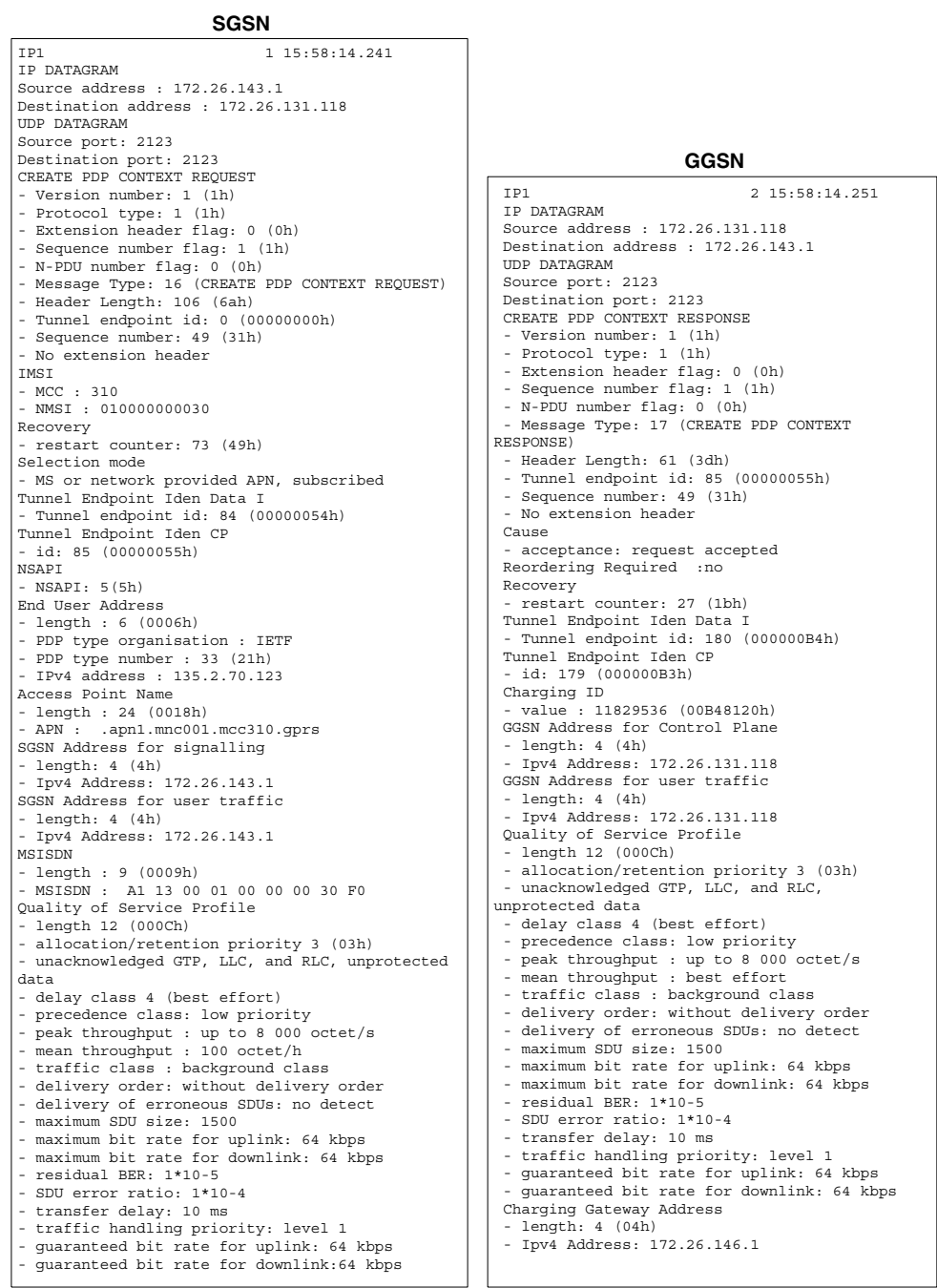
Figure 4.45 Trace PDP context creation. Reproduced by permission of NetHawk Oyj
