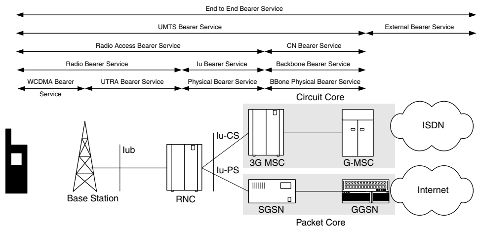
Figure 6.10 End-to-end QoS
