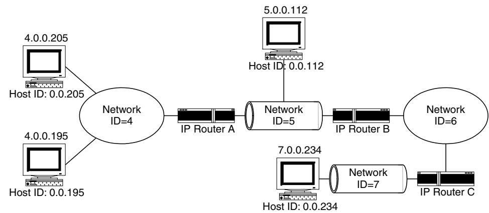
Figure 5.10 IP routing
