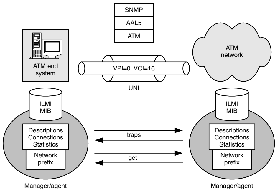
Figure 7.54 ILMI model
