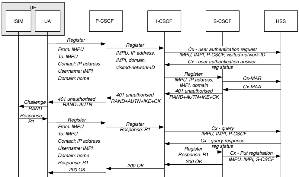
Figure 9.28 IMS registration/authentication
