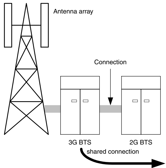
Figure 7.23 2G/3G co-siting
