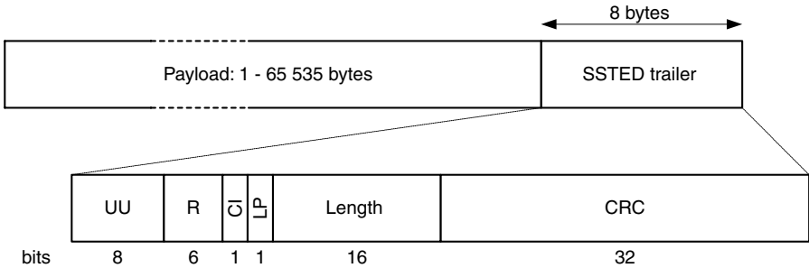
Figure 7.37 SSTED
