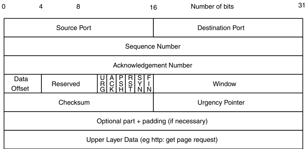
Figure 5.4 TCP header
