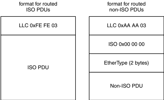
Figure 7.83 Routed protocols
