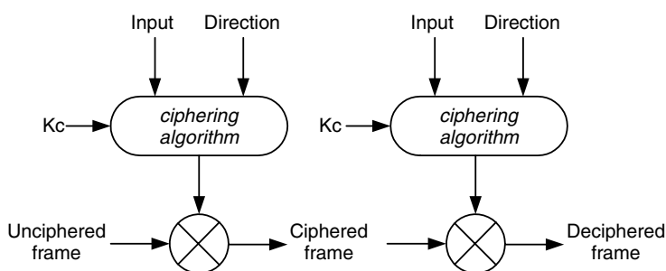
Figure 4.20 Ciphering algorithm
