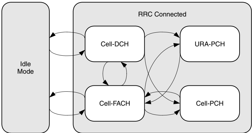
Figure 6.65 RRC Modes
