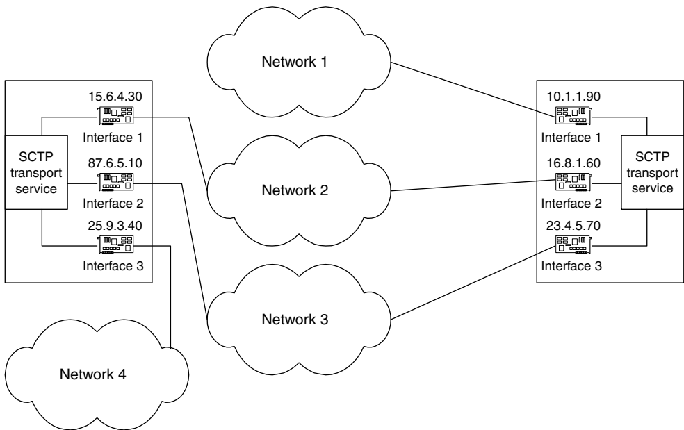
Figure 8.30 Sctp multi-homing
