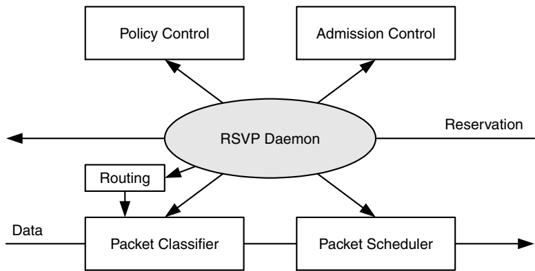
Figure 5.39 Resource reservation
