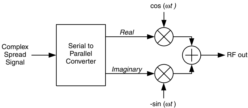
Figure 6.23 QPSK modulation
