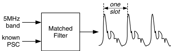
Figure 6.34 Output of matched filter
