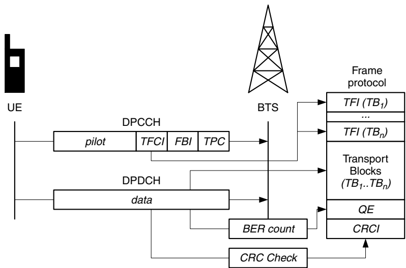
Figure 6.74 Role of uplink frame protocol
