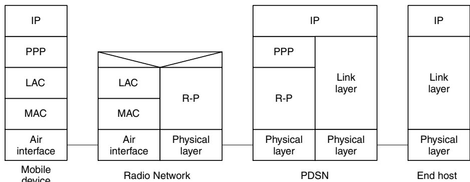
Figure 5.67 PPP for CDMA2000
