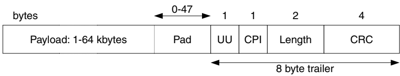
Figure 7.41 AAL5 PDU format
