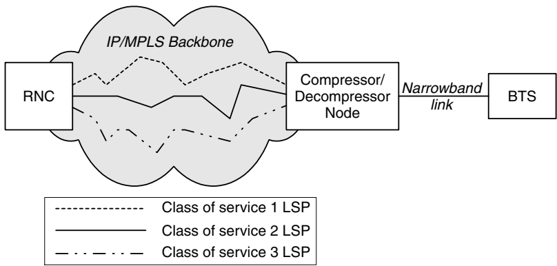
Figure 9.46 MPLS in the RAN
