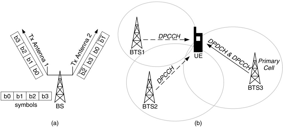
Figure 6.39 (a) STTD and (b) SSdT
