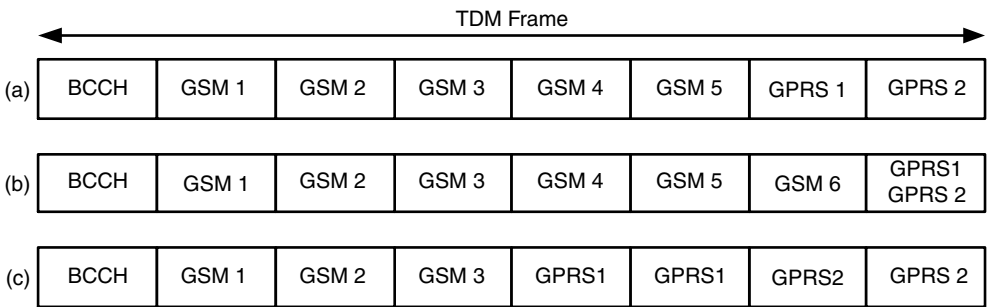
Figure 4.5 TDM frames
