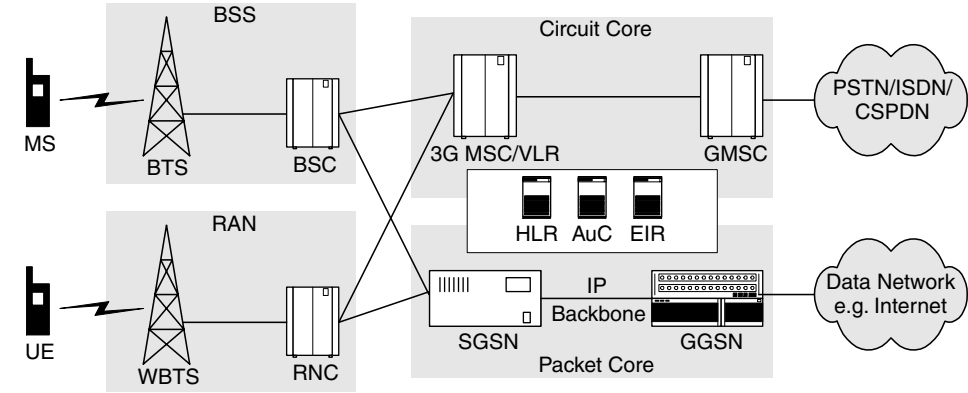
Figure 6.2 UMTS release 99 network
