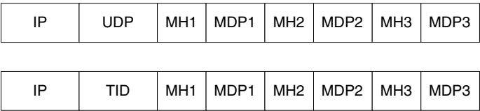
Figure 9.39 LIPE encapsulation format
