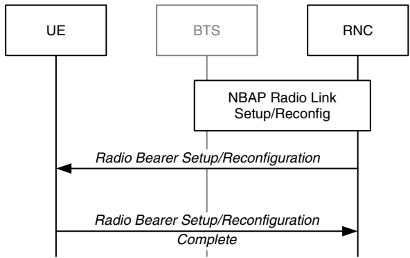
Figure 6.68 Radio bearer setup or reconfiguration
