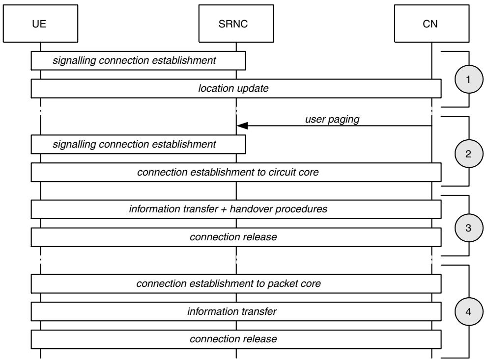
Figure 6.127 Basic UMTS call life cycle
