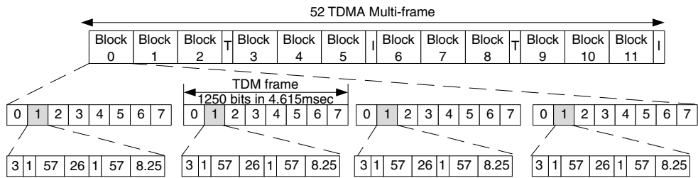
Figure 4.4 52-frame format
