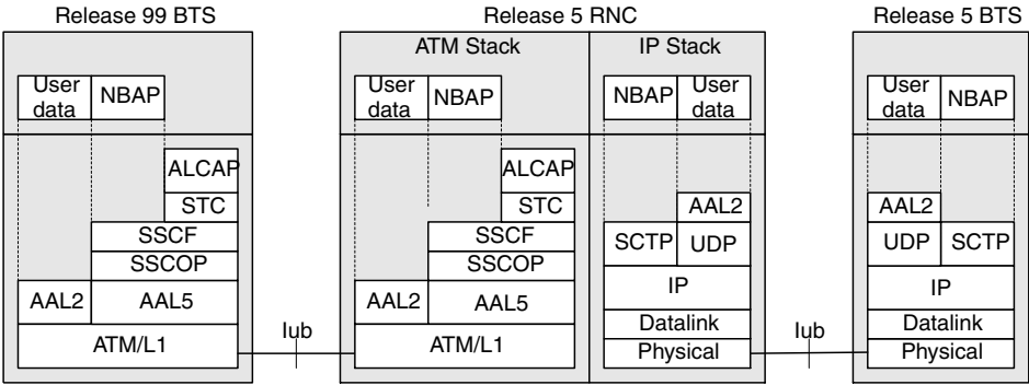
Figure 9.43 RNC dual stack IP/ATM (Iub)
