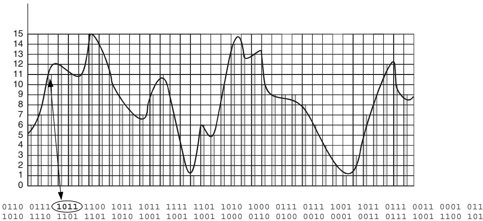
Figure 2.6 Pulse code modulation
