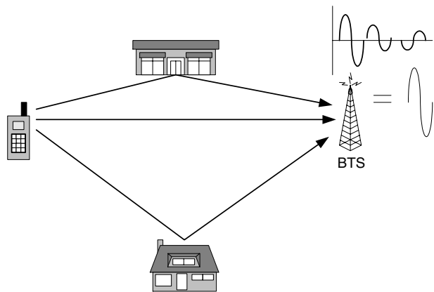
Figure 2.21 Multipath propagation
