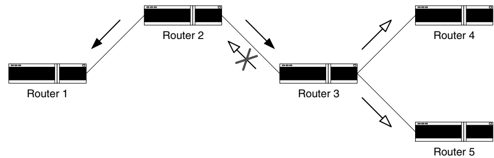
Figure 5.16 Example of split horizon
