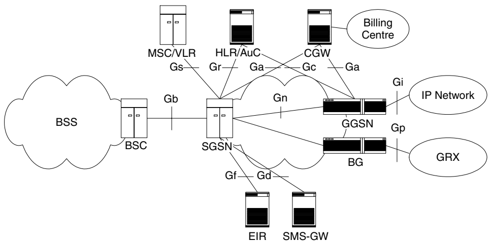
Figure 4.3 GPRS interfaces
