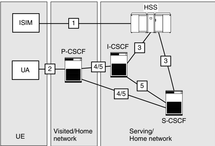
Figure 9.26 IMS security architecture
