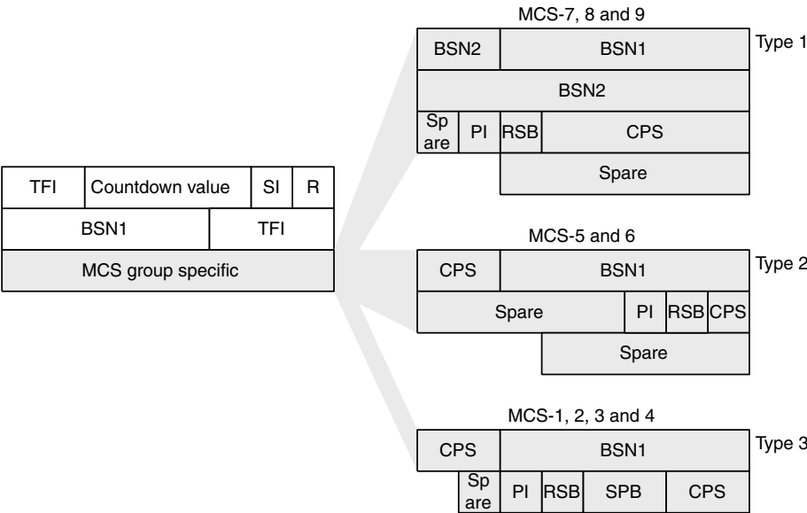
Figure 4.56 EDGE uplink RLC/MAC headers
