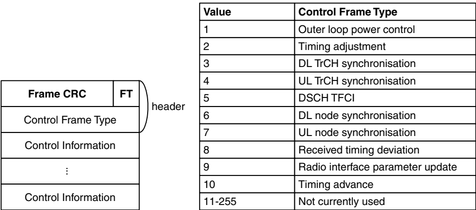
Figure 6.75 Control frame general format
