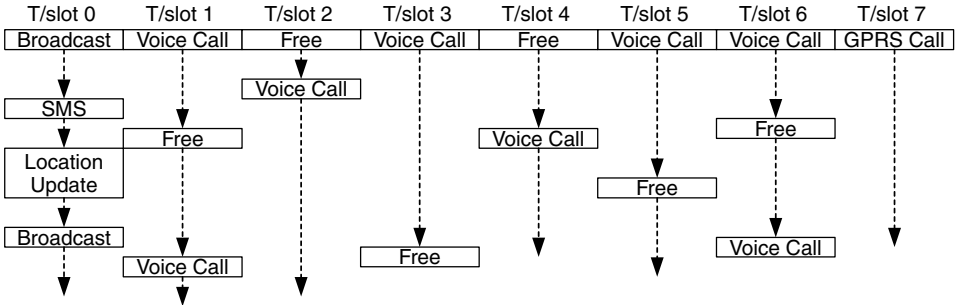
Figure 3.10 Example use of time slots
