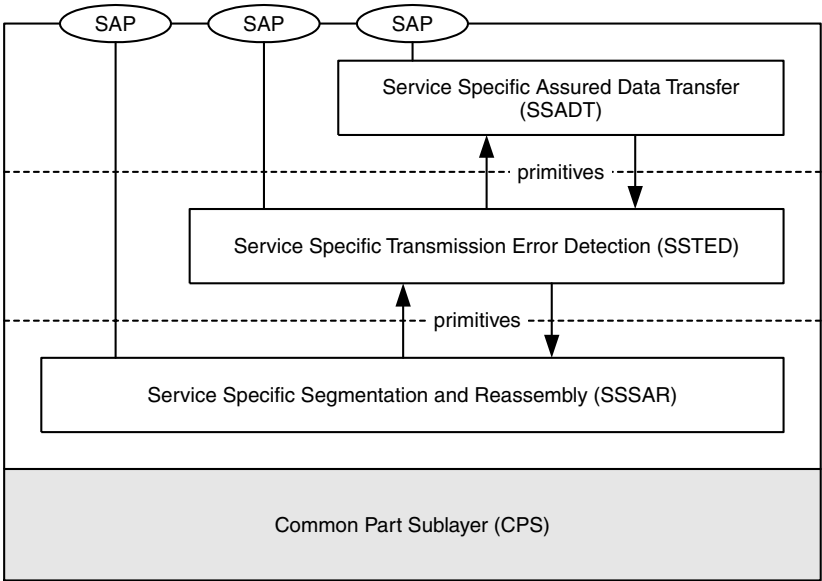
Figure 7.35 SAR service-specific convergence sublayer
