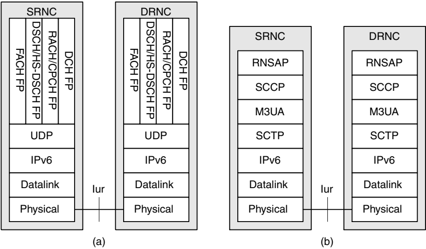
Figure 9.35 Iur IP transport option: user and control planes
