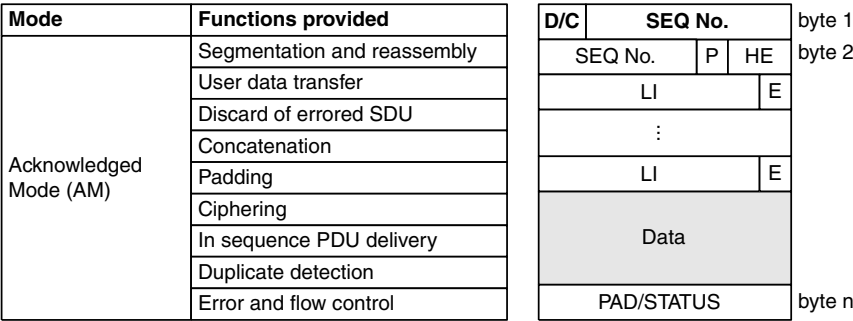
Figure 6.48 RLC acknowledged mode PDU
