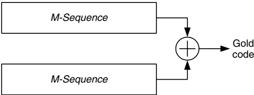
Figure 2.20 Gold code generator
