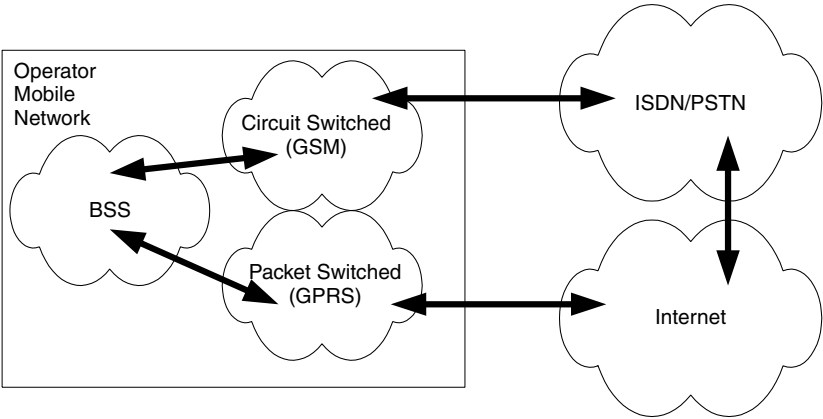
Figure 4.1 Network infrastructure
