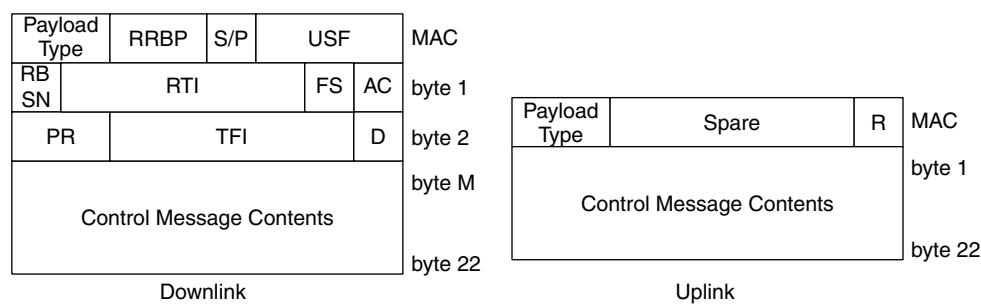
Figure 4.25 RLC/MAC control block
