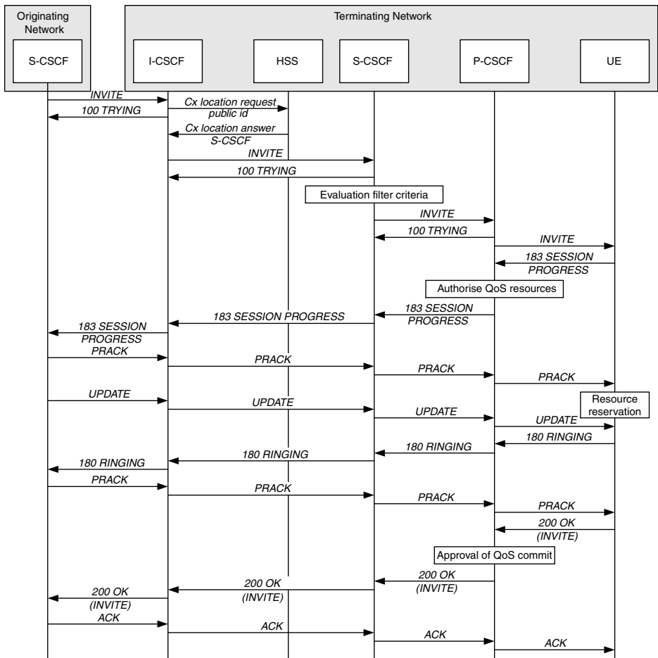
Figure 9.30 Mobile terminated call
