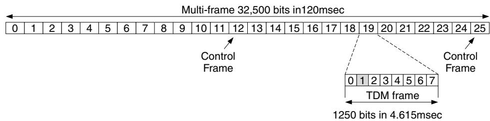
Figure 3.13 GSM multiframe
