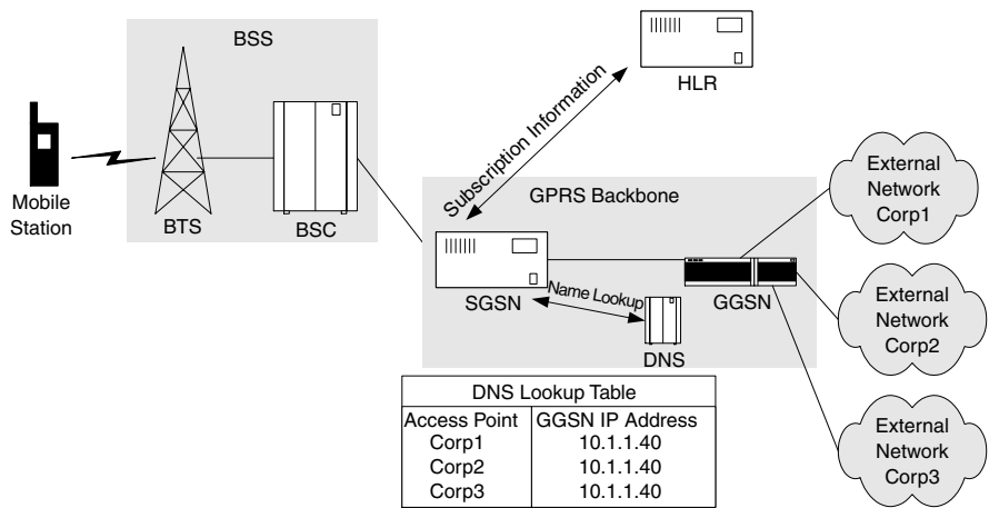
Figure 4.40 PDP context activation
