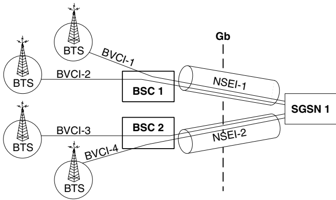
Figure 4.28 Example use of BVC and NSEI identifiers
