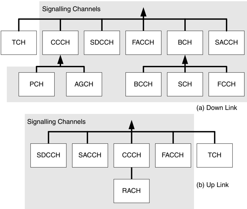
Figure 3.15 GSM logical channels
