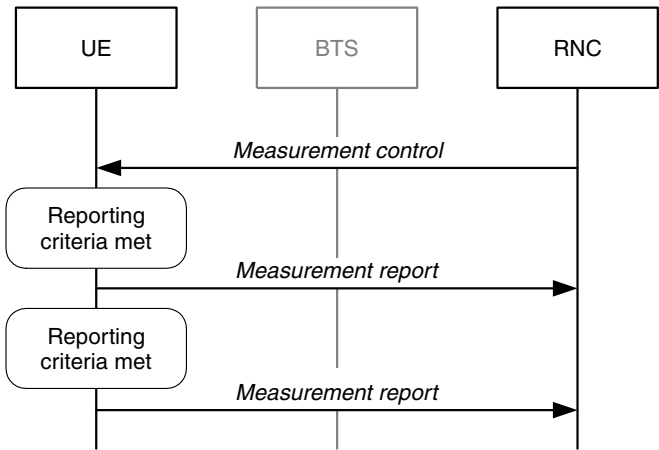
Figure 6.70 RRC measurement reporting
