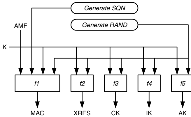
Figure 6.120 Authentication vector generation
