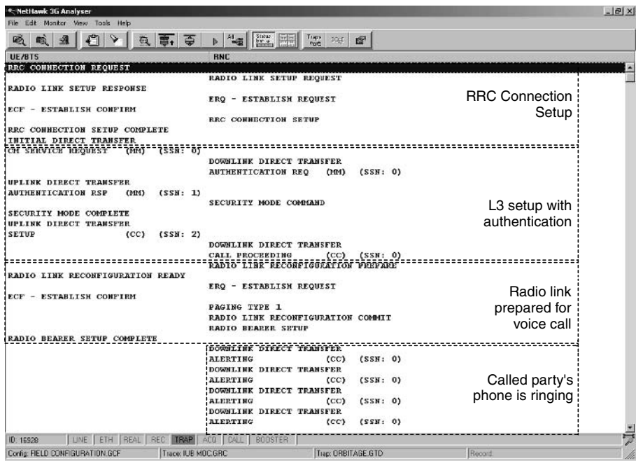
Figure 6.135 Sample Iub trace of part of a mobile originated call. Reproduced by permission of NetHawk Oyj
