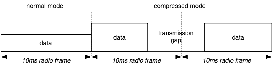
Figure 6.37 Compressed mode
