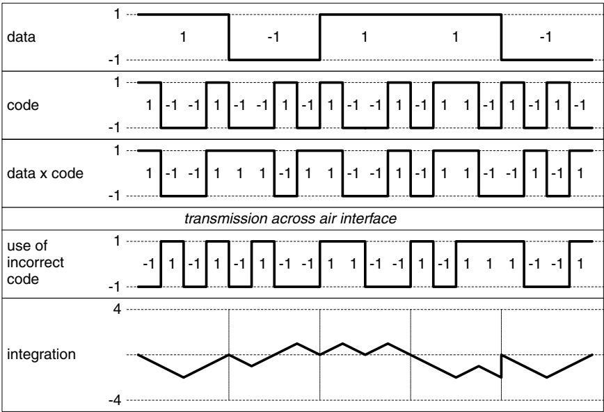
Figure 2.13 Correlation with incorrect code
