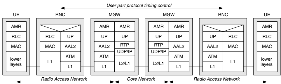
Figure 8.3 User plane for UMTS Release 4
