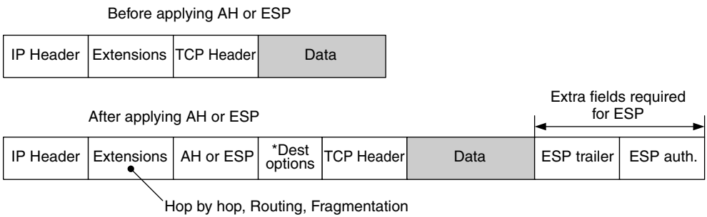
Figure 5.49 Inclusion of IPSec header (IPv6)
