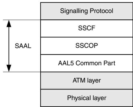
Figure 7.57 ATM signalling protocol stack
