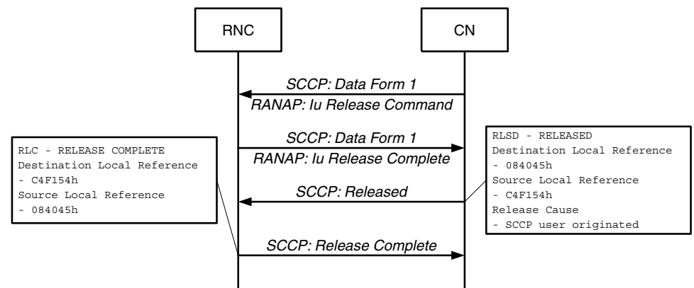
Figure 6.117 SCCP connection release. Reproduced by permission of NetHawk Oyj
