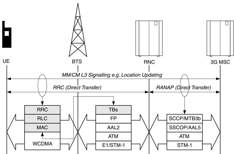
Figure 6.106 Signalling protocol stack
