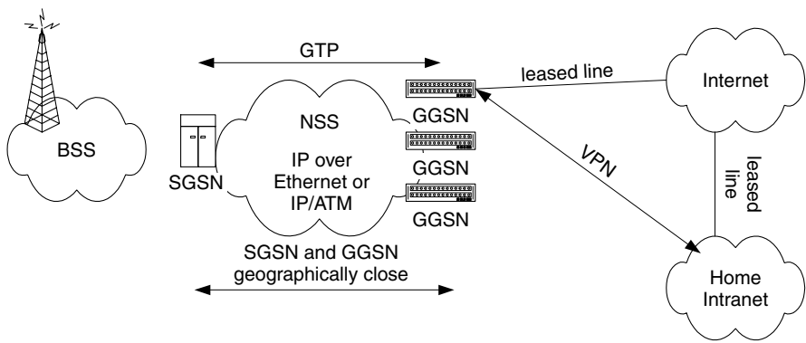
Figure 4.51 Connection using a leased line or VPN
