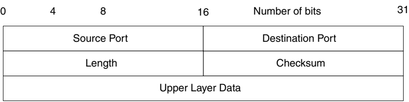
Figure 5.7 UDP header
