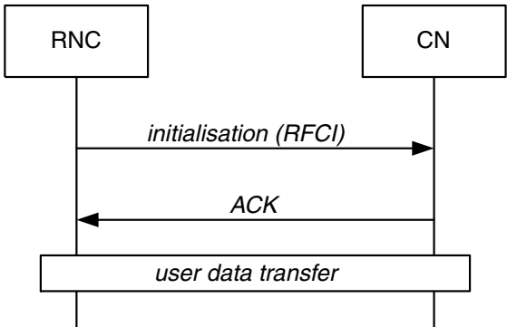
Figure 6.95 Initialization procedure
