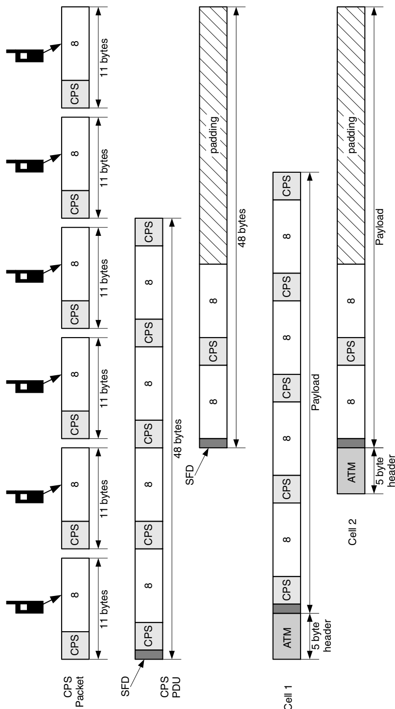
Figure 7.33 AAL2 overheads
