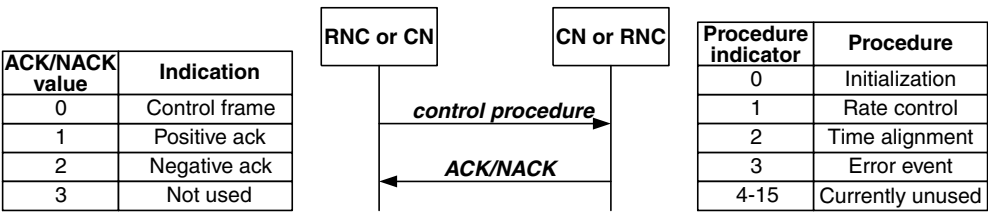
Figure 6.93 Acknowledge procedure
