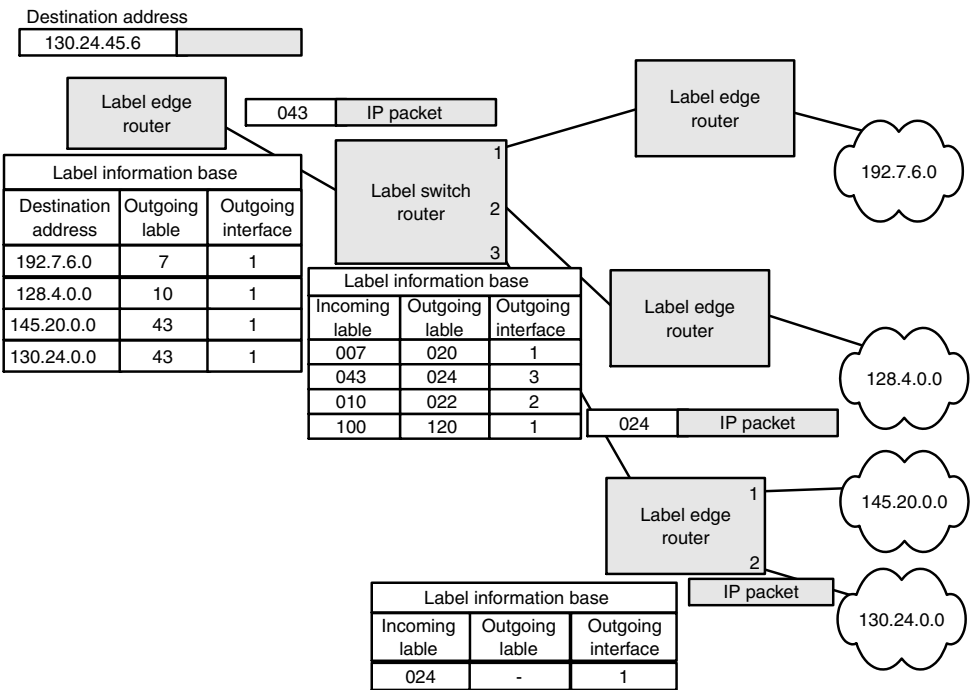
Figure 9.48 MPLS forwarding
