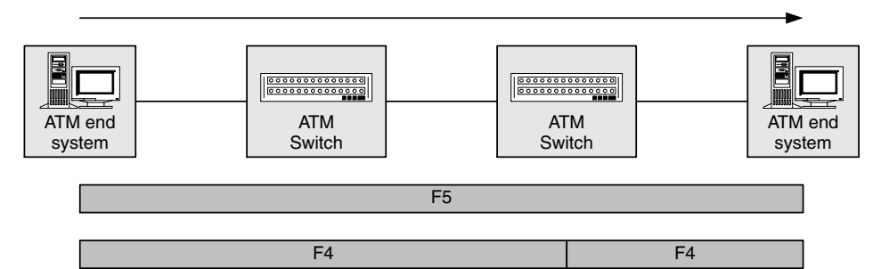
Figure 7.55 OAM flows
