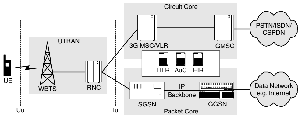
Figure 5.29 UMTS release 99
