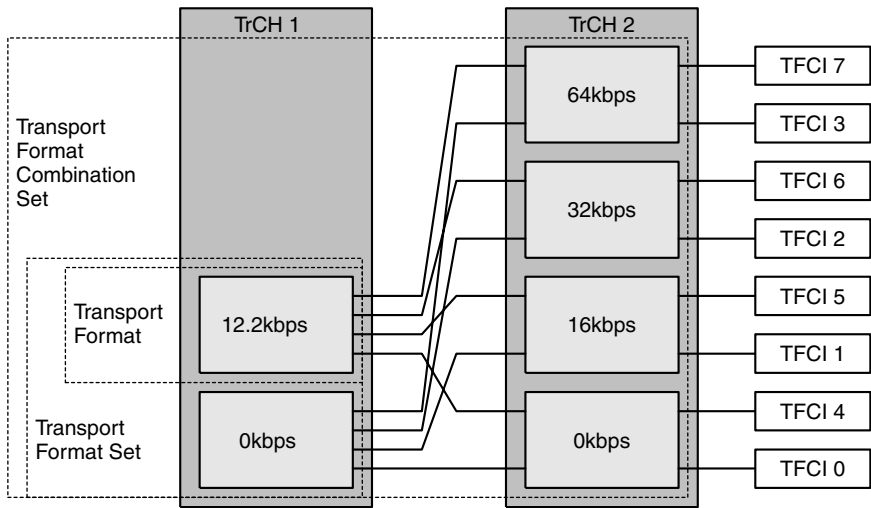
Figure 6.60 TFCS example
