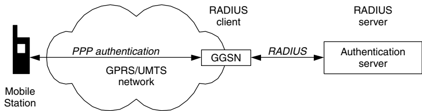
Figure 5.68 RADIUS configuration
