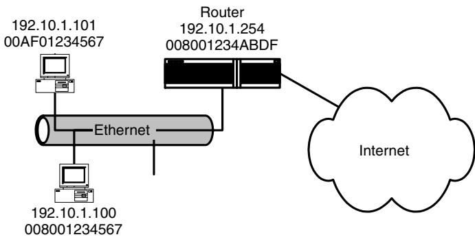
Figure 5.9 ARP example
