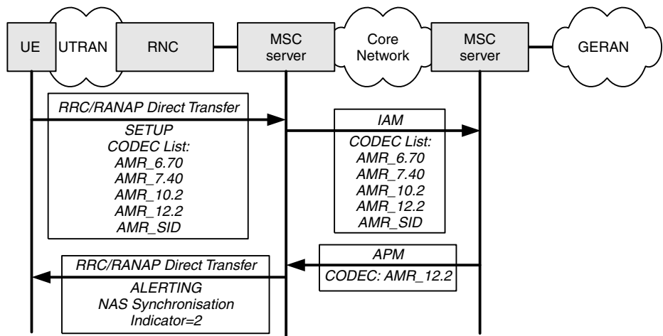
Figure 8.27 CODEC negotiation
