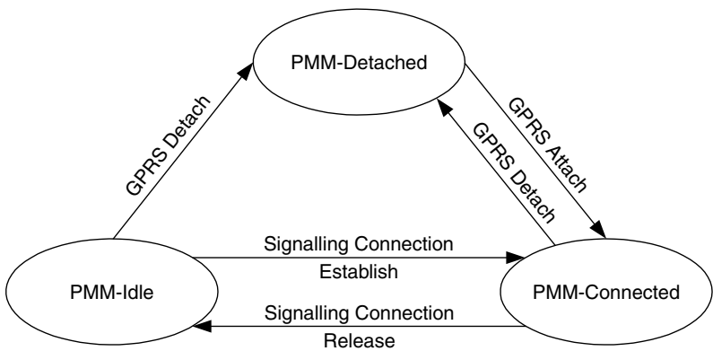
Figure 6.118 Mobility management
