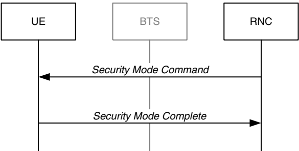
Figure 6.67 Security procedure
