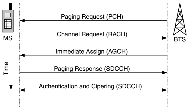
Figure 3.18 Initial access
