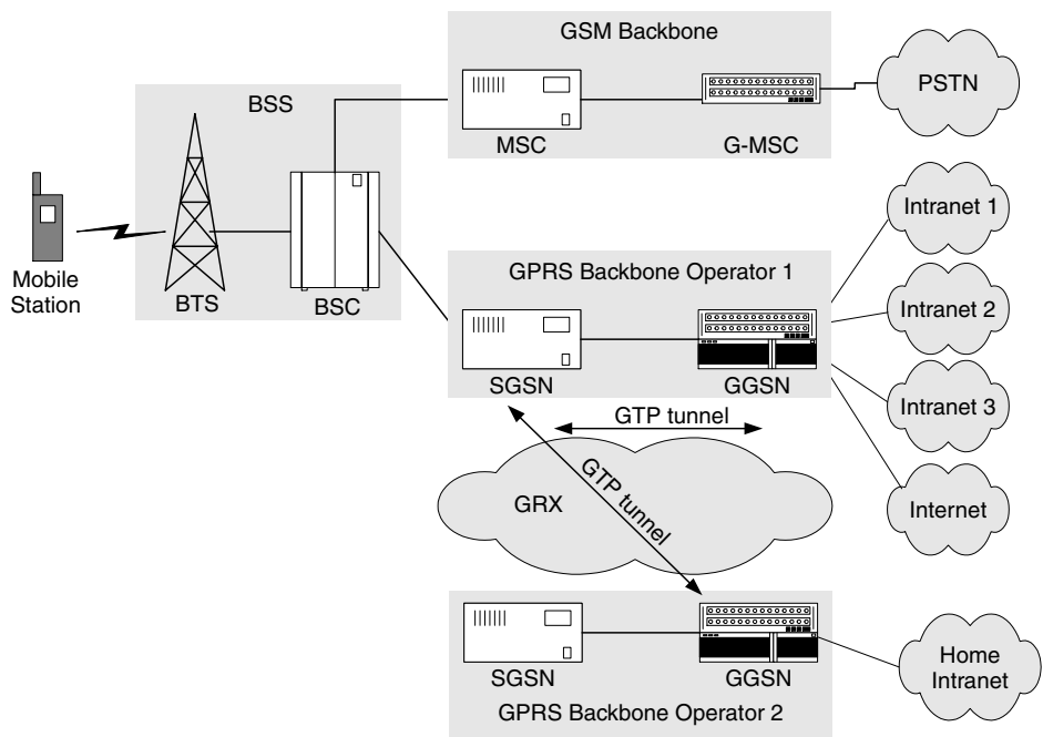
Figure 4.41 GTP tunnel
