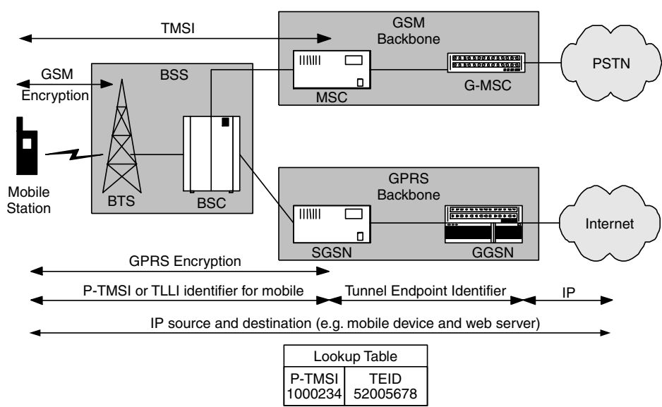
Figure 4.32 GPRS network identifiers
