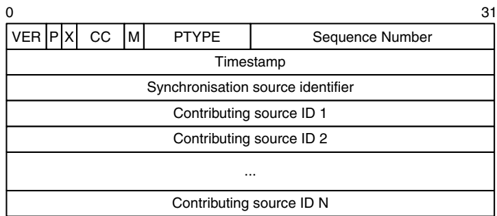
Figure 8.4 RTP header
