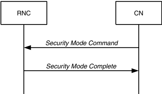
Figure 6.114 Security procedure
