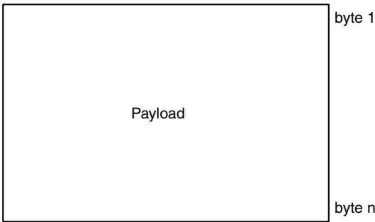
Figure 6.90 Transparent mode
