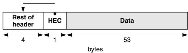
Figure 7.13 Header checking
