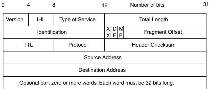
Figure 5.2 IP header
