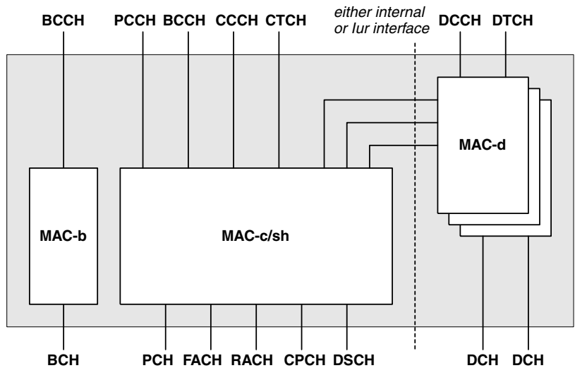
Figure 6.51 MAC architecture
