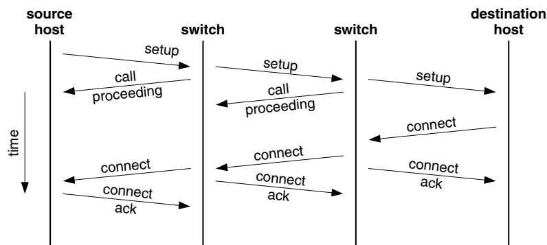
Figure 7.67 Connection setup
