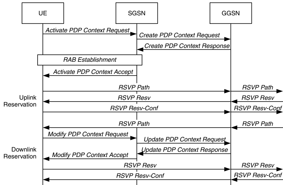
Figure 5.42 End-to-end reservation
