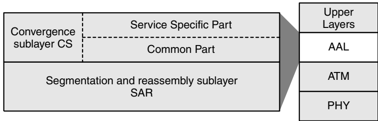
Figure 7.19 AAL sublayers
