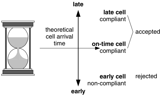
Figure 7.50 Virtual scheduling
