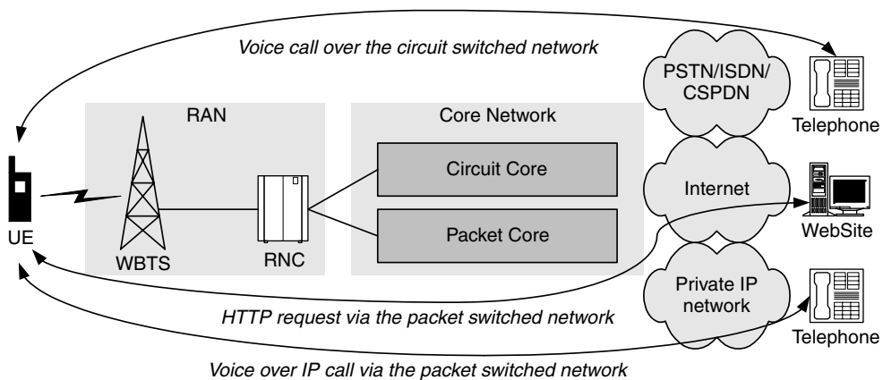
Figure 6.9 QoS considerations
