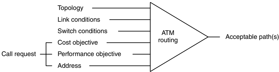
Figure 7.74 ATM routing
