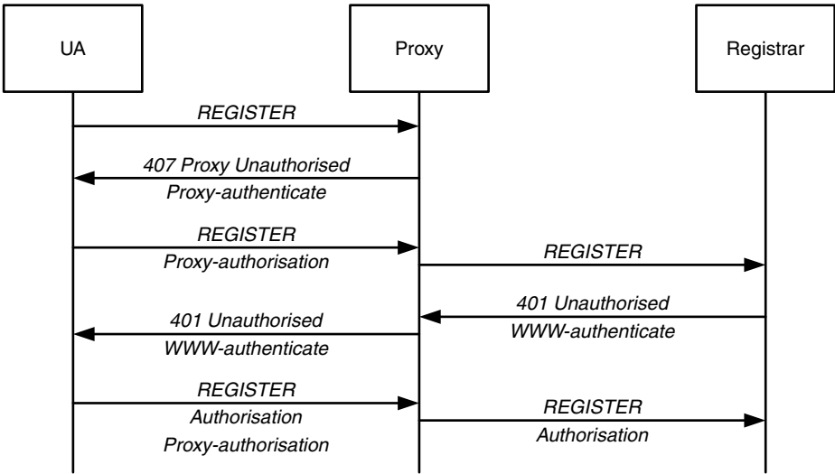
Figure 9.22 Authenticated registration
