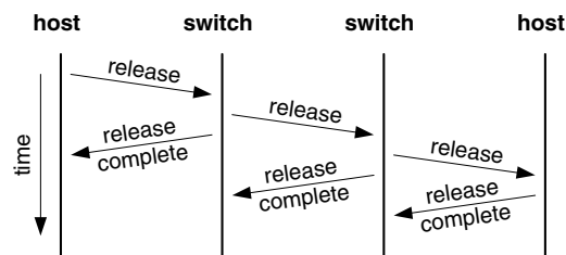
Figure 7.68 Connection release
