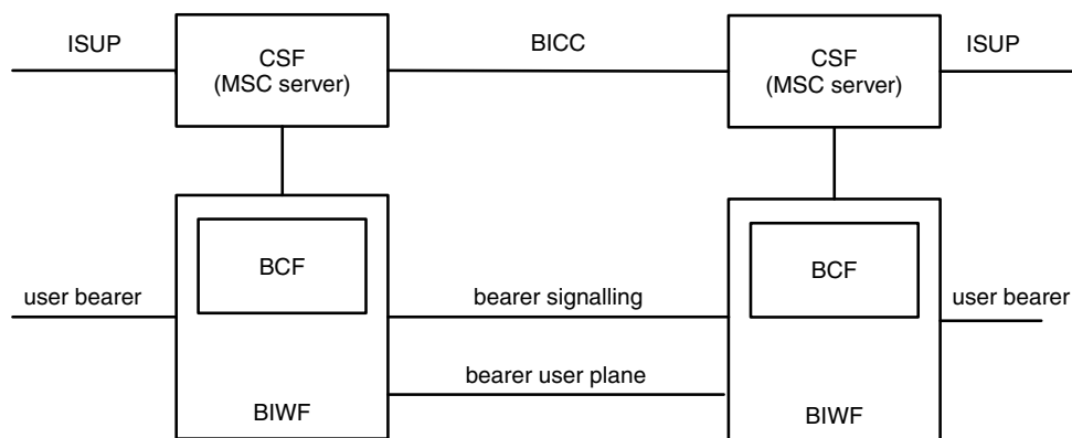
Figure 8.17 BICC architecture
