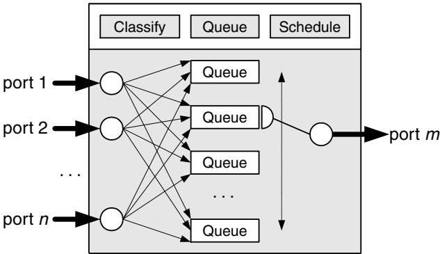
Figure 7.45 CQS architecture
