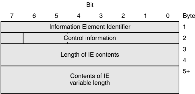
Figure 7.72 IE format
