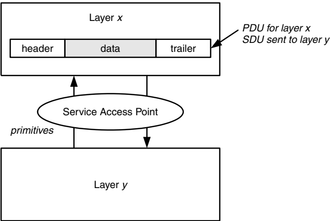
Figure 7.5 Layered model
