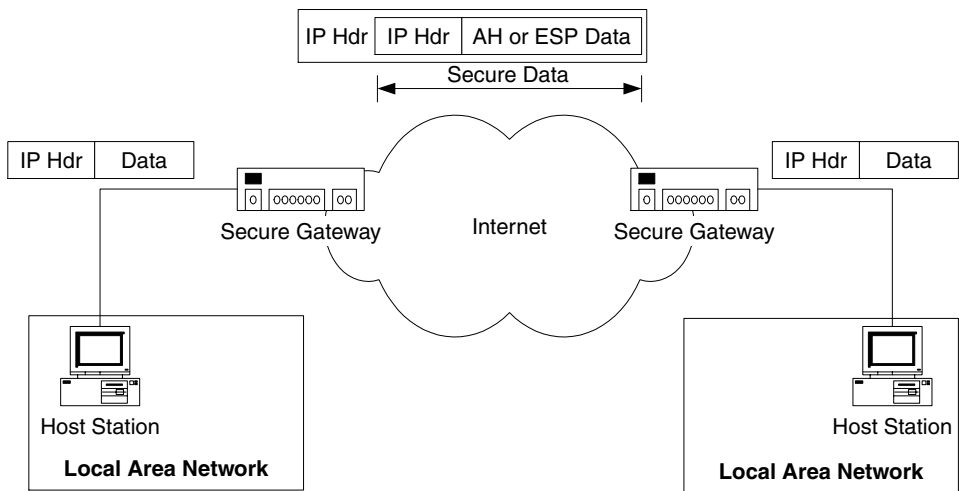
Figure 5.50 Tunnel mode
