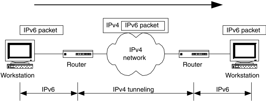
Figure 5.59 IPv6 tunnelling
