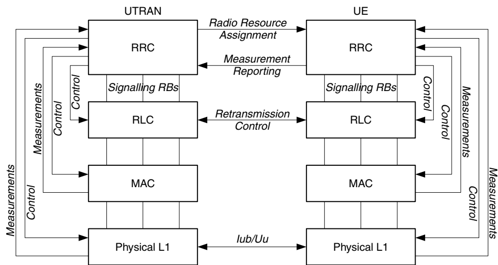
Figure 6.64 RRC control
