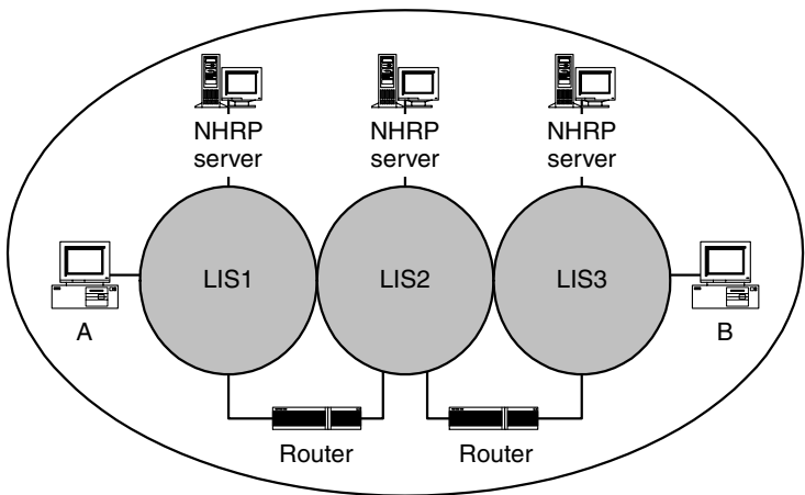
Figure 7.87 NHRP
