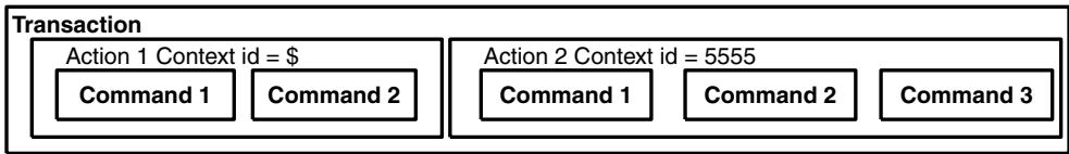
Figure 8.11 MEGACO transaction
