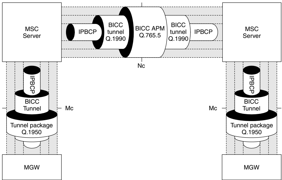
Figure 8.21 IPBCP tunnelling
