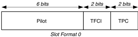
Figure 6.28 DPCCH slot format 0
