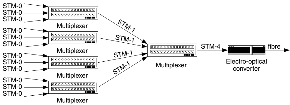
Figure 7.9 SDH signals
