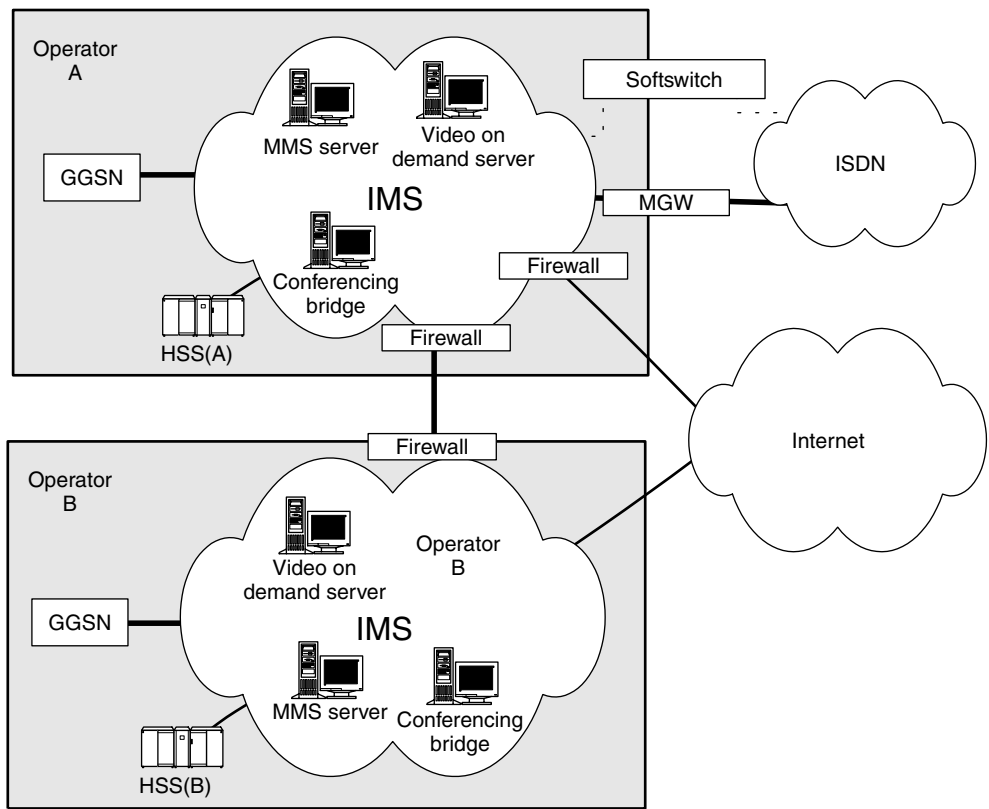
Figure 9.3 IMS connection
