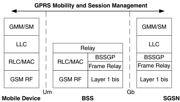
Figure 4.7 Control plane for GPRS/GSM
