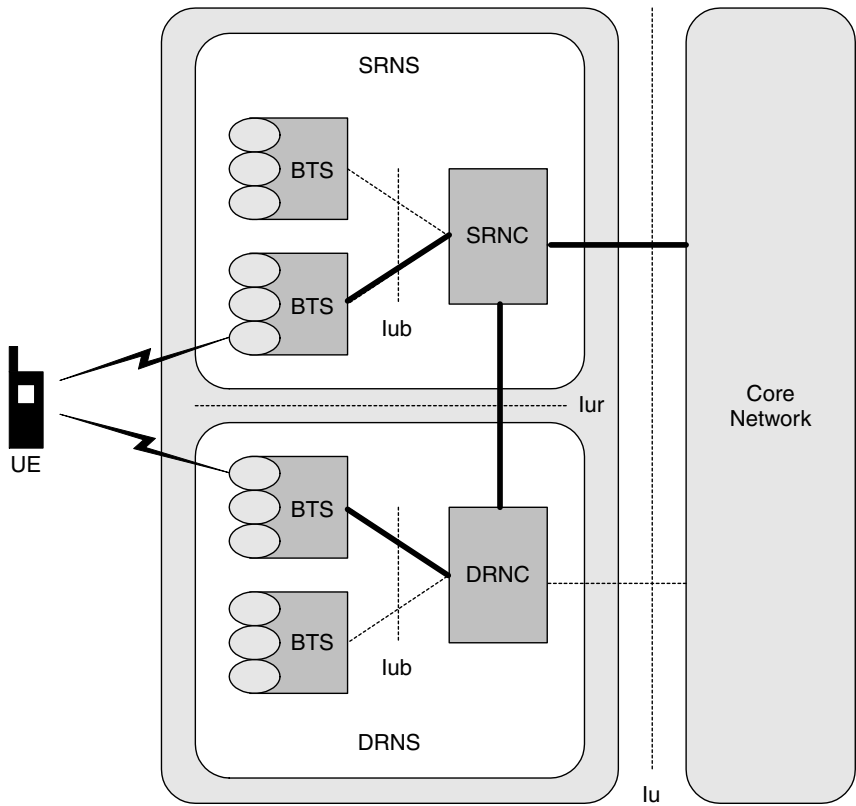
Figure 6.8 Serving and drift RNC for soft handover
