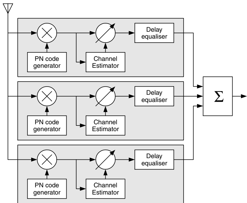
Figure 2.23 Rake receiver
