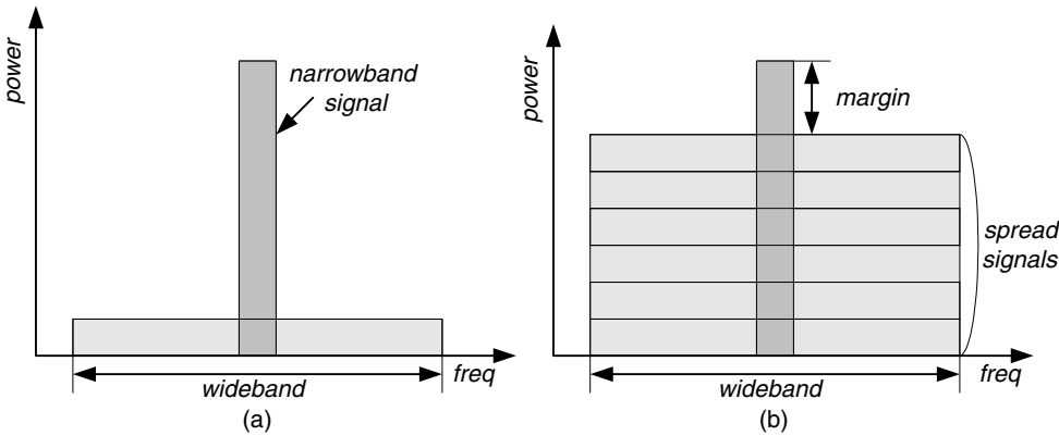
Figure 2.10 Signal spreading
