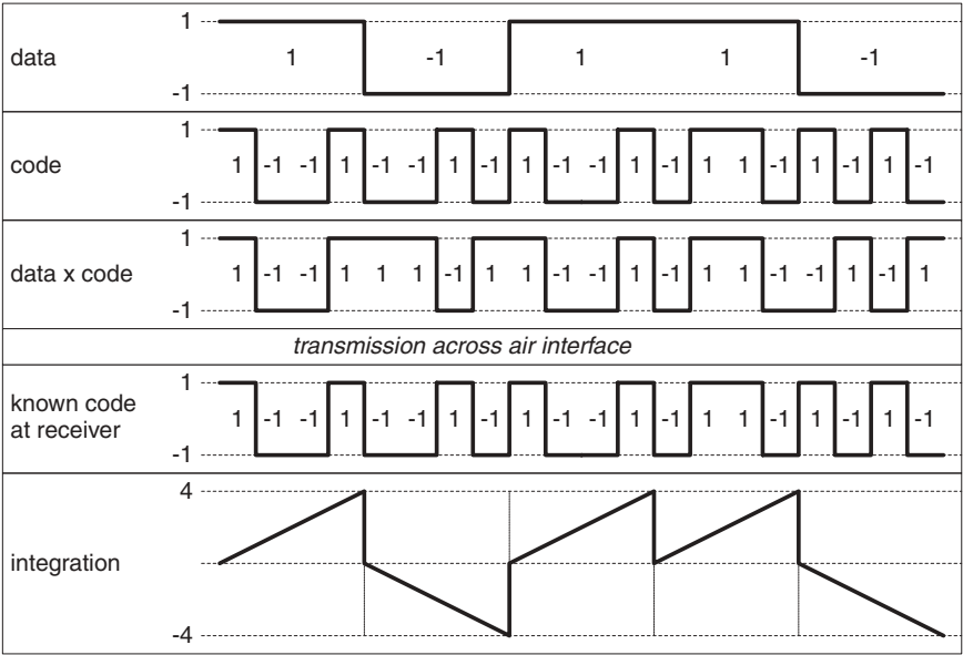
Figure 2.12 Correlation at a CDMA receiver
