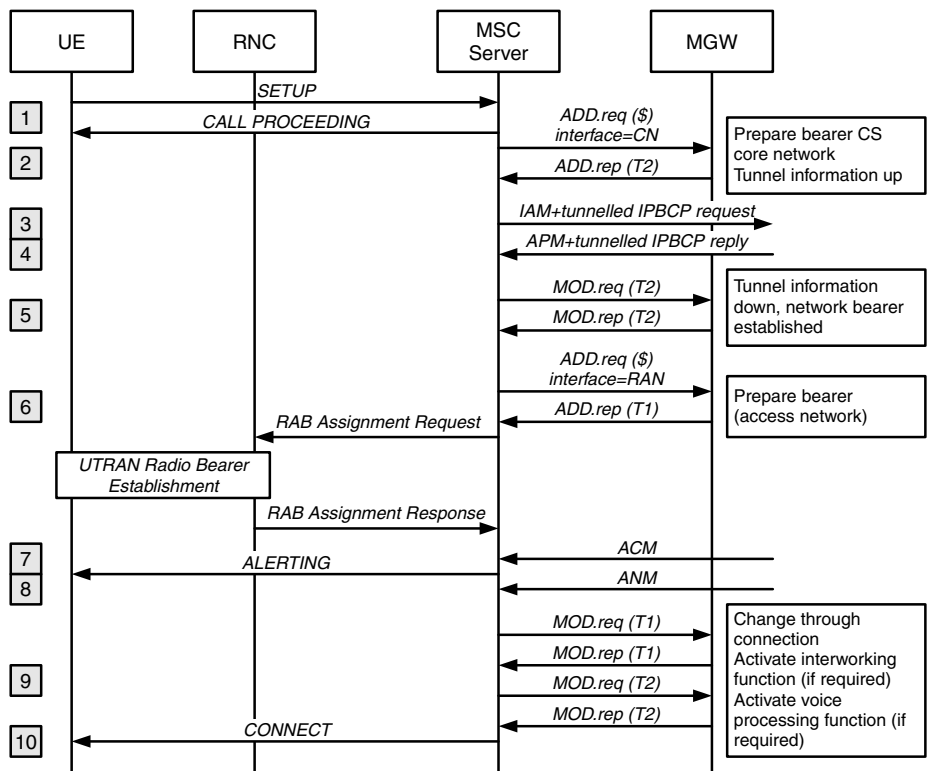
Figure 8.22 BICC Release 4 call flow example (forward bearer establishment)
