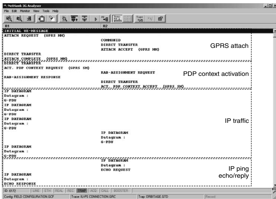
Figure 6.139 Sample lu-PS trace packet connection establishment. Reproduced by permission of NetHawk Oyj
