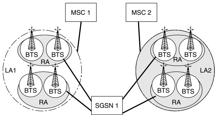
Figure 4.34 GPRS routing area
