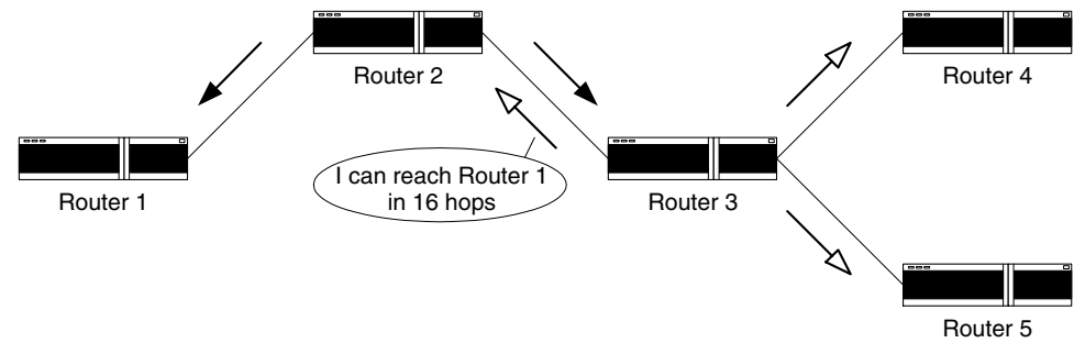
Figure 5.17 Example of poison reverse
