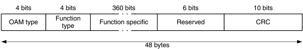
Figure 7.56 OAM cell structure
