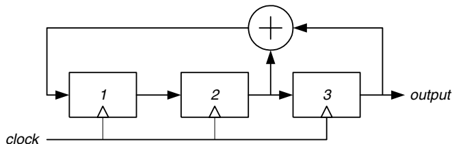
Figure 2.18 Three-stage shift register
