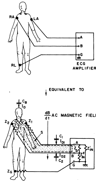
Fig. 1. Typical ECG recording configuration lead I and the equivalent circuit. RA is right arm; LA is left arm. RL is right leg. The capacitors simulate the entry of displacement currents. Dotted lines indicate the area S of the conductive loop.
