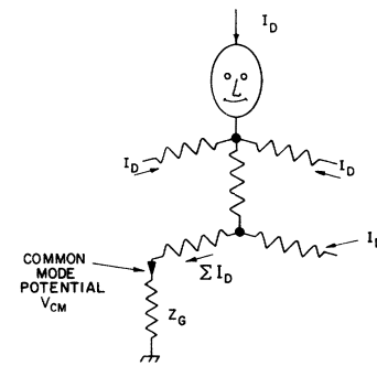
Fig. 6. Model illustrating the body's internal resistance and displacement currents flowing to ground with only the ground electrode attached.
