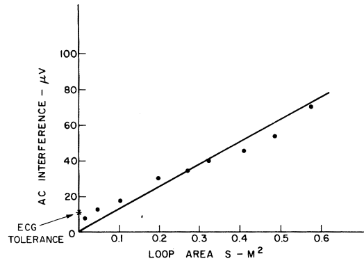
Fig. 2. AC potential at the amplifier input versus loop area for magnetic induction interference.
