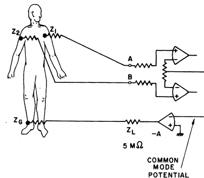
Fig. 10. Driven right-leg configuration.
