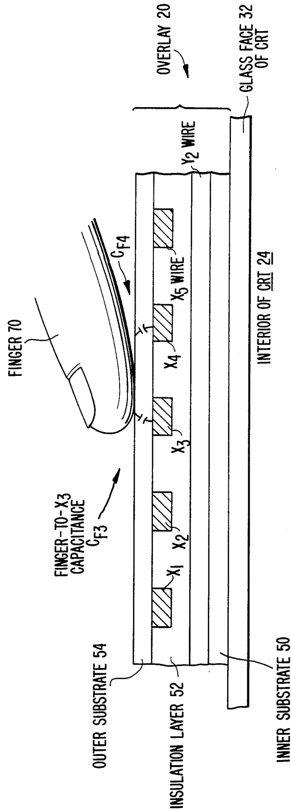
FIG. 8. FINGER TOUCH DETECTION
