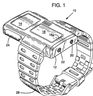
Figure 1 is an isometric view of a wrist-worn ECG monitor 10. Ex. 1006, 2:39–41.
