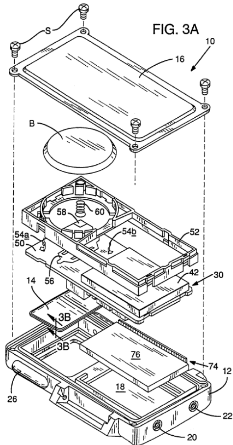
Figure 2 is a frontal isometric view of the ECG monitor 10 (with the wrist band removed), and Figure 3A is an exploded isometric view of the ECG monitor (shown from the rear instead of the front). Ex. 1006, 2:42–47.
