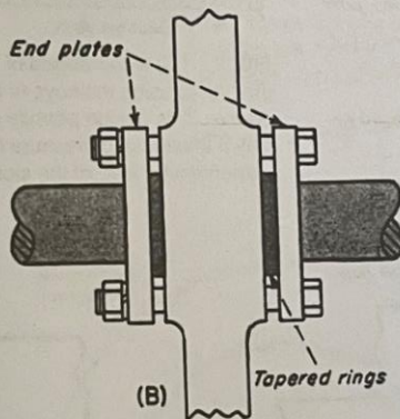
Fig. 7 Interlocking tapered rings hold the hub tightly to the shaft when the nut is tightened. Coarse machining of the hub and shaft does not affect concentricity as in pinned and keyed assemblies. A shoulder is required (A) for end-of-shaft mounting. End plates and four bolts (B) allow the hub to be mounted anywhere on the shaft.
