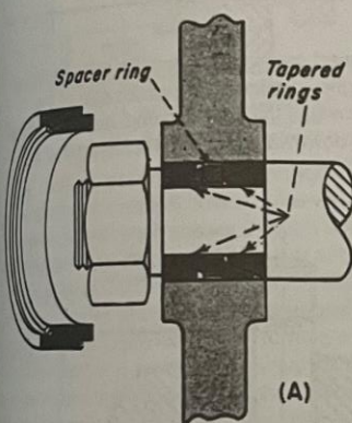
Fig. 7 Interlocking tapered rings hold the hub tightly to the shaft when the nut is tightened. Coarse machining of the hub and shaft does not affect concentricity as in pinned and keyed assemblies. A shoulder is required (A) for end-of-shaft mounting. End plates and four bolts (B) allow the hub to be mounted anywhere on the shaft.
