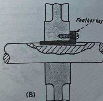
Fig. 3 A feather key (A) allows axial gear movement. A keyway must be milled to the end of the shaft. For a blind keyway (B) the hub and key must be drilled and tapped, but the design allows the gear to be mounted anywhere on the shaft with only a short keyway.
